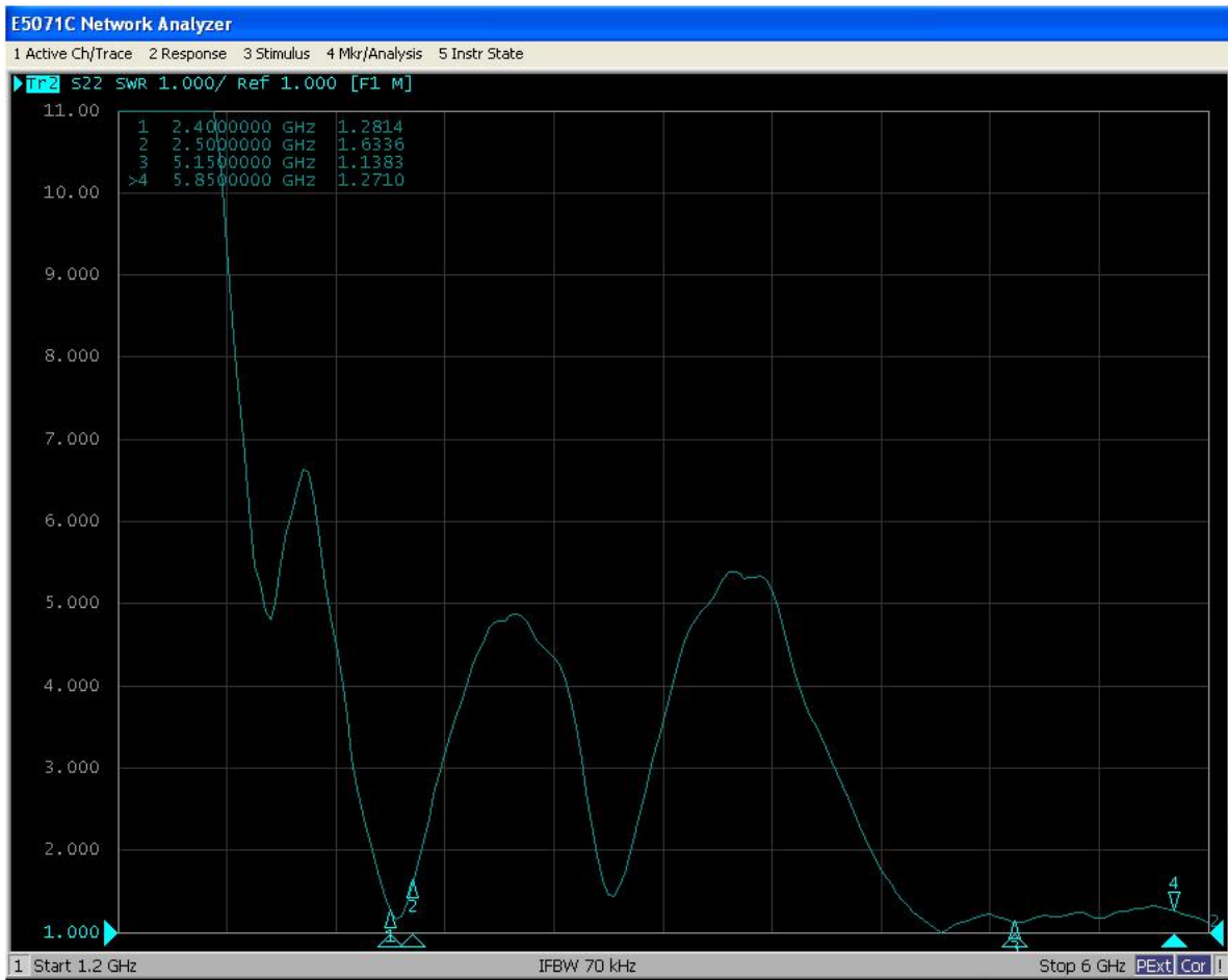
2.4+5.8G WIFI antenna VSWR
