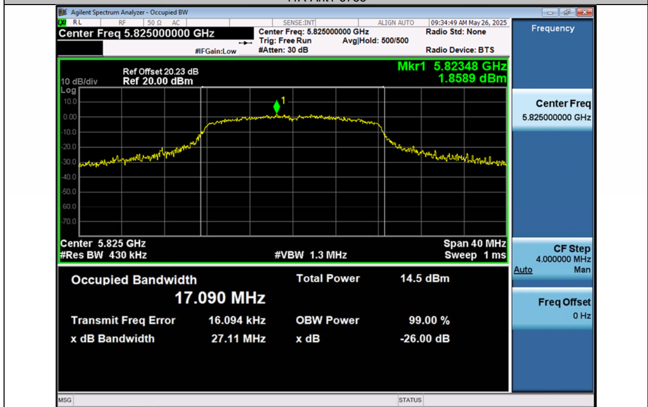
11A-Ant1-5825
