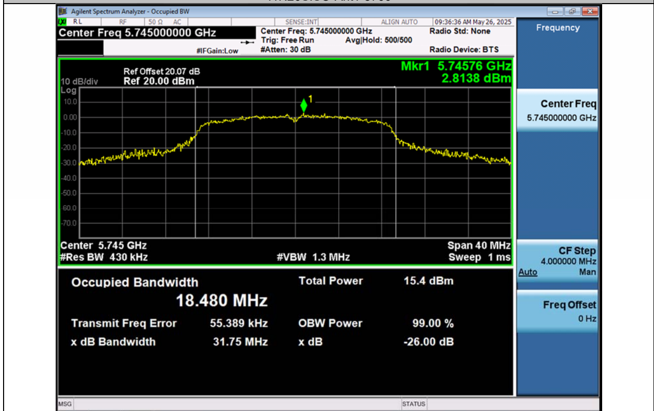
11N20SISO-Ant1-5745
