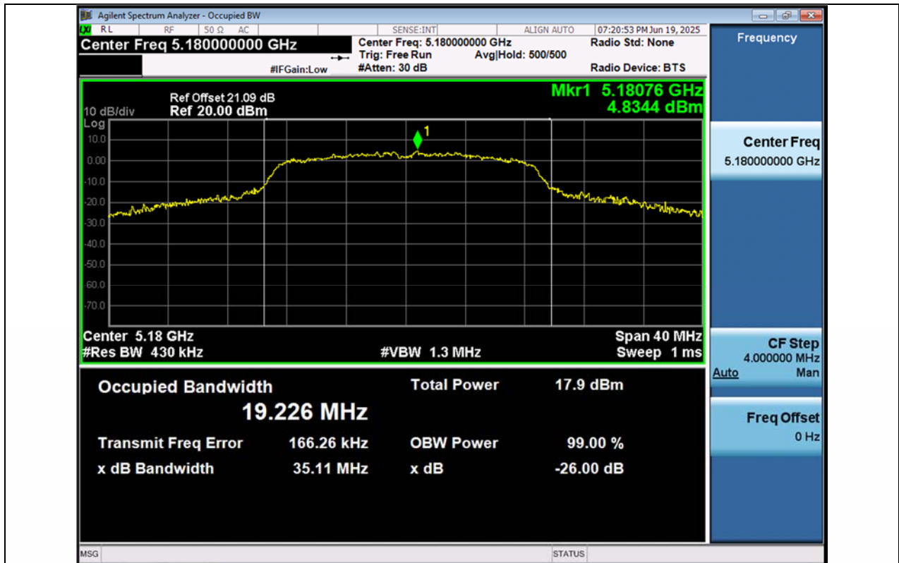
11N20SISO-Ant1-5180
