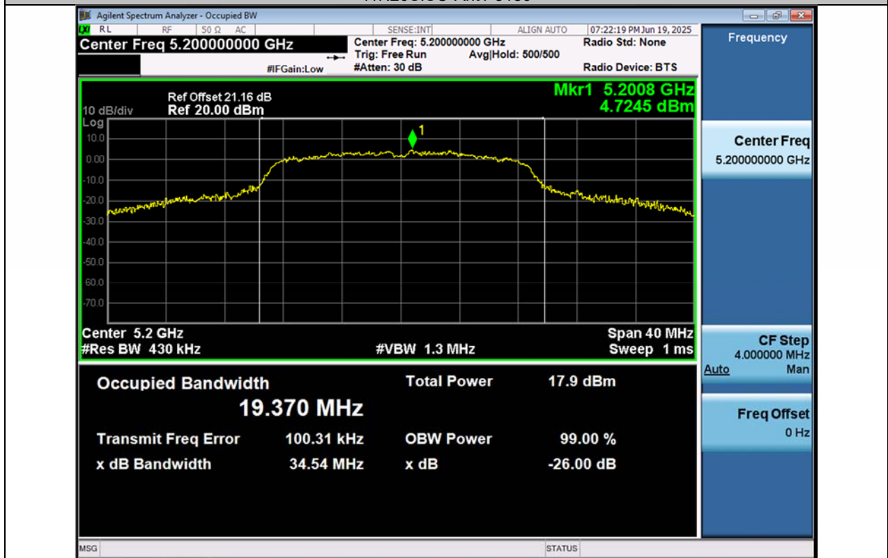
11N20SISO-Ant1-5200
