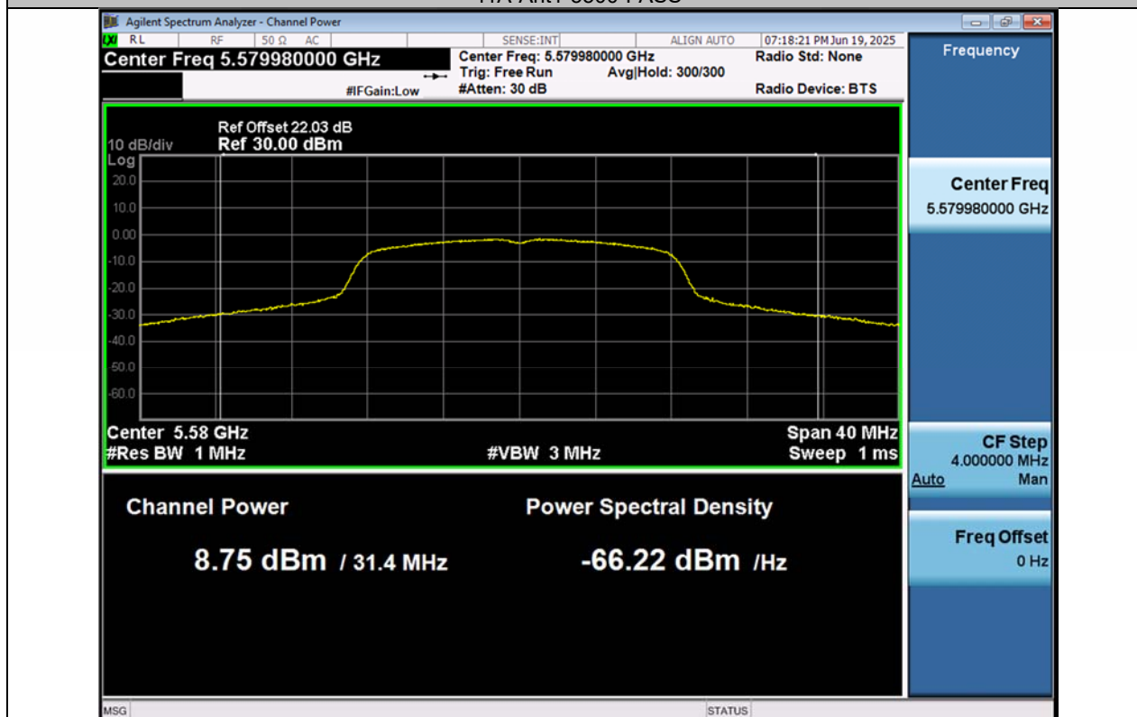
11A-Ant1-5580-PASS
