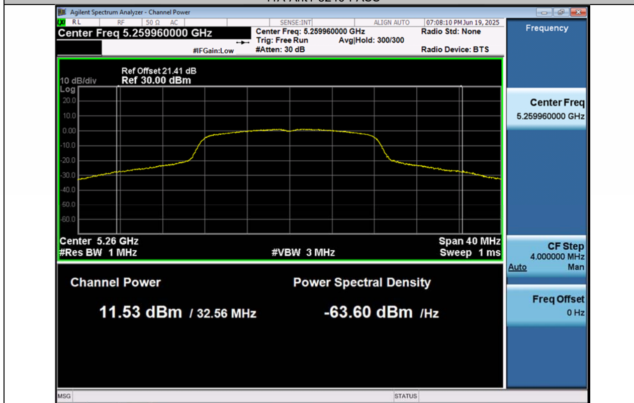
11A-Ant1-5260-PASS
