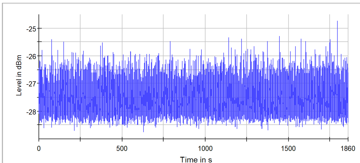
802.11a Channel 52
