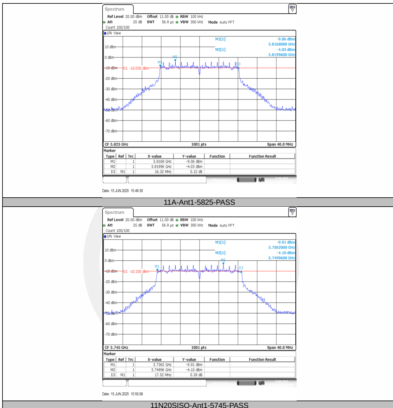
11N20SISO-Ant1-5745-PASS
