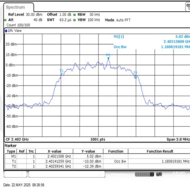
2DH5-Ant1-2402
