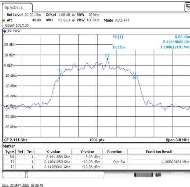
2DH5-Ant1-2441
