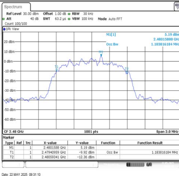
2DH5-Ant1-2480
