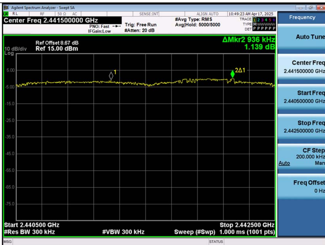
2DH5-Ant1-Hop_2441-PASS
