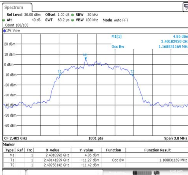
3DH5-Ant1-2402
