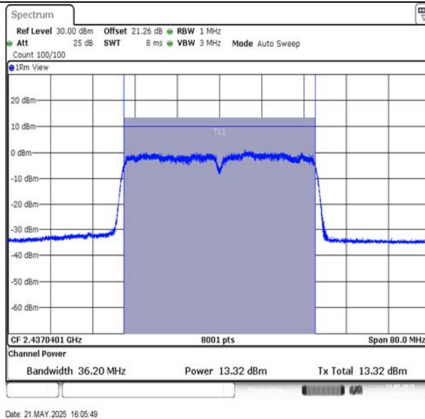
11N40SISO-Ant1-2437-PASS
