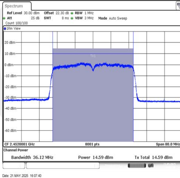
11N40SISO-Ant1-2452-PASS
