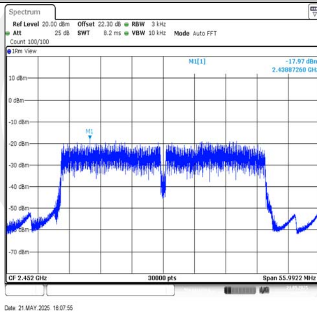
11N40SISO-Ant1-2452-PASS
