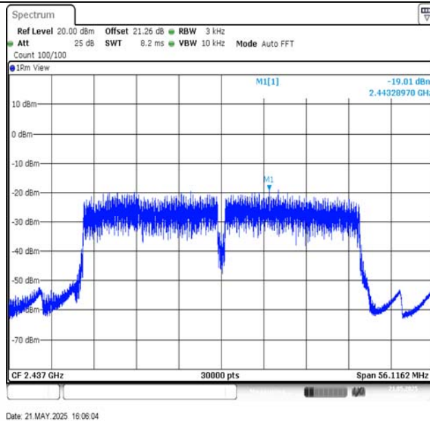
11N40SISO-Ant1-2437-PASS
