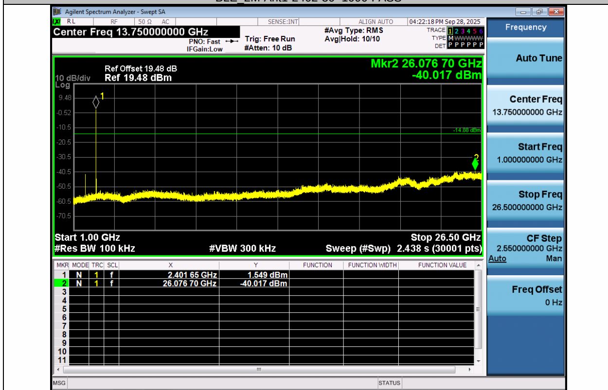
BLE_2M-Ant1-2402-1000~26500-PASS
