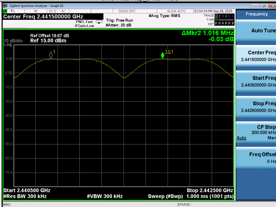
DH5-Ant1-Hop_2441-PASS
