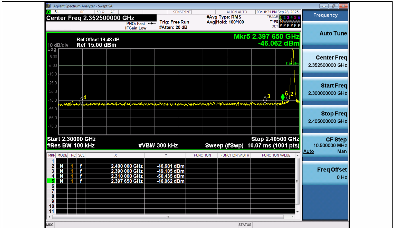
DH5-Ant1-2402-PASS
