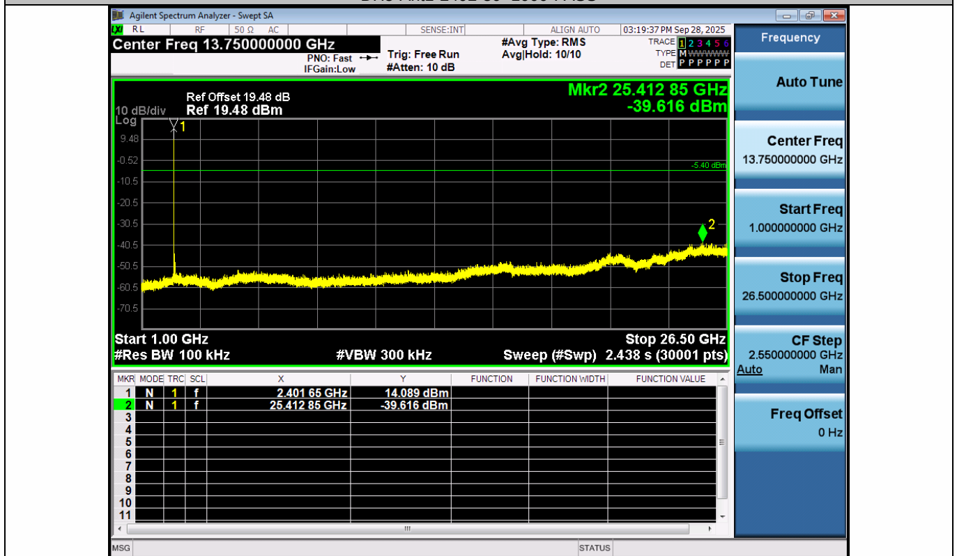
DH5-Ant1-2402-1000~26500-PASS
