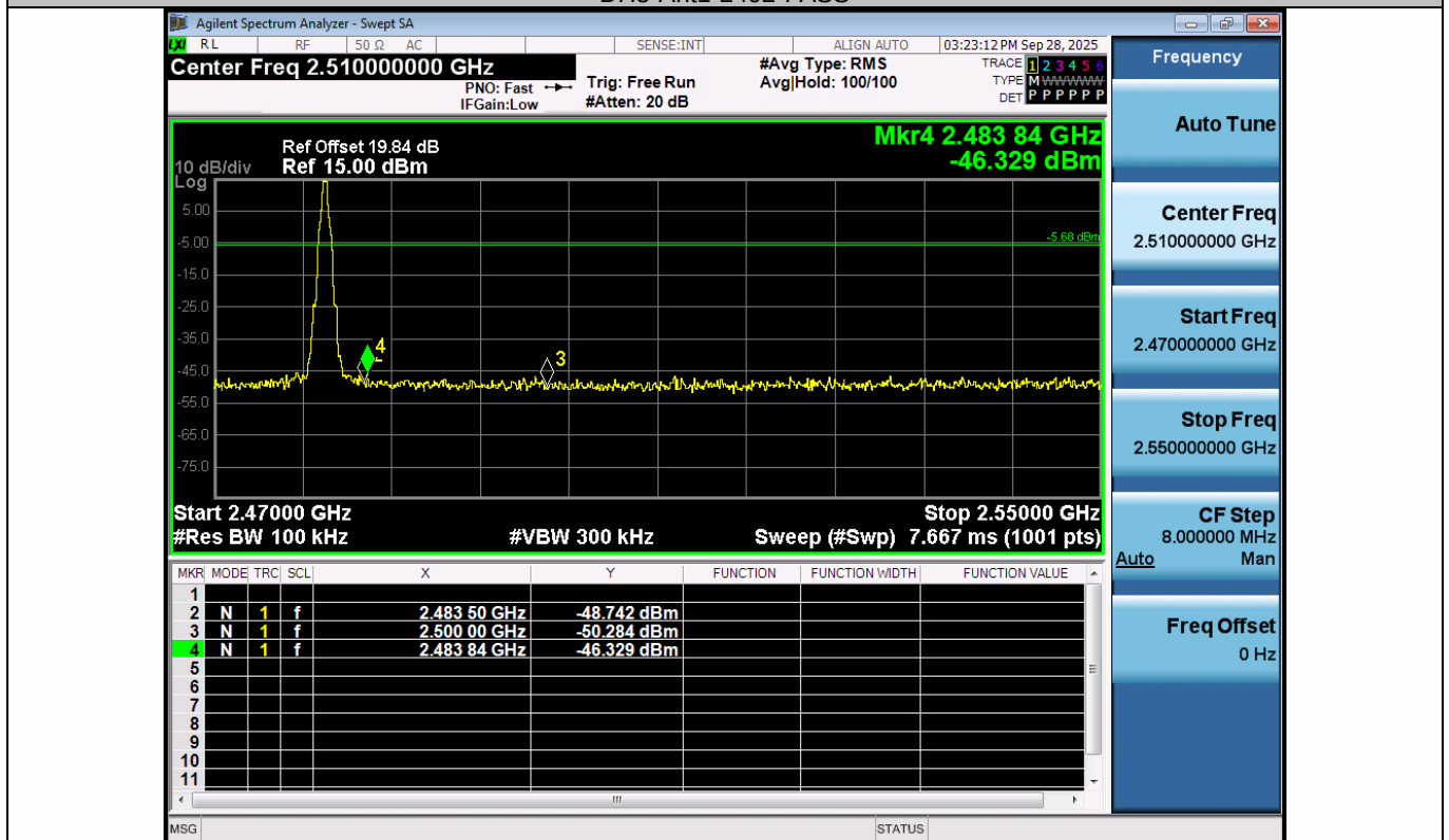
DH5-Ant1-2480-PASS
