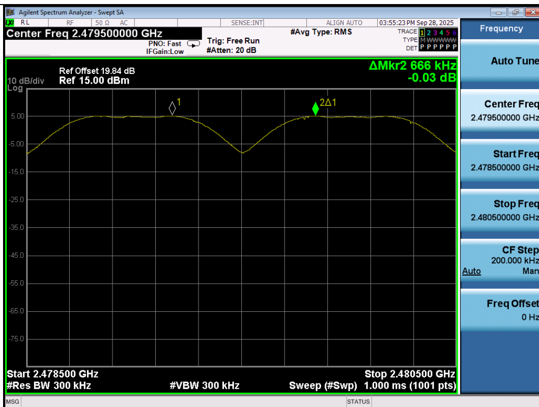
DH5-Ant1-Hop_2480-PASS
