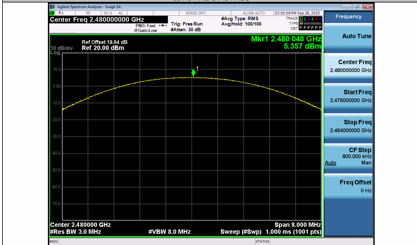
2DH5-Ant1-2480-PASS
