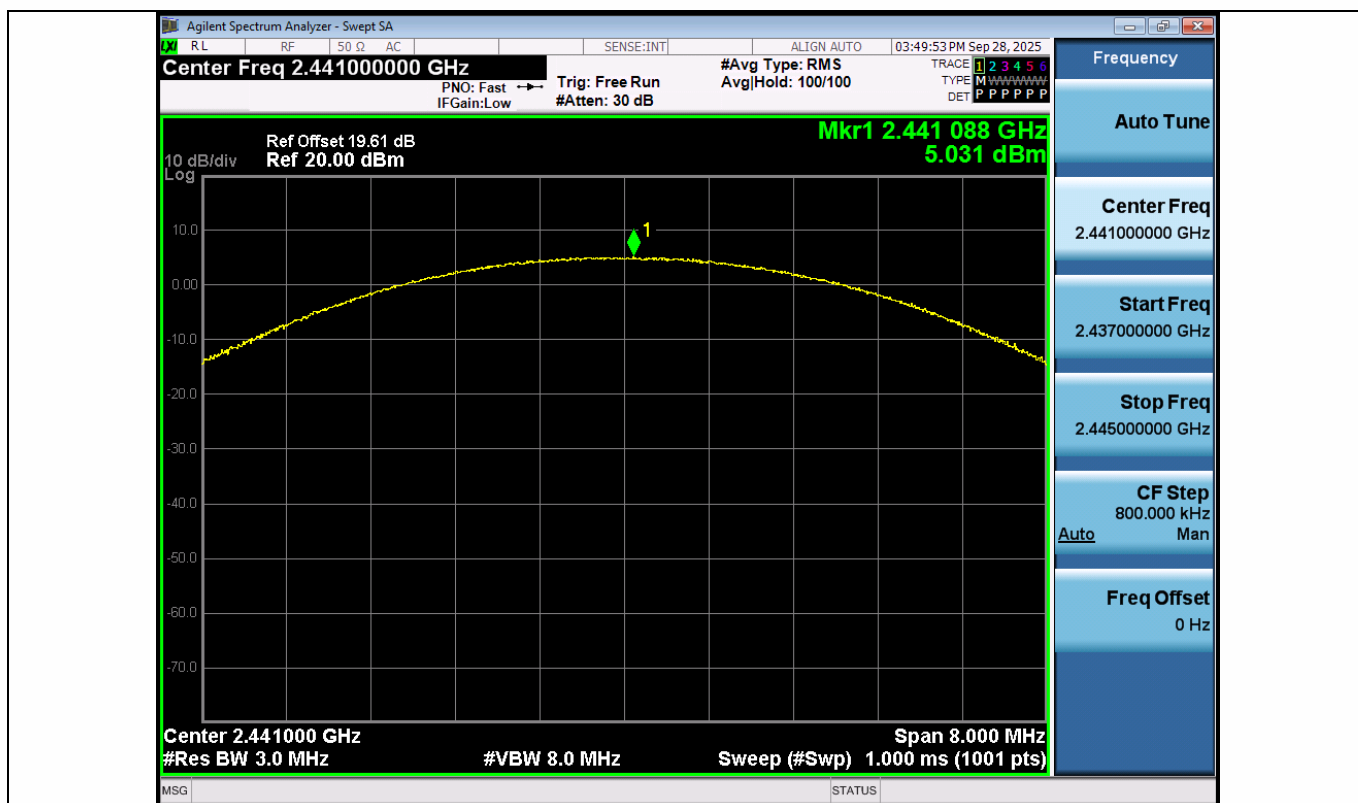
2DH5-Ant1-2441-PASS
