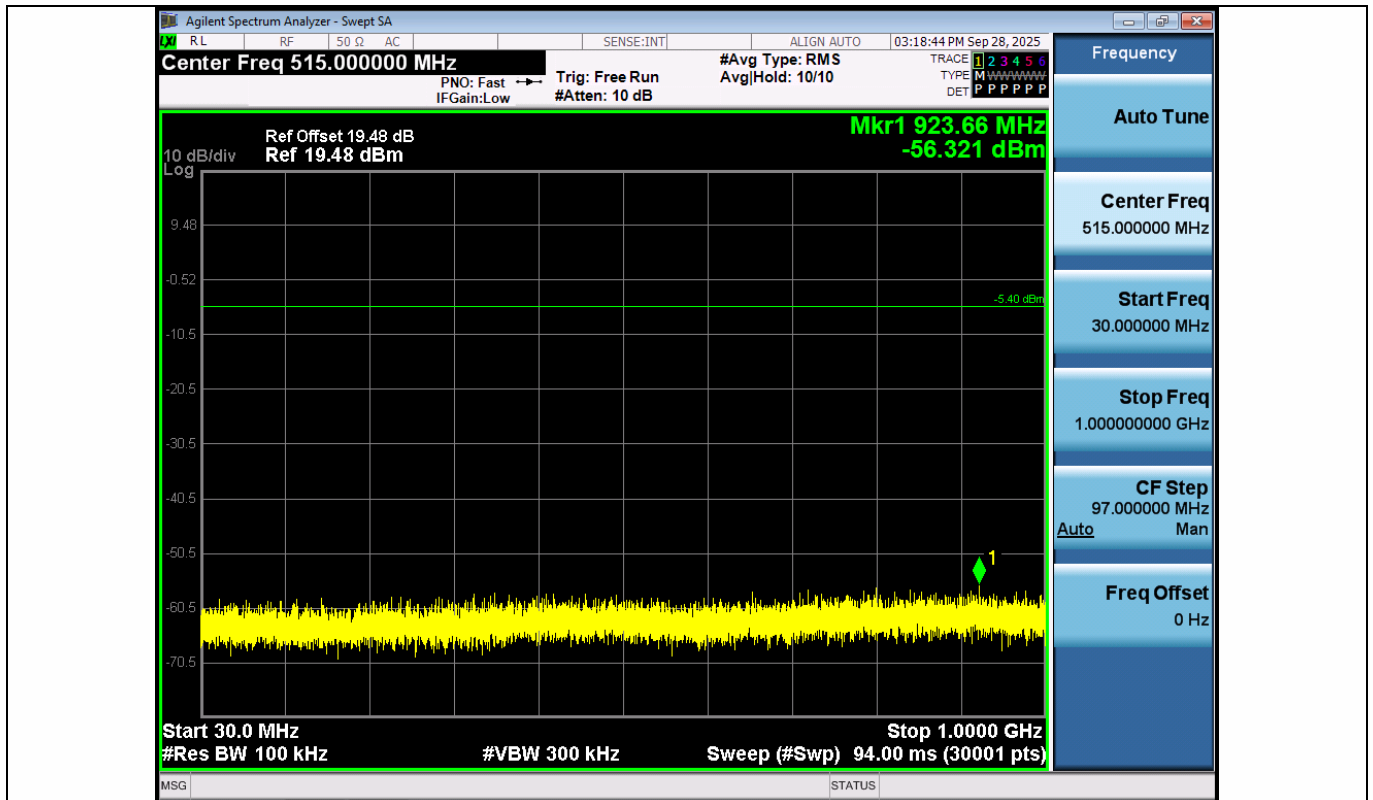
DH5-Ant1-2402-30~1000-PASS
