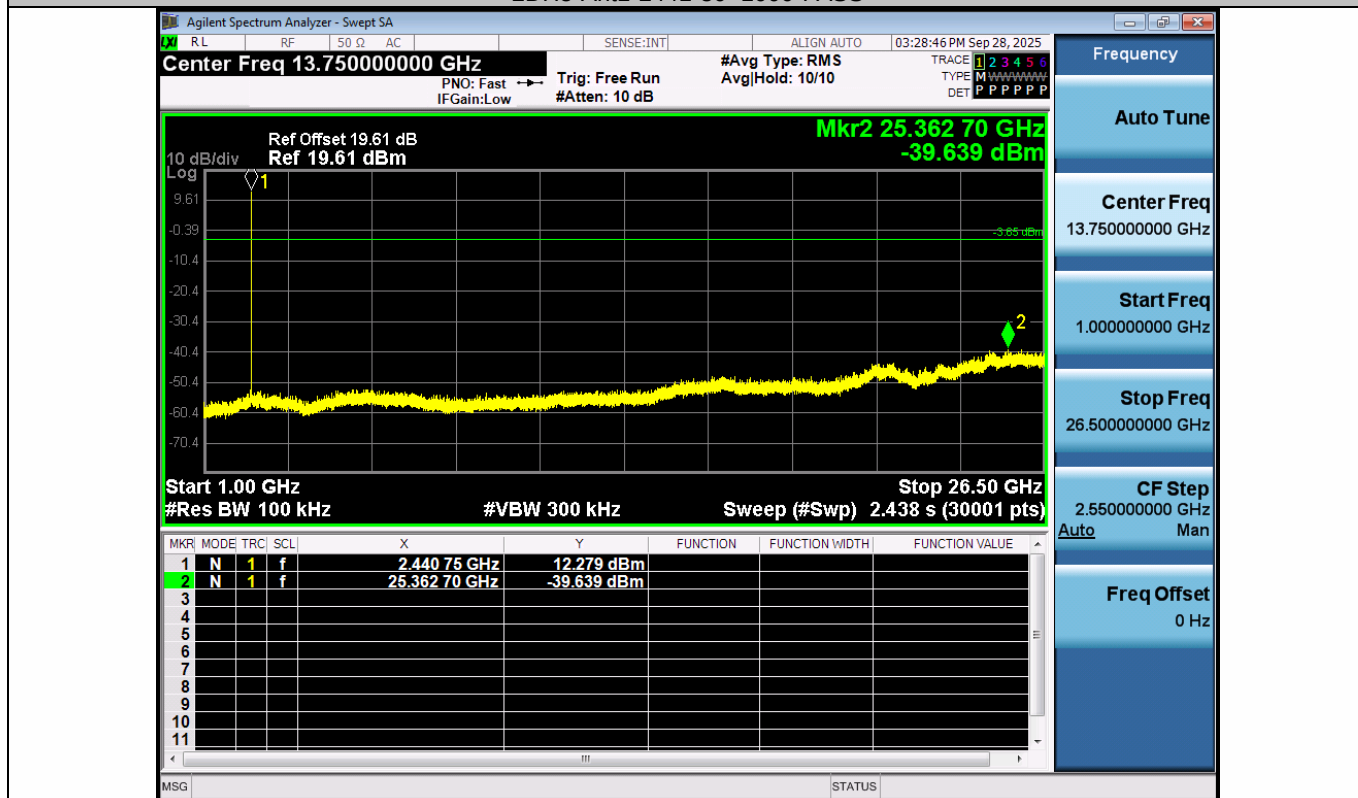
2DH5-Ant1-2441-1000~26500-PASS
