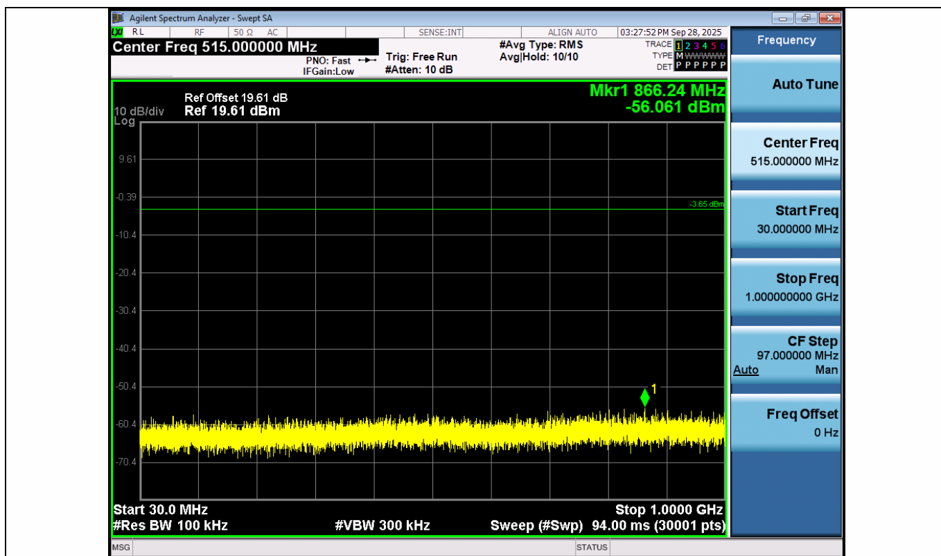
2DH5-Ant1-2441-30~1000-PASS
