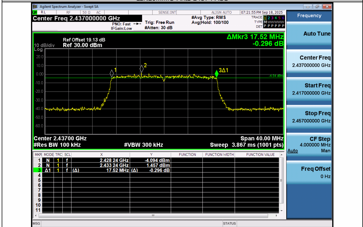
11N20MIMO-Ant2-2437-PASS
