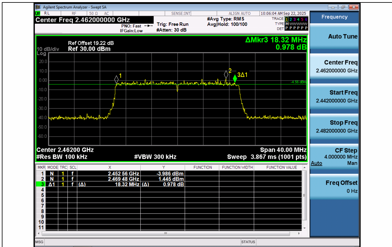
11AX20MIMO-Ant1-2462-PASS
