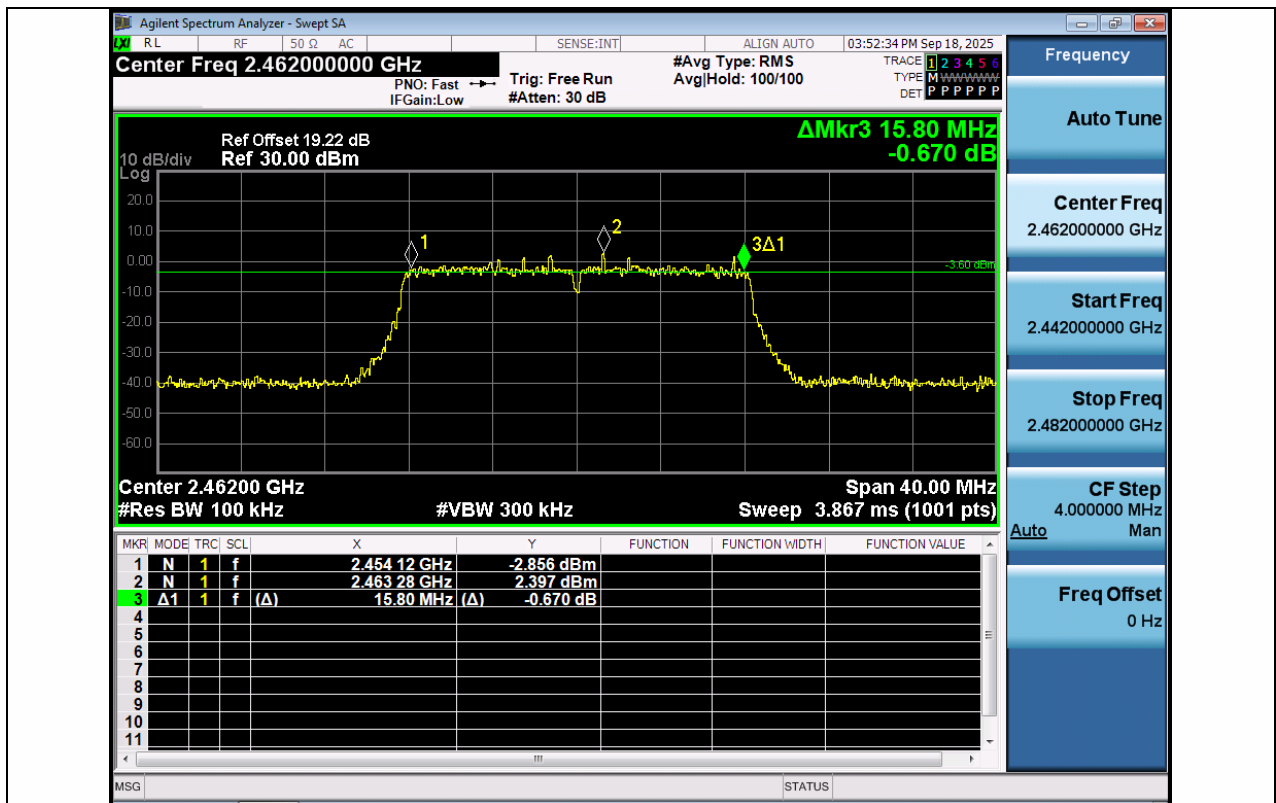
11G-Ant1-2462-PASS
