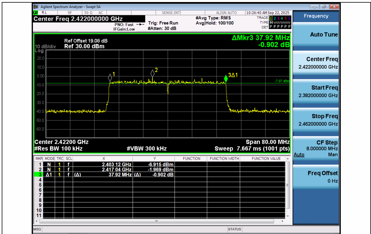
11AX40MIMO-Ant1-2422-PASS
