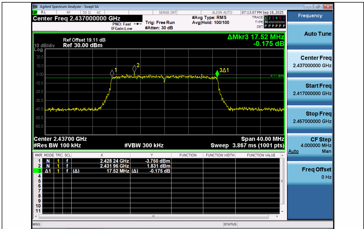
11N20MIMO-Ant1-2437-PASS
