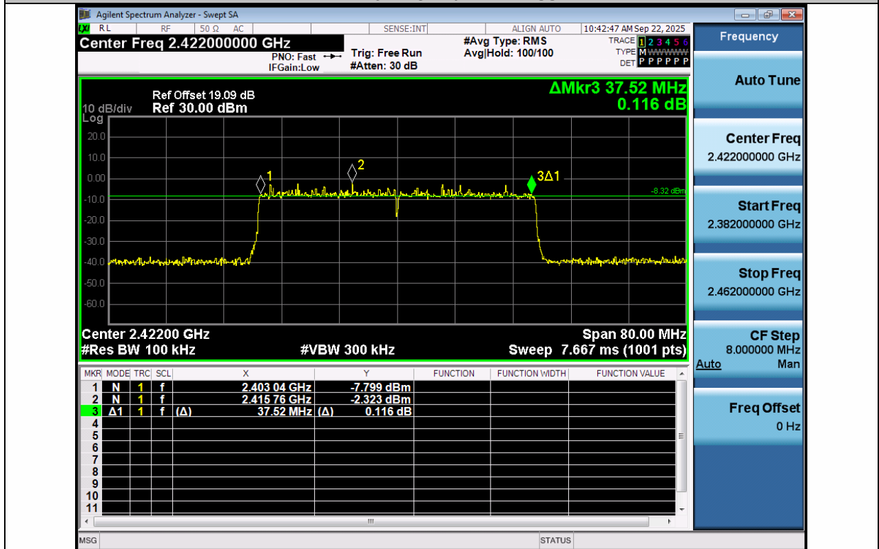
11AX40MIMO-Ant2-2422-PASS
