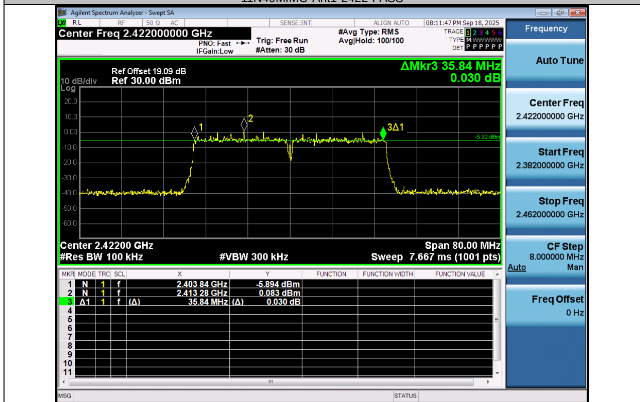
11N40MIMO-Ant2-2422-PASS
