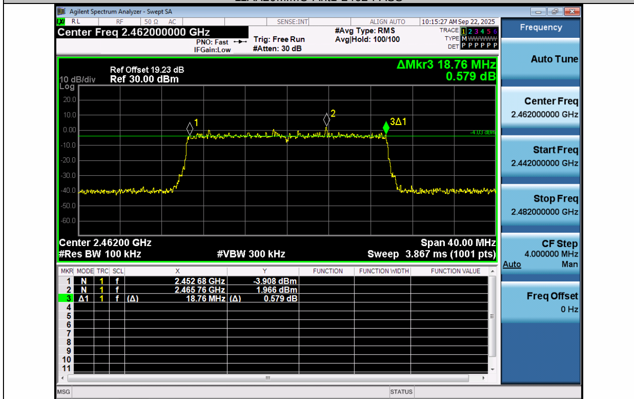
11AX20MIMO-Ant2-2462-PASS
