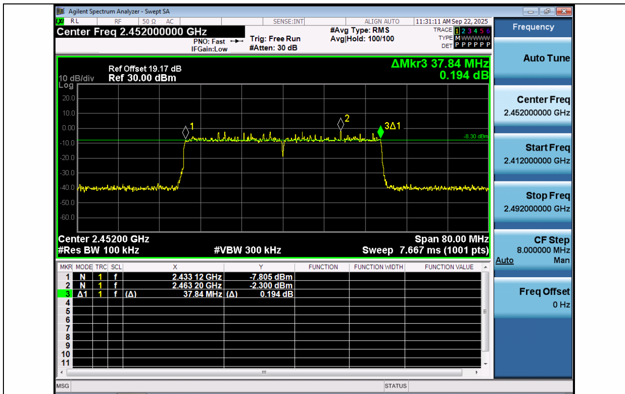
11AX40MIMO-Ant1-2452-PASS
