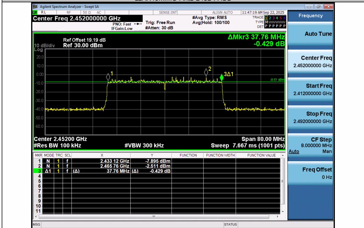
11AX40MIMO-Ant2-2452-PASS
