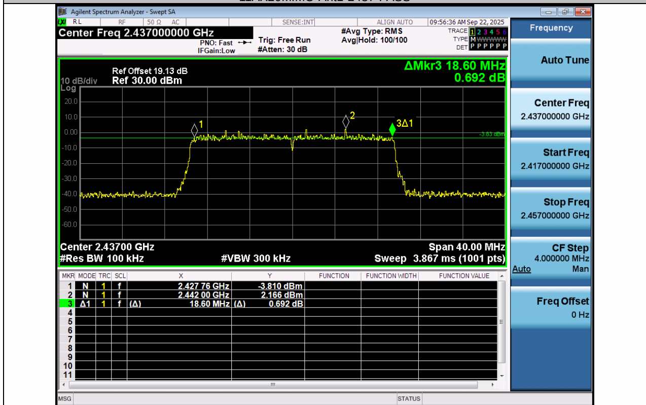
11AX20MIMO-Ant2-2437-PASS
