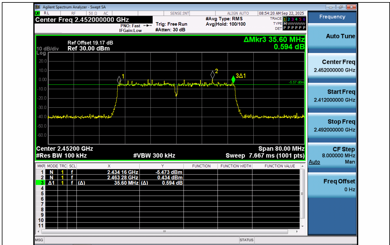
11N40MIMO-Ant1-2452-PASS
