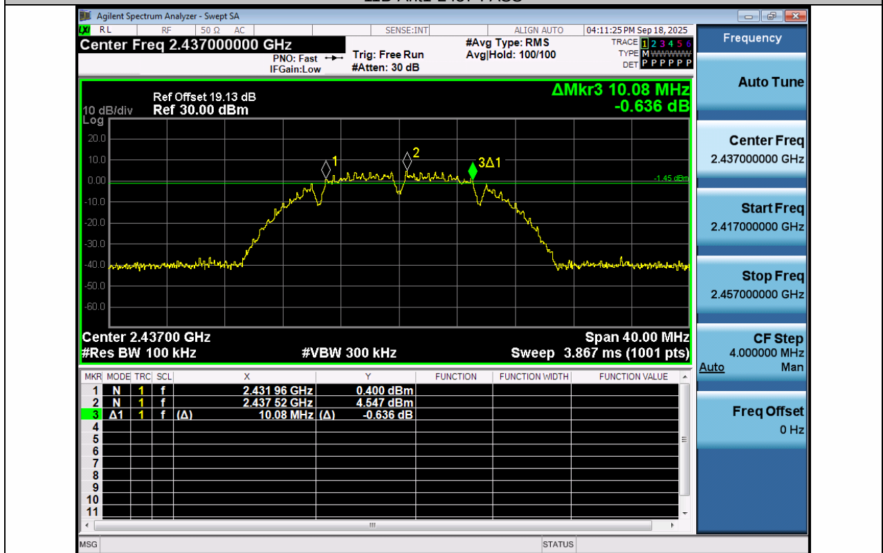
11B-Ant2-2437-PASS
