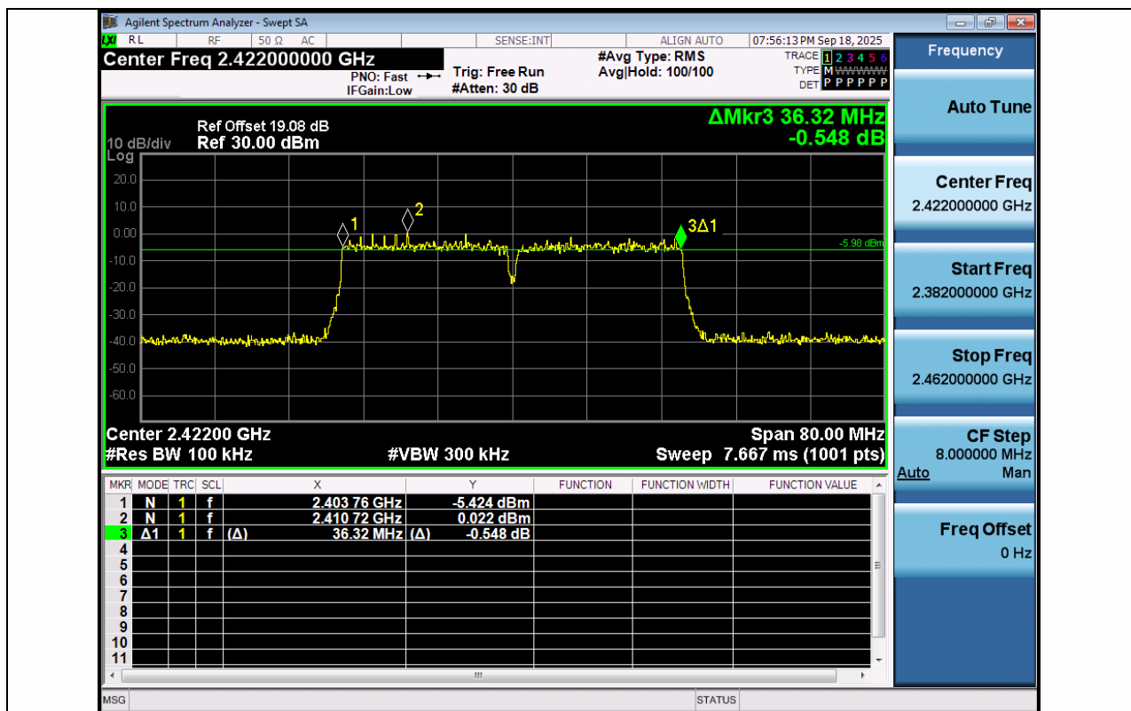
11N40MIMO-Ant1-2422-PASS
