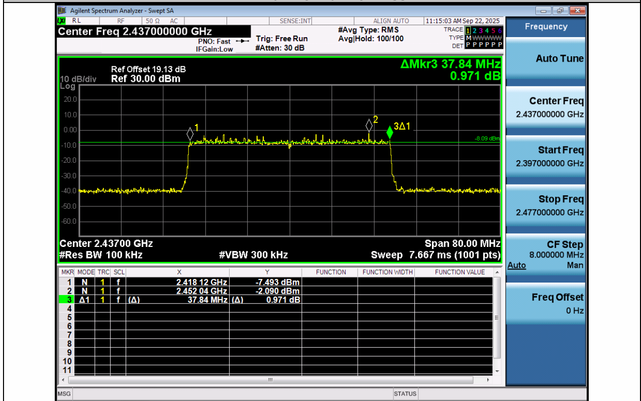
11AX40MIMO-Ant2-2437-PASS
