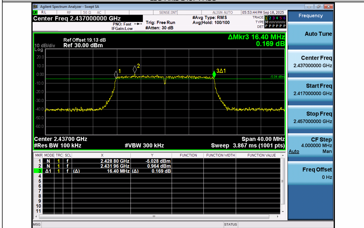
11G-Ant2-2437-PASS
