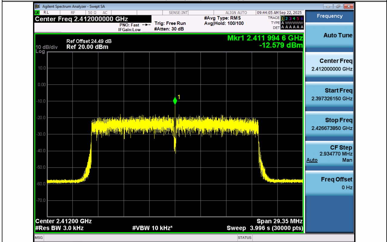
11AX20MIMO-Ant2-2412-PASS
