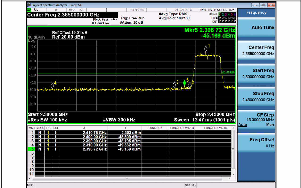
11G-Ant2-2412-PASS
