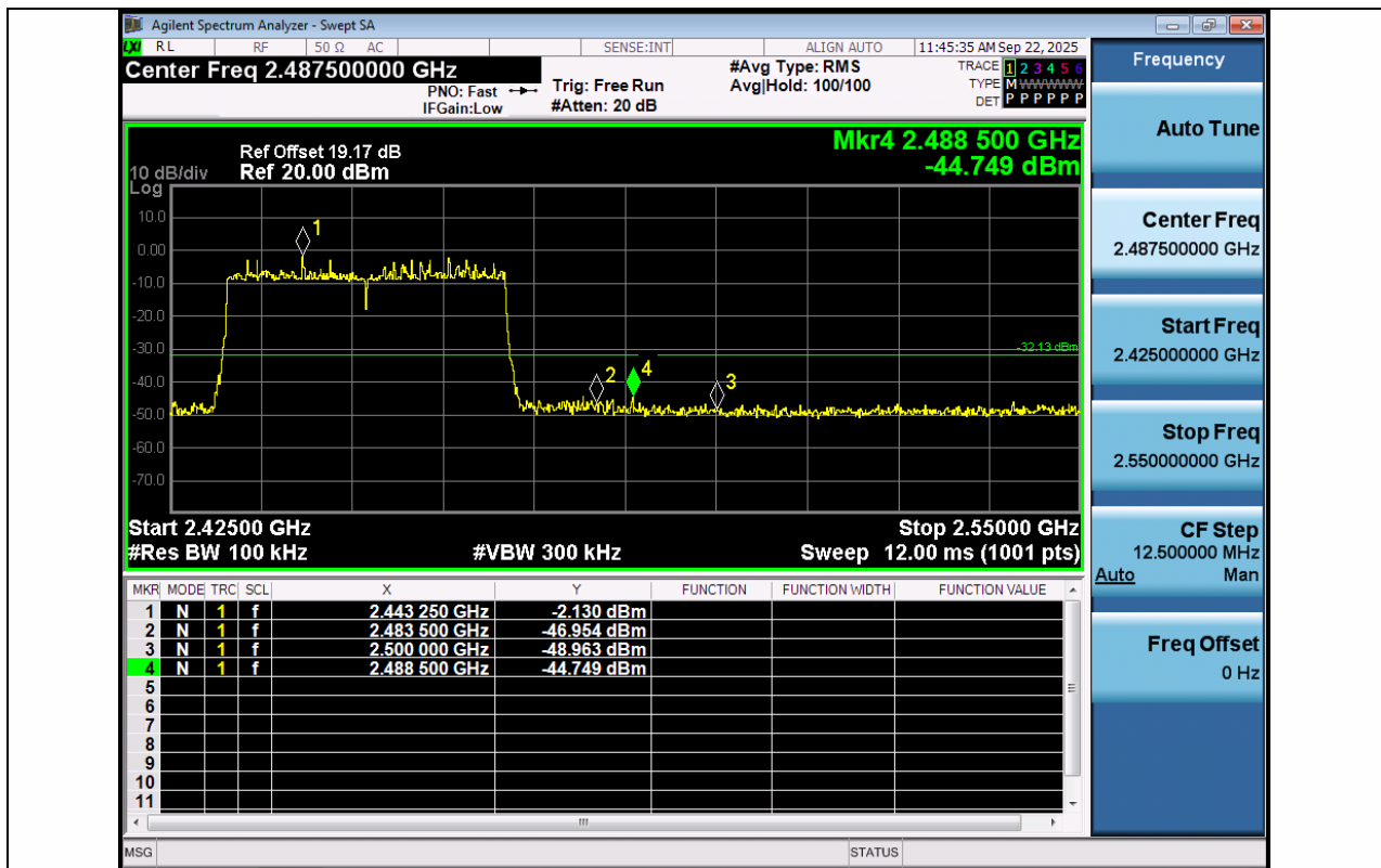
11AX40MIMO-Ant1-2452-PASS
