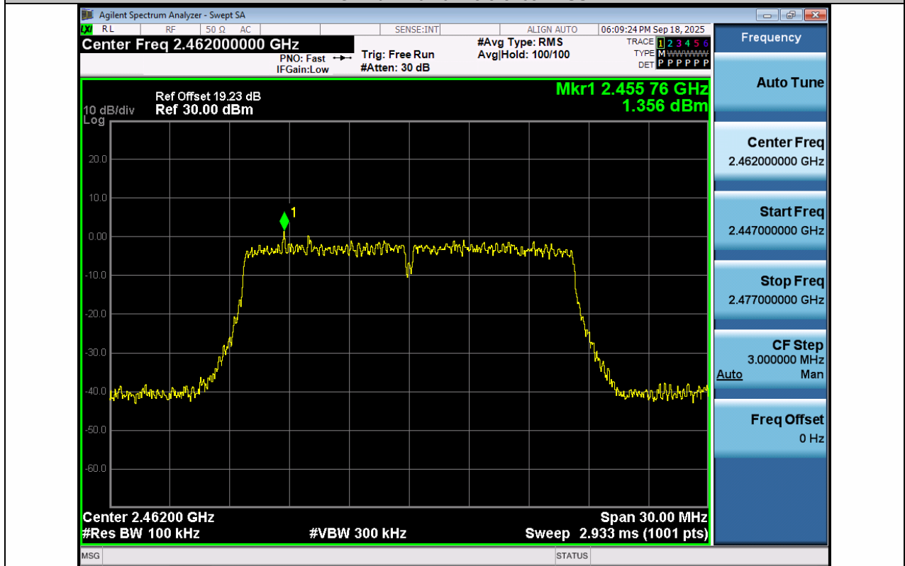
11G-Ant2-2462-0~Reference-PASS
