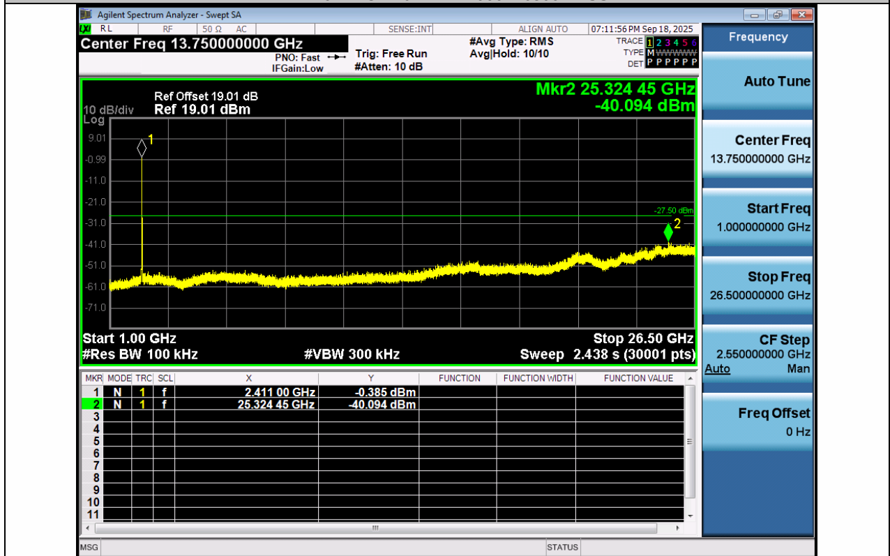
11N20MIMO-Ant2-2412-1000~26500-PASS
