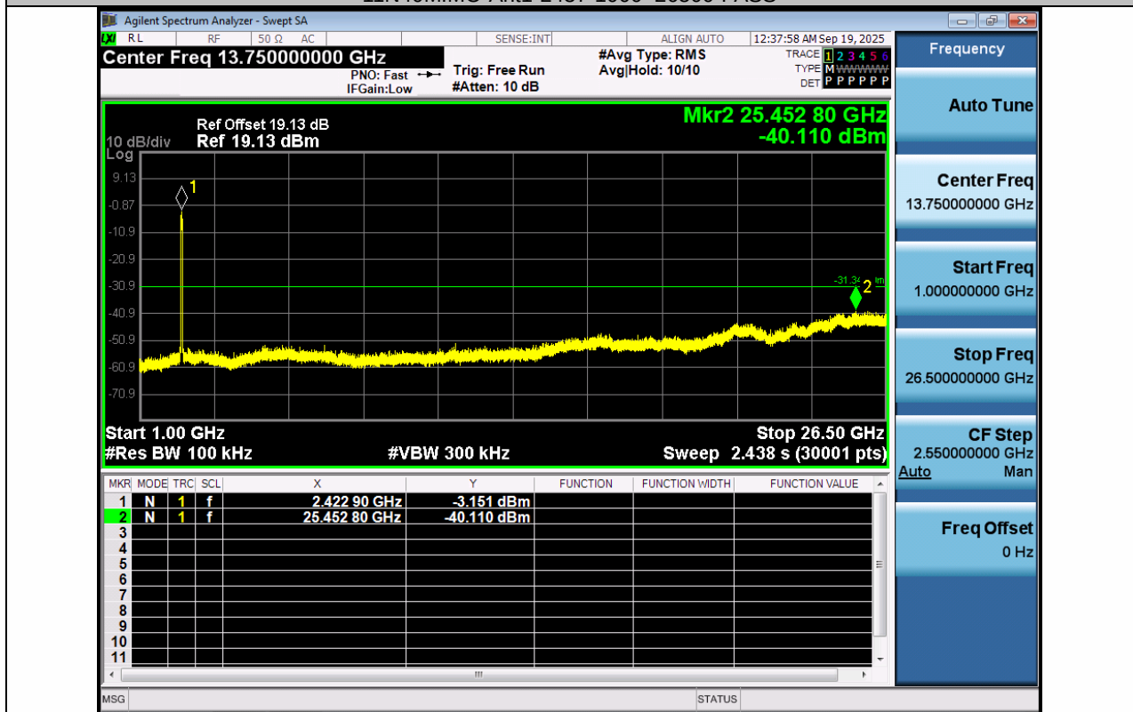
11N40MIMO-Ant2-2437-1000~26500-PASS
