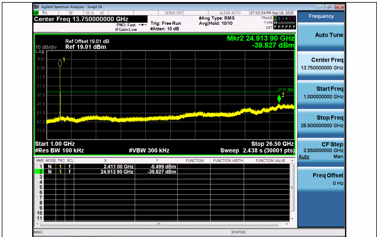
11N20MIMO-Ant1-2412-1000~26500-PASS
