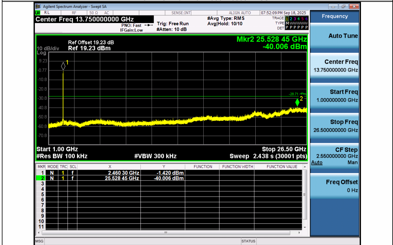
11N20MIMO-Ant2-2462-1000~26500-PASS
