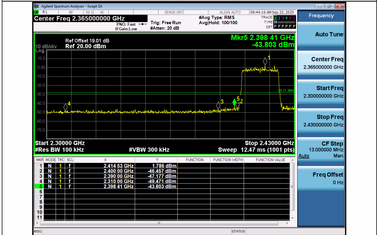
11AX20MIMO-Ant2-2412-PASS
