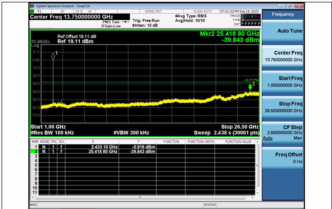
11N20MIMO-Ant1-2437-1000~26500-PASS
