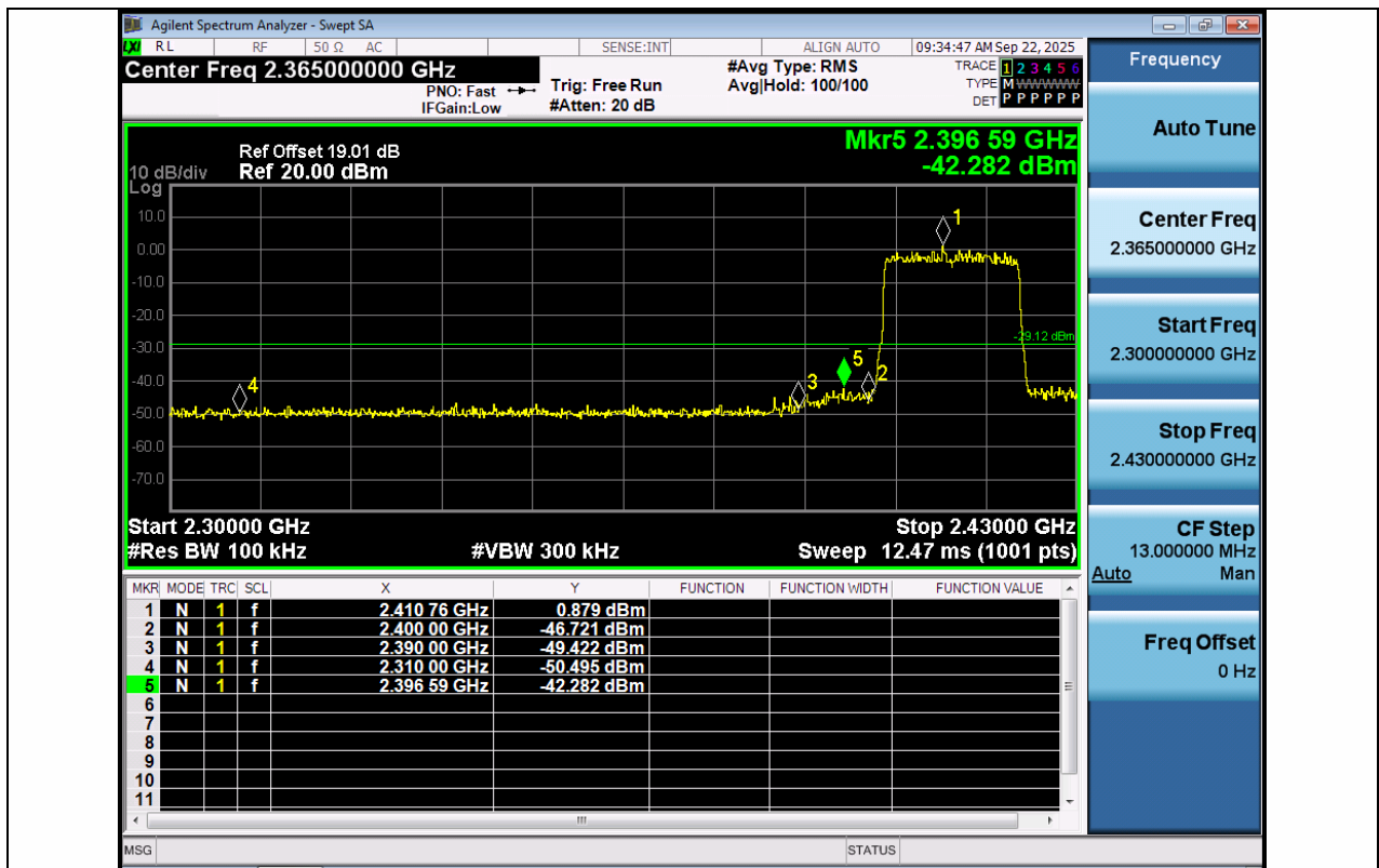
11AX20MIMO-Ant1-2412-PASS
