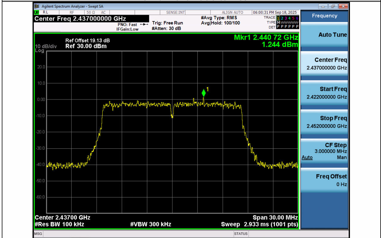
11G-Ant2-2437-0~Reference-PASS
