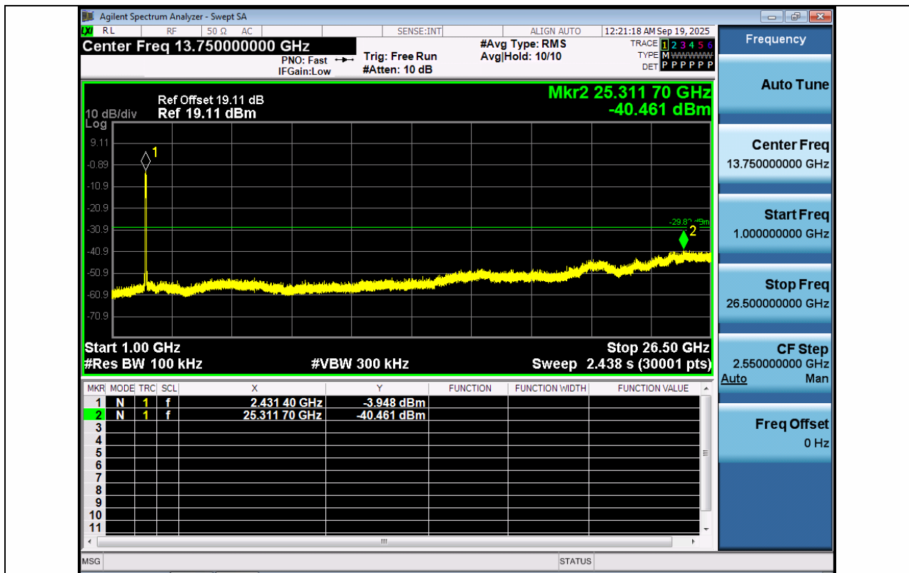
11N40MIMO-Ant1-2437-1000~26500-PASS
