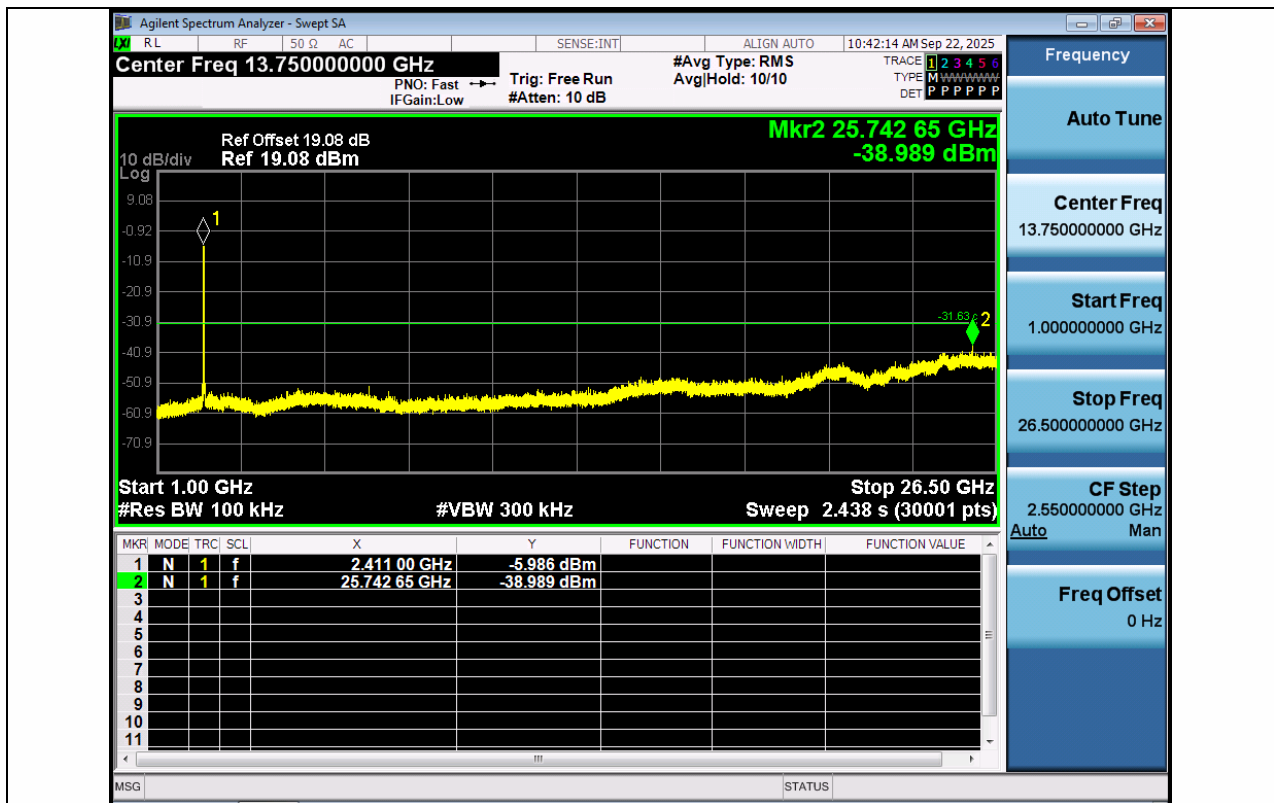
11AX40MIMO-Ant1-2422-1000~26500-PASS
