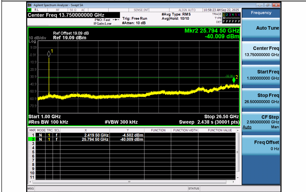
11AX40MIMO-Ant2-2422-1000~26500-PASS
