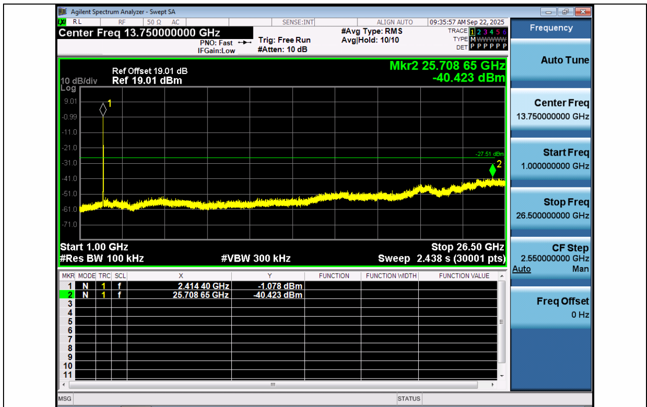
11AX20MIMO-Ant1-2412-1000~26500-PASS
