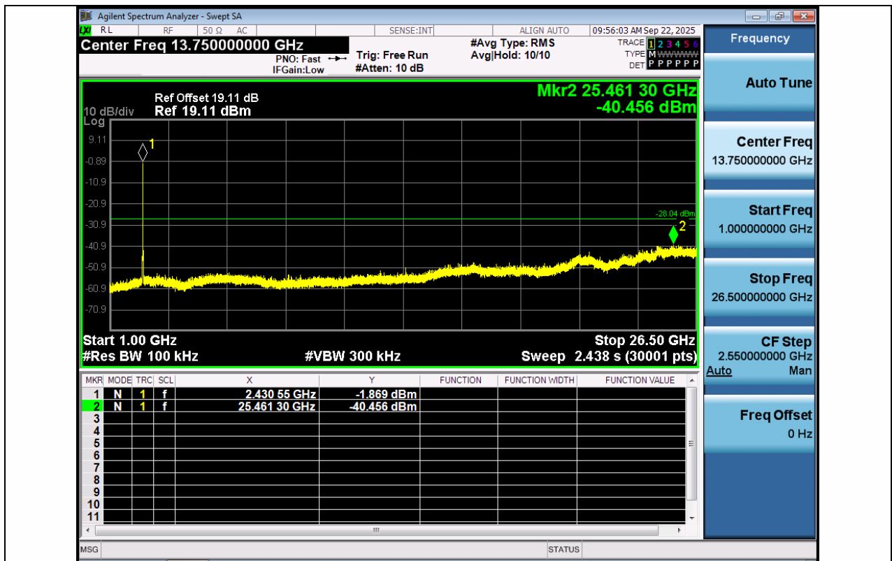
11AX20MIMO-Ant1-2437-1000~26500-PASS
