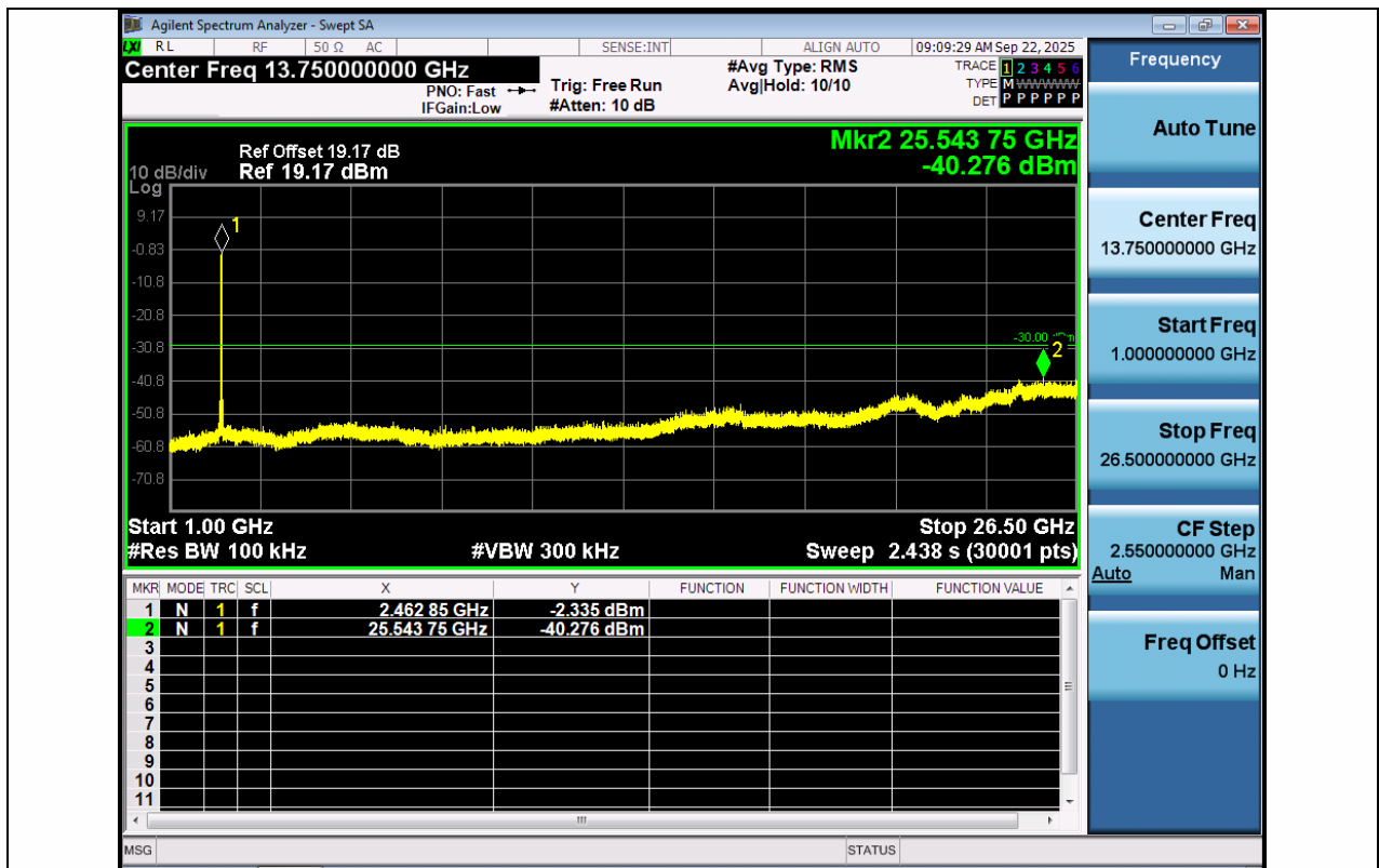
11N40MIMO-Ant1-2452-1000~26500-PASS
