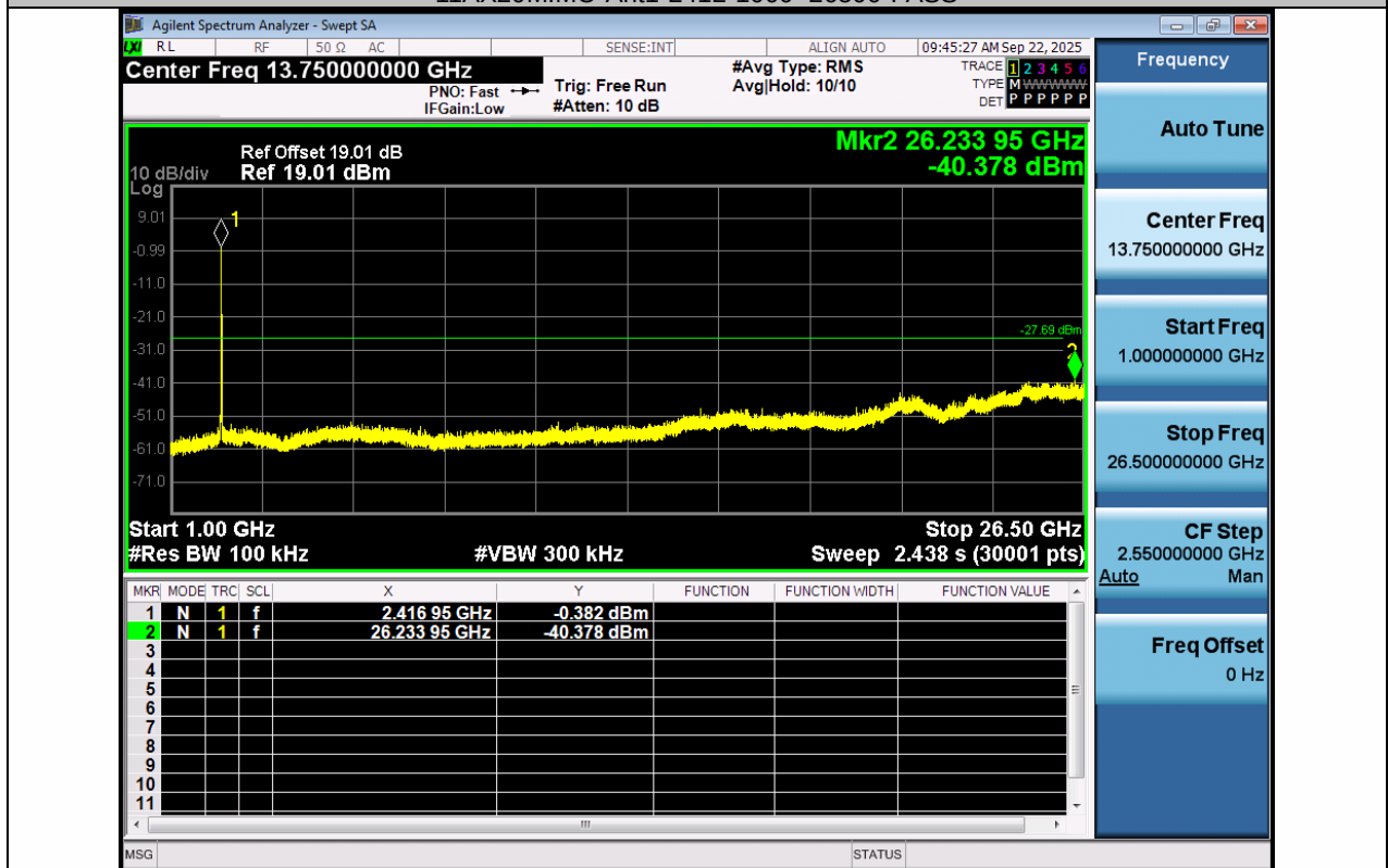
11AX20MIMO-Ant2-2412-1000~26500-PASS
