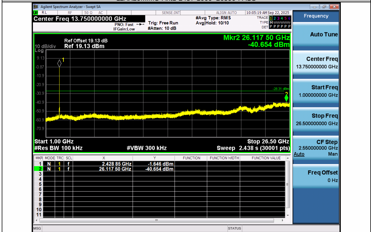
11AX20MIMO-Ant2-2437-1000~26500-PASS
