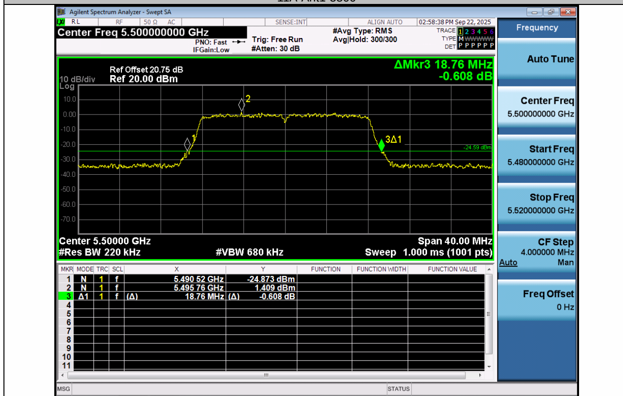
11A-Ant2-5500
