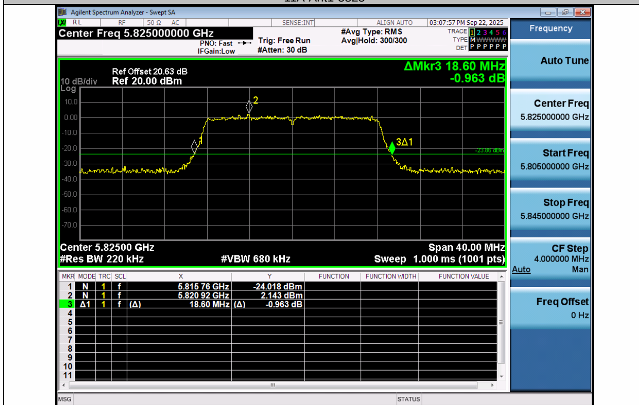
11A-Ant2-5825
