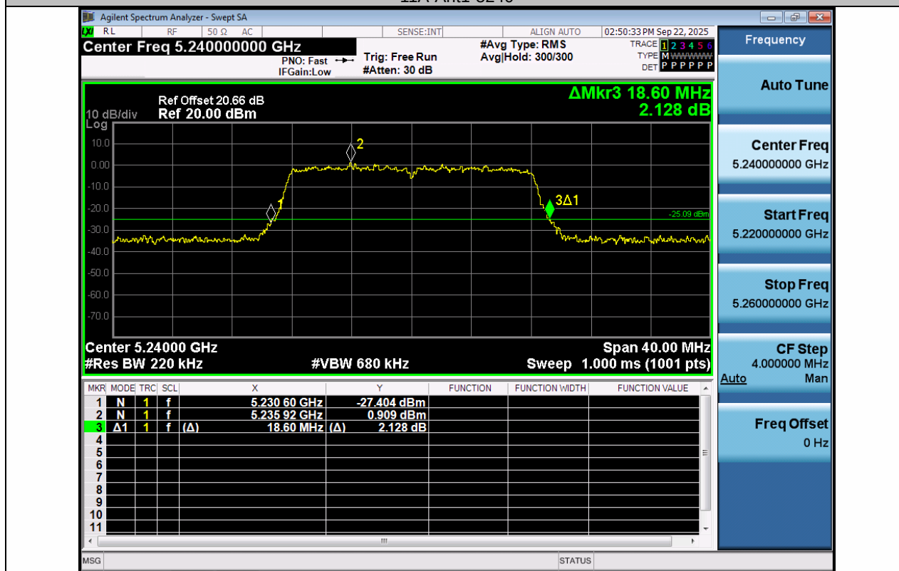
11A-Ant2-5240
