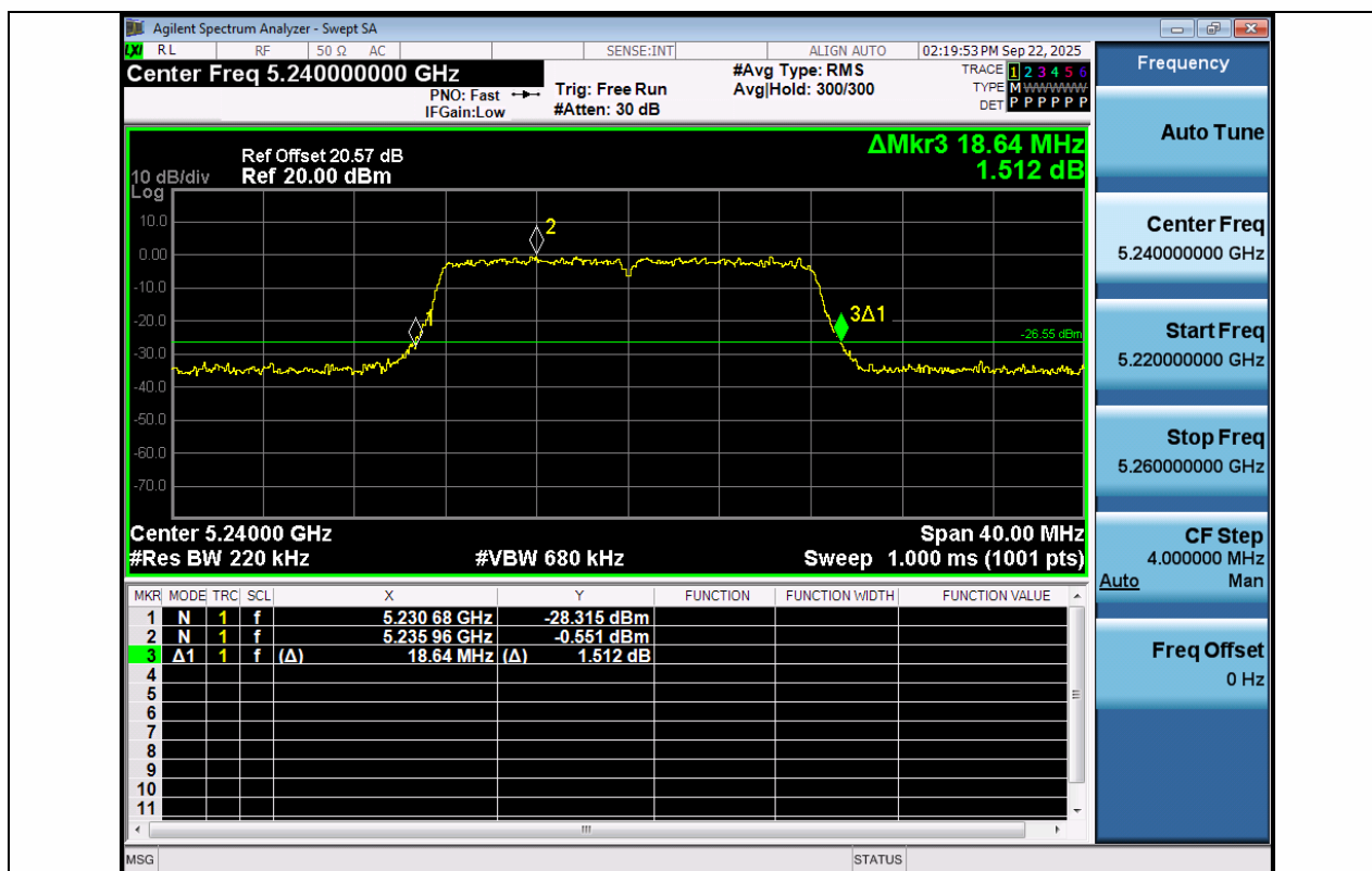
11A-Ant1-5240
