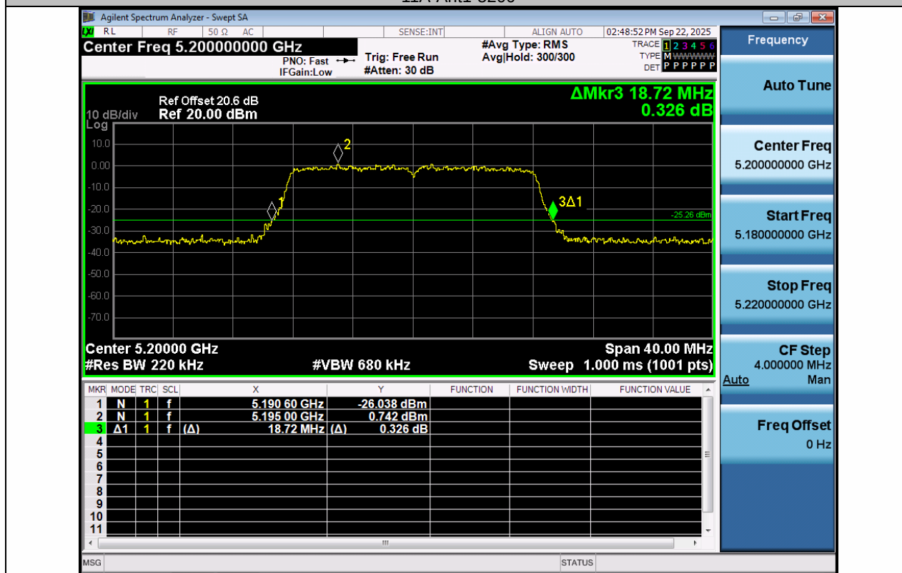
11A-Ant2-5200
