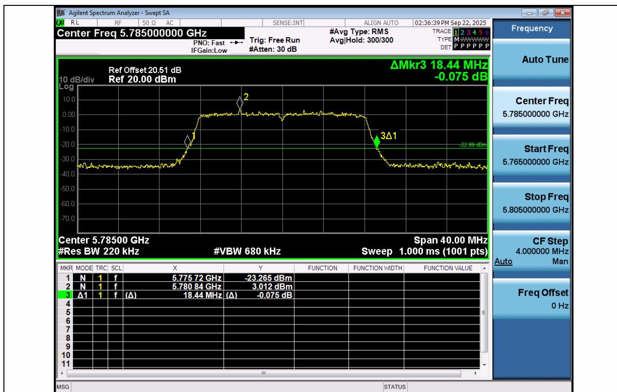
11A-Ant1-5785
