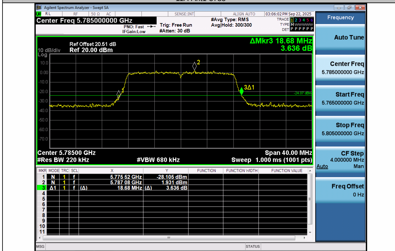
11A-Ant2-5785
