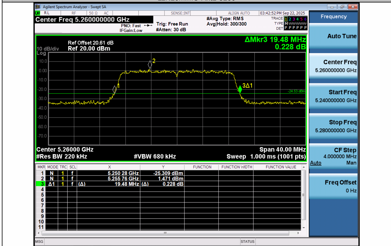
11N20MIMO-Ant2-5260
