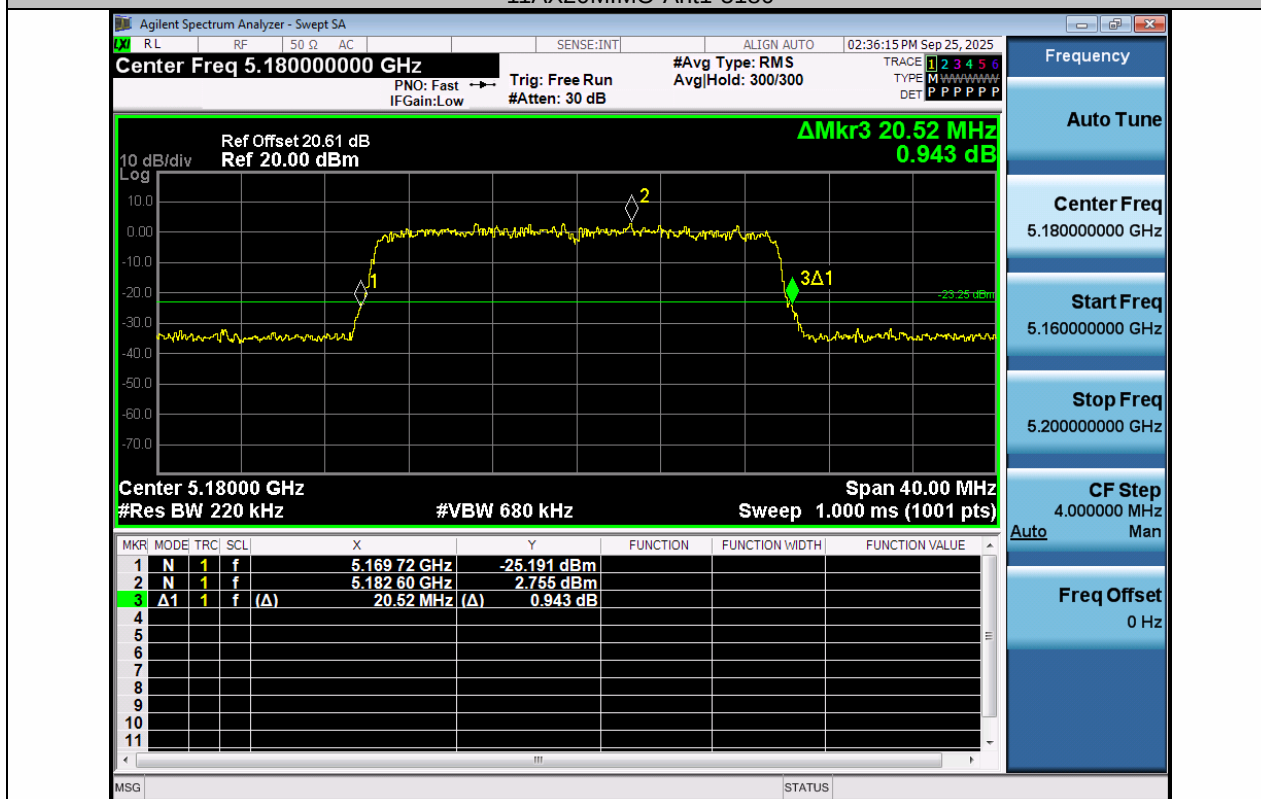
11AX20MIMO-Ant2-5180
