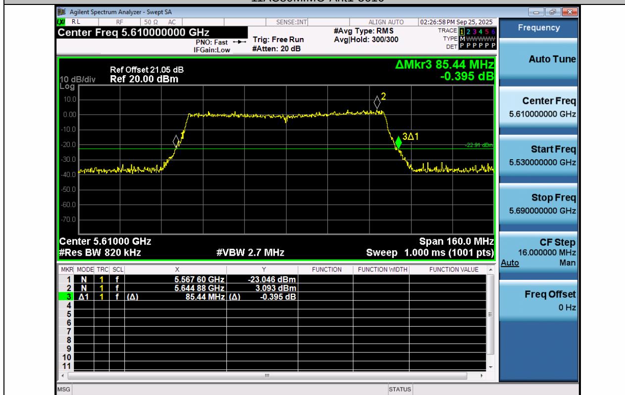
11AC80MIMO-Ant2-5610
