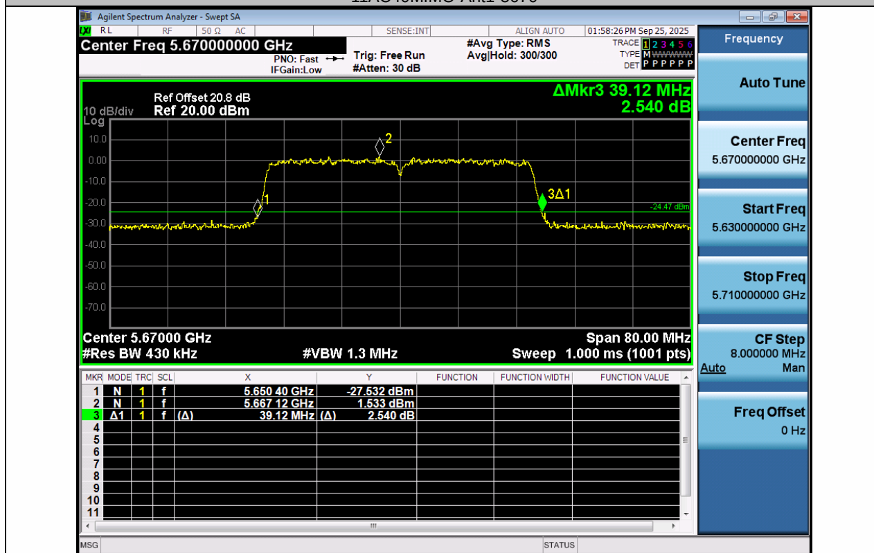
11AC40MIMO-Ant2-5670
