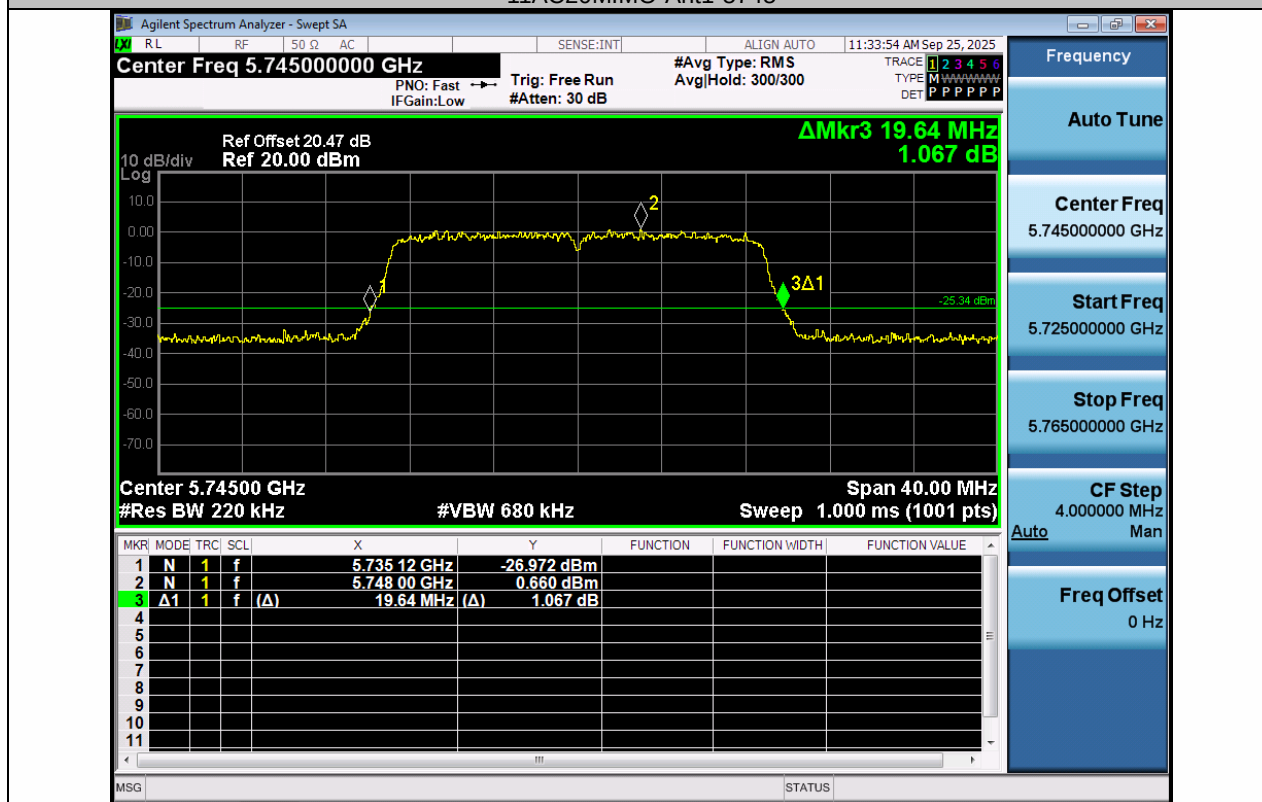
11AC20MIMO-Ant2-5745
