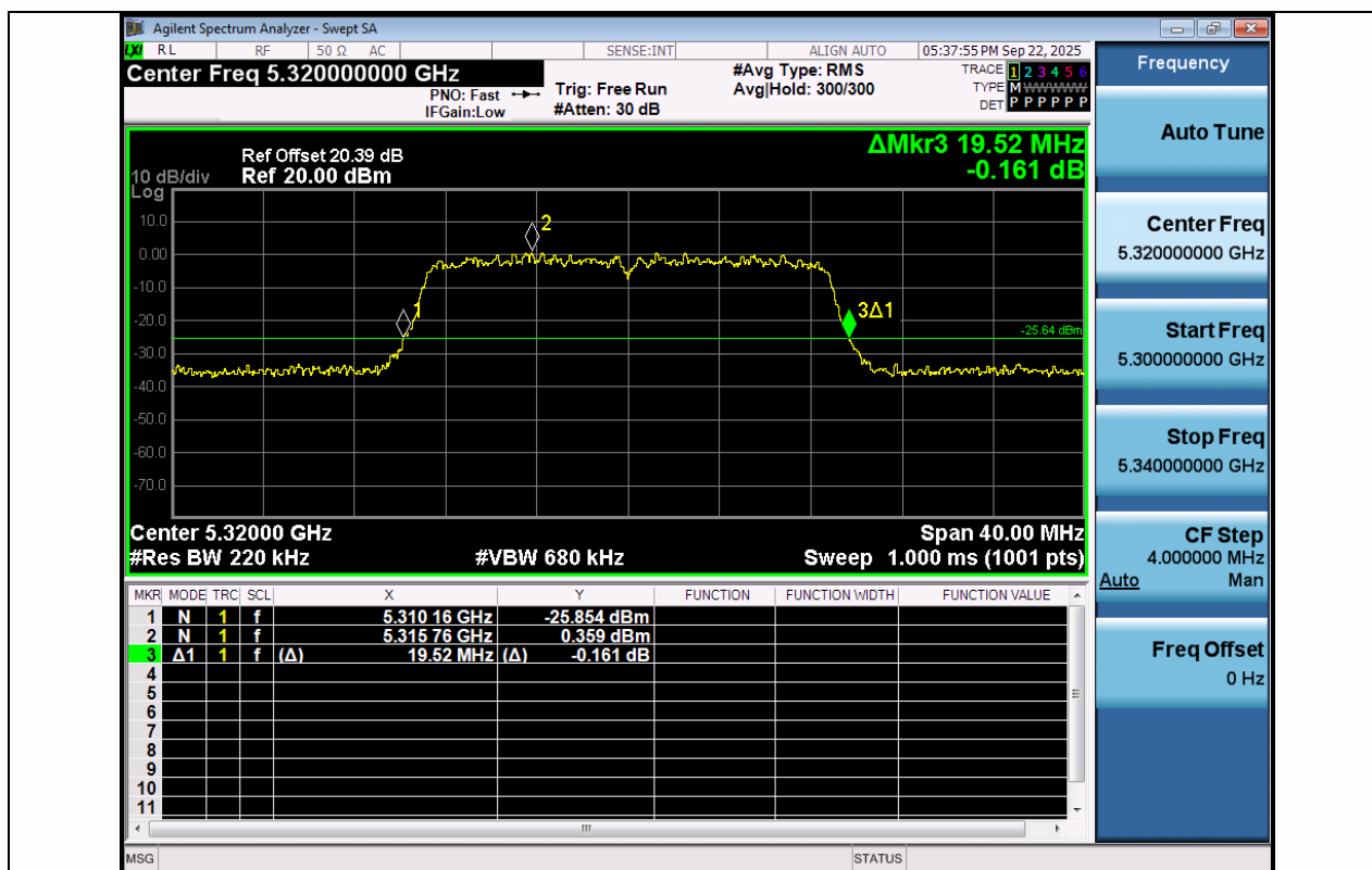
11AC20MIMO-Ant1-5320
