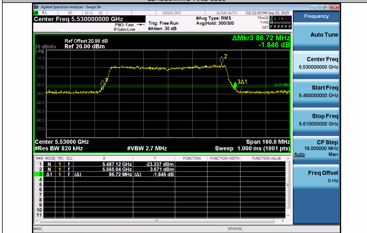
11AC80MIMO-Ant2-5530
