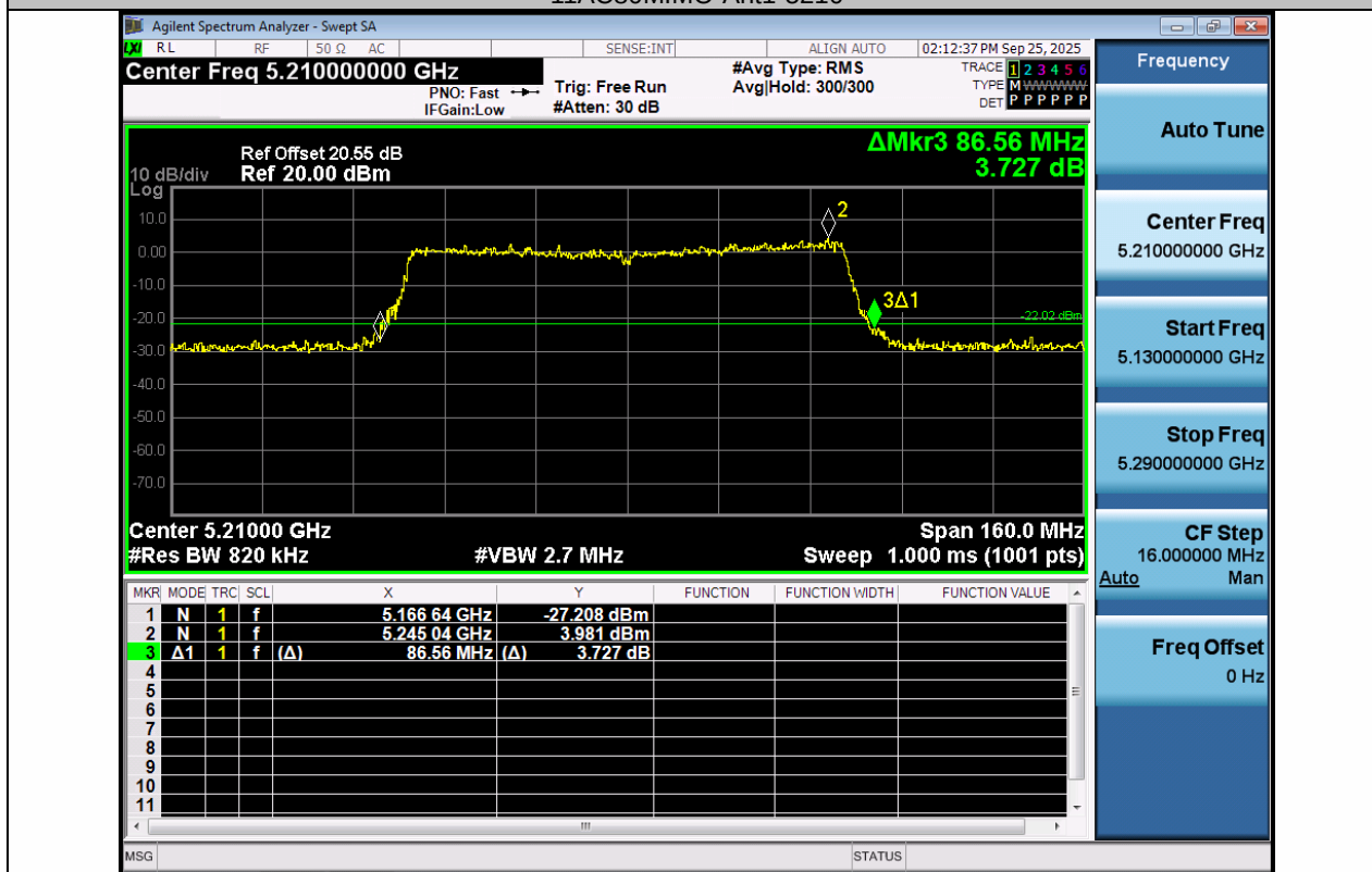
11AC80MIMO-Ant2-5210
