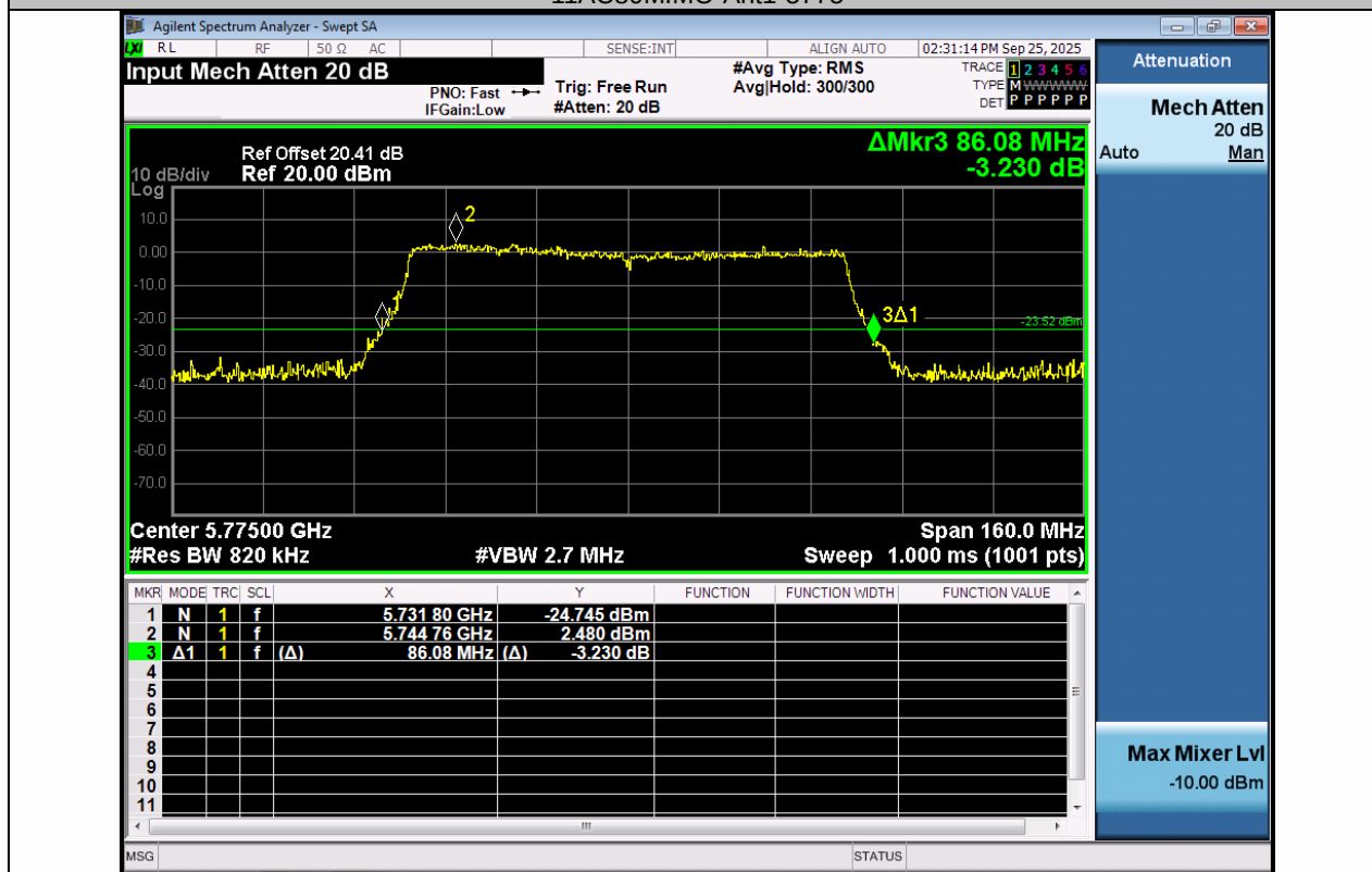
11AC80MIMO-Ant2-5775
