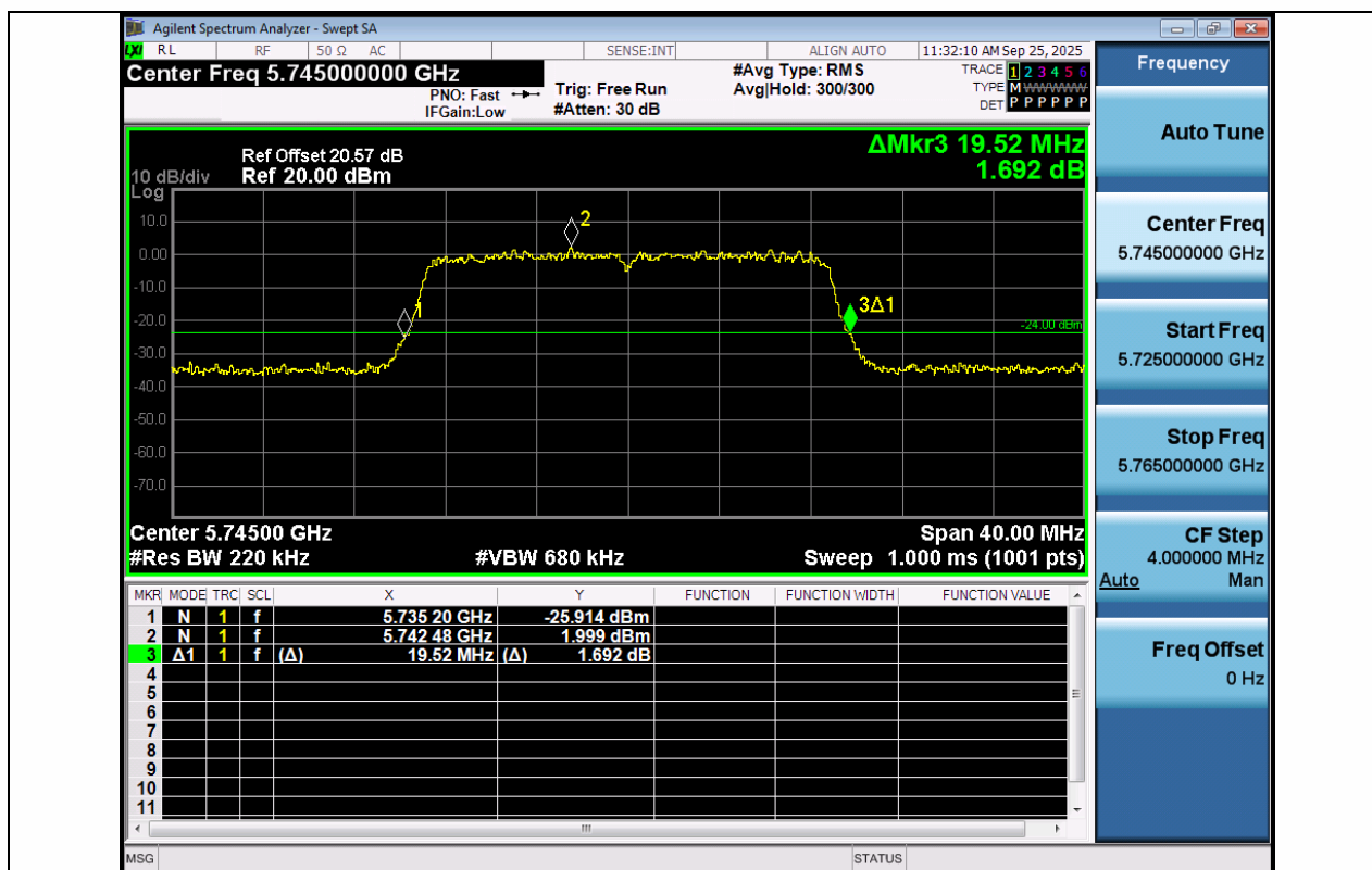
11AC20MIMO-Ant1-5745
