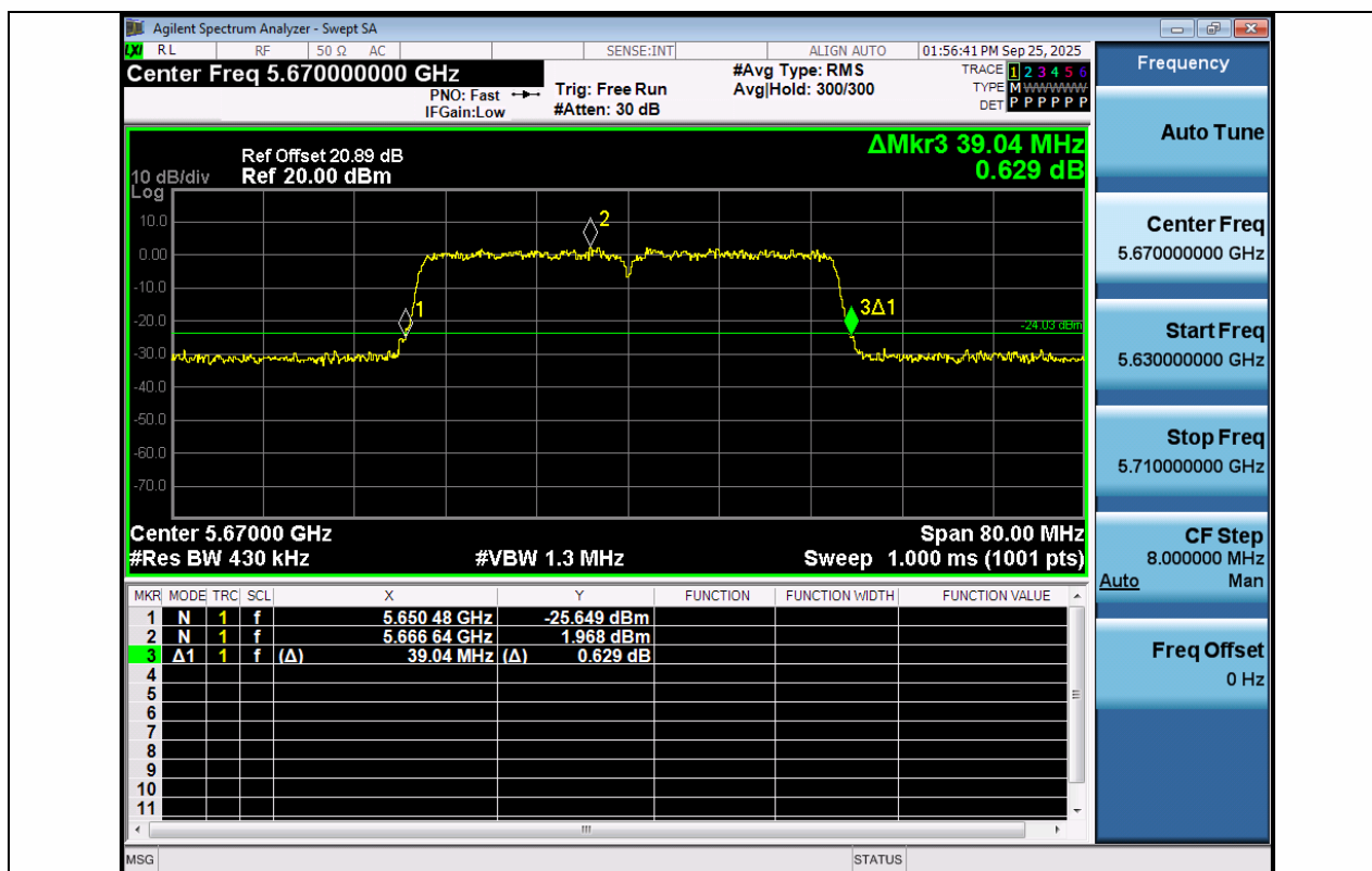
11AC40MIMO-Ant1-5670
