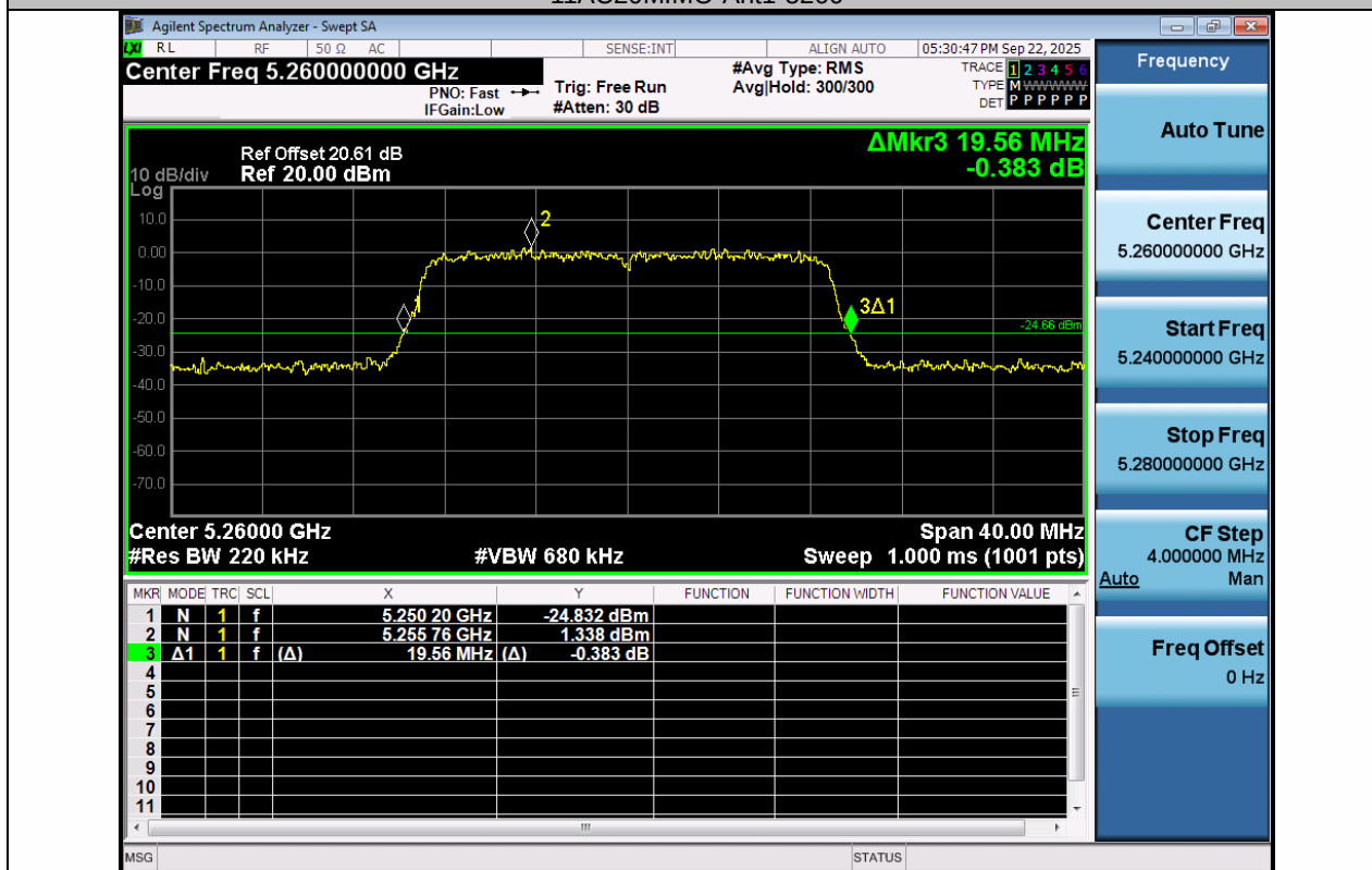
11AC20MIMO-Ant2-5260
