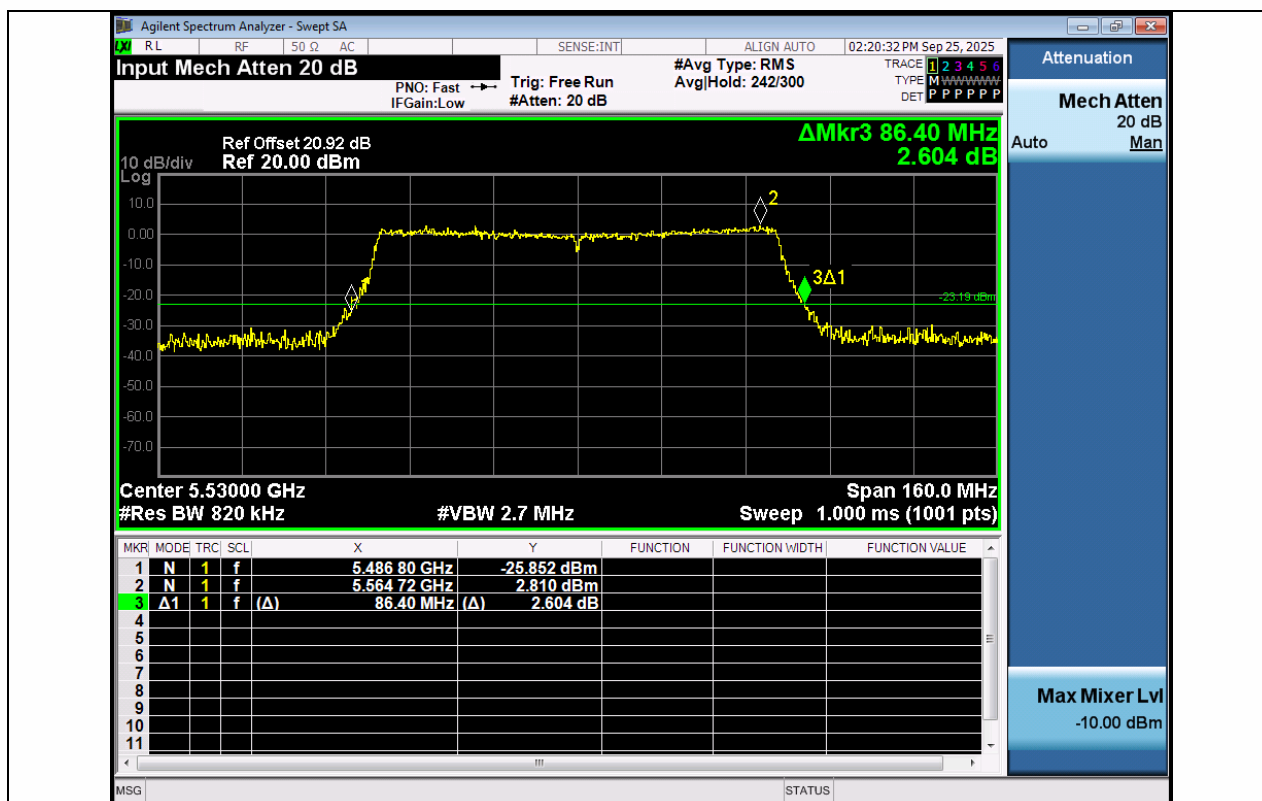
11AC80MIMO-Ant1-5530
