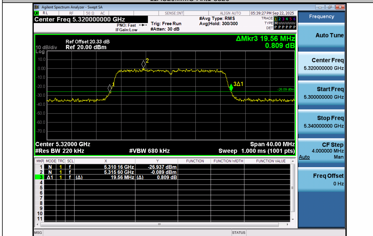
11AC20MIMO-Ant2-5320
