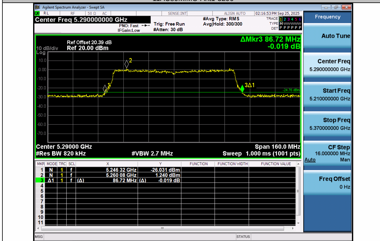
11AC80MIMO-Ant2-5290
