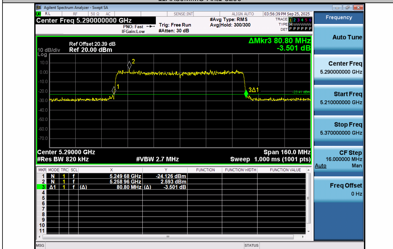
11AX80MIMO-Ant2-5290
