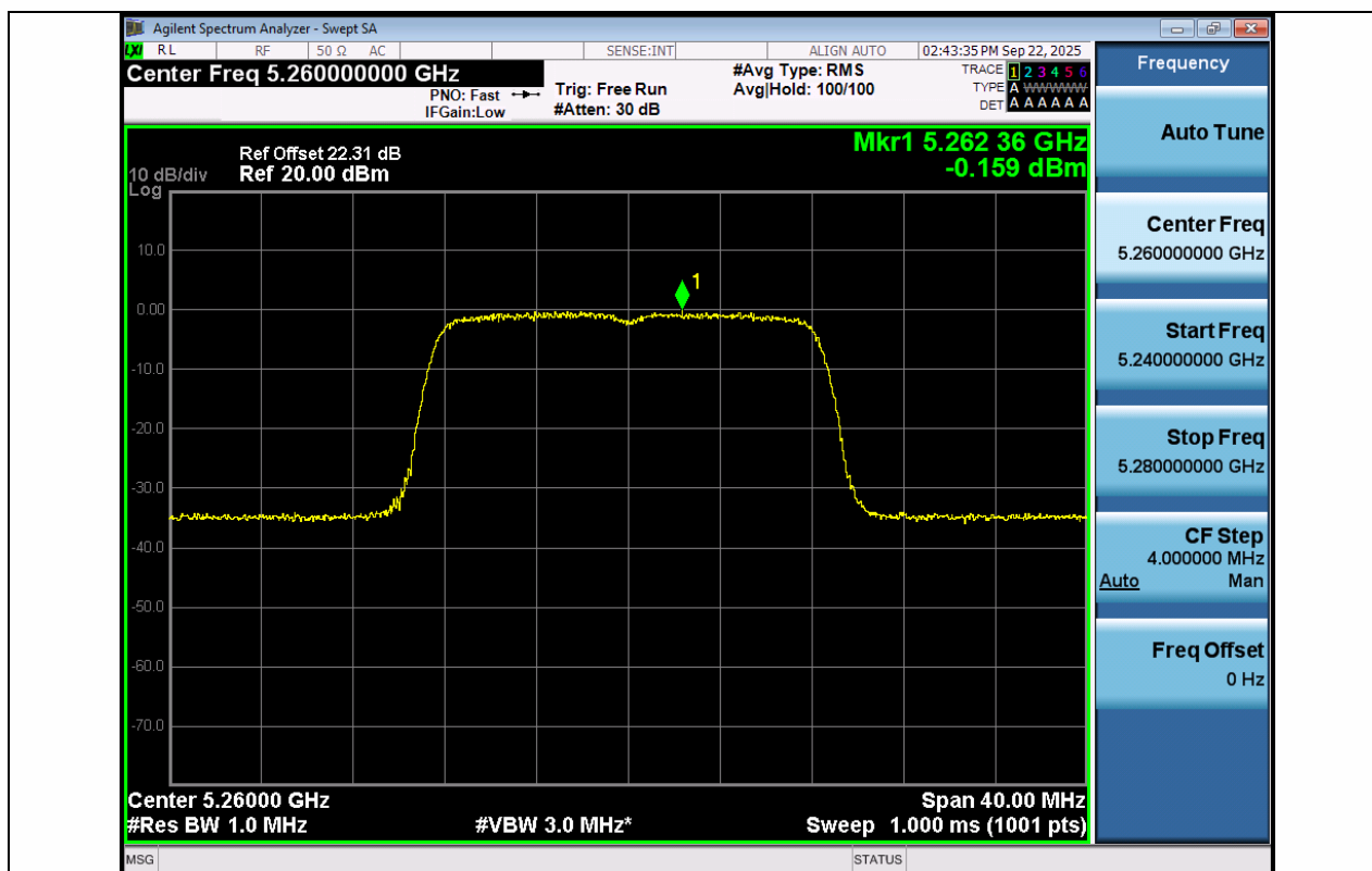
11A-Ant1-5260-PASS
