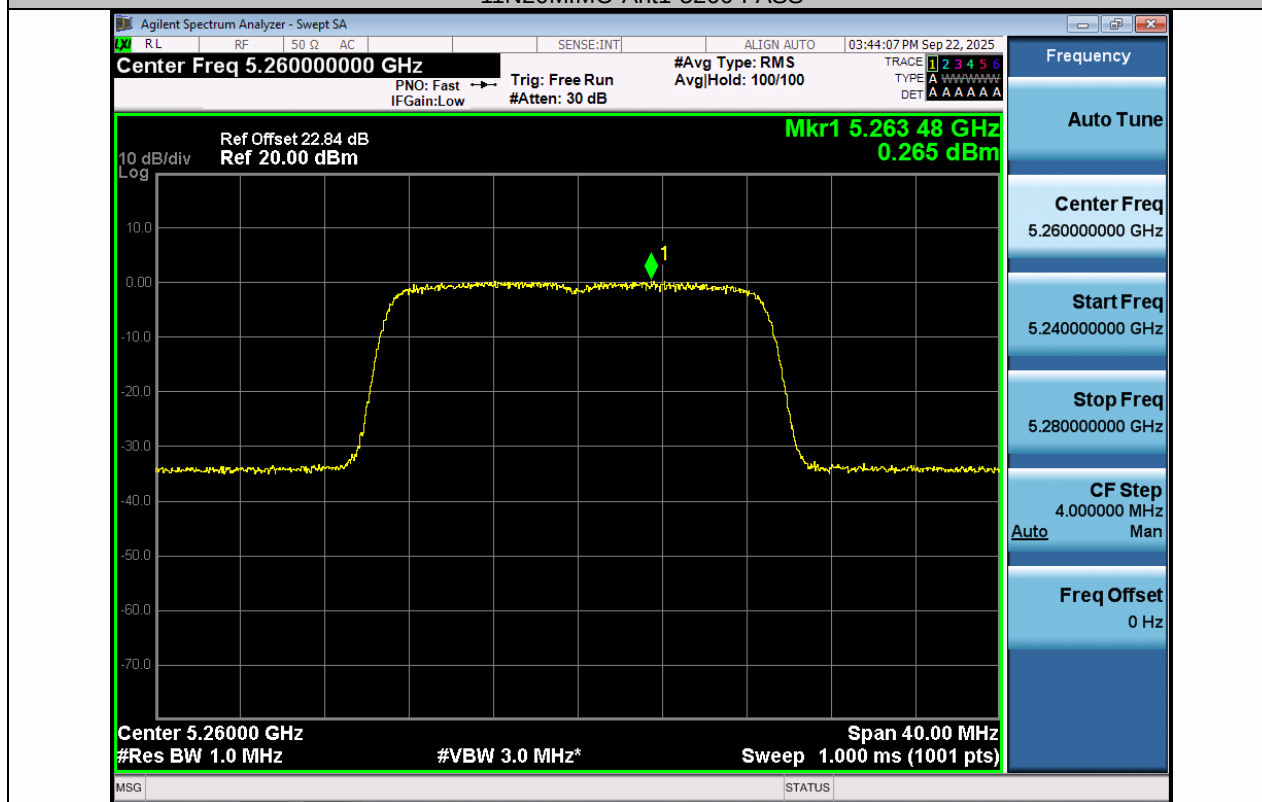
11N20MIMO-Ant2-5260-PASS
