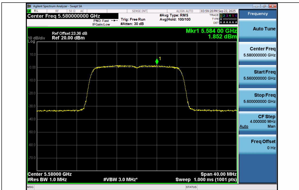
11N20MIMO-Ant1-5580-PASS
