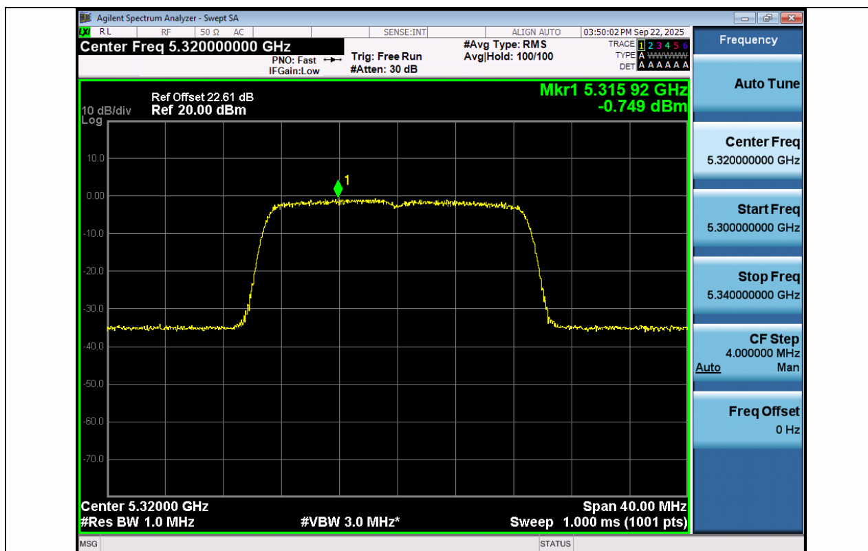
11N20MIMO-Ant1-5320-PASS
