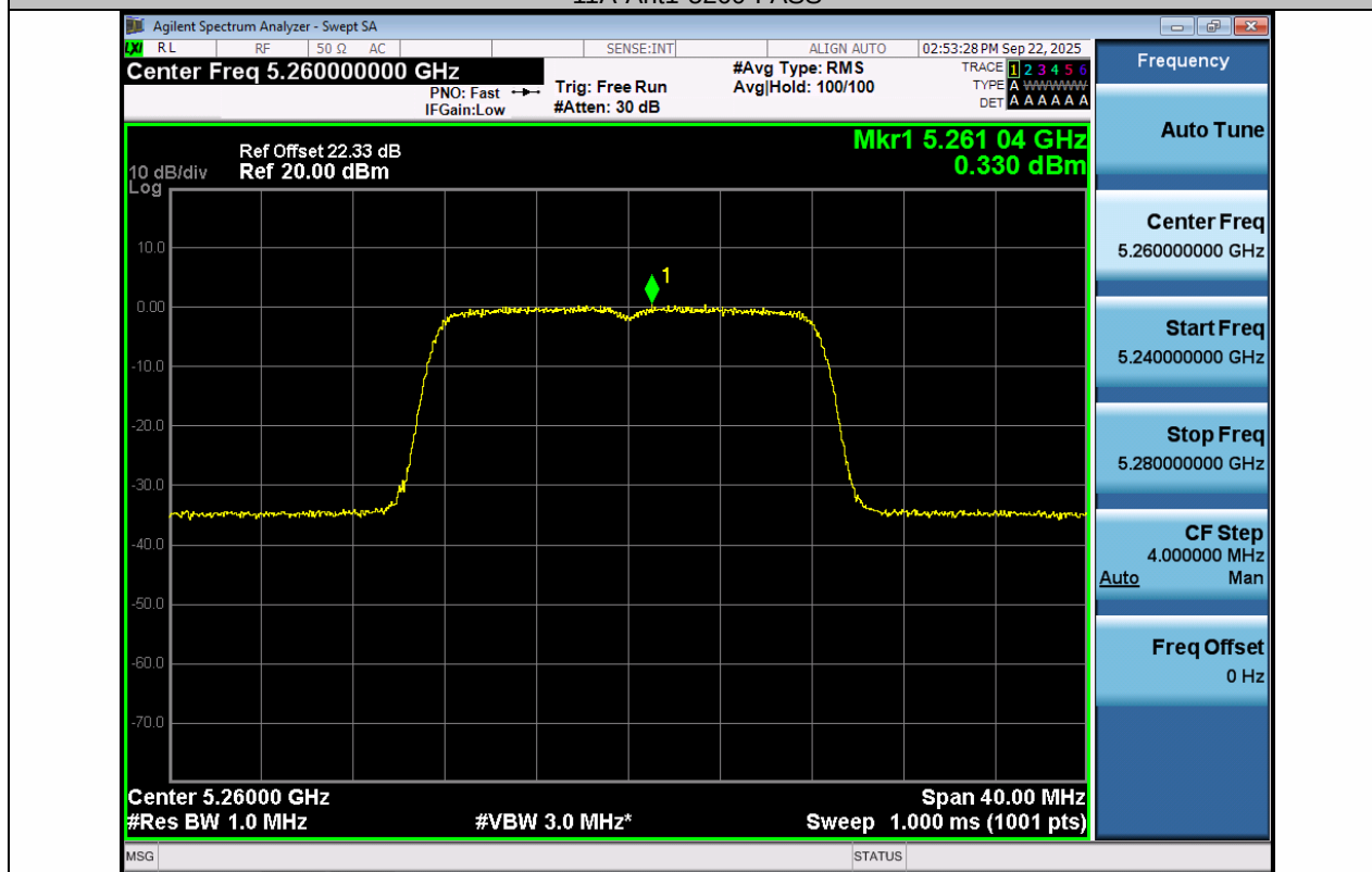
11A-Ant2-5260-PASS
