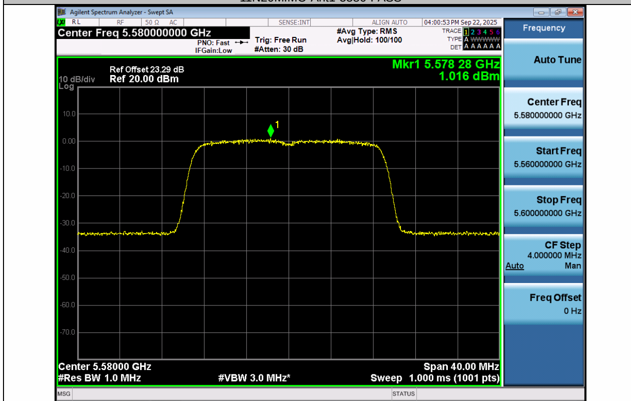
11N20MIMO-Ant2-5580-PASS
