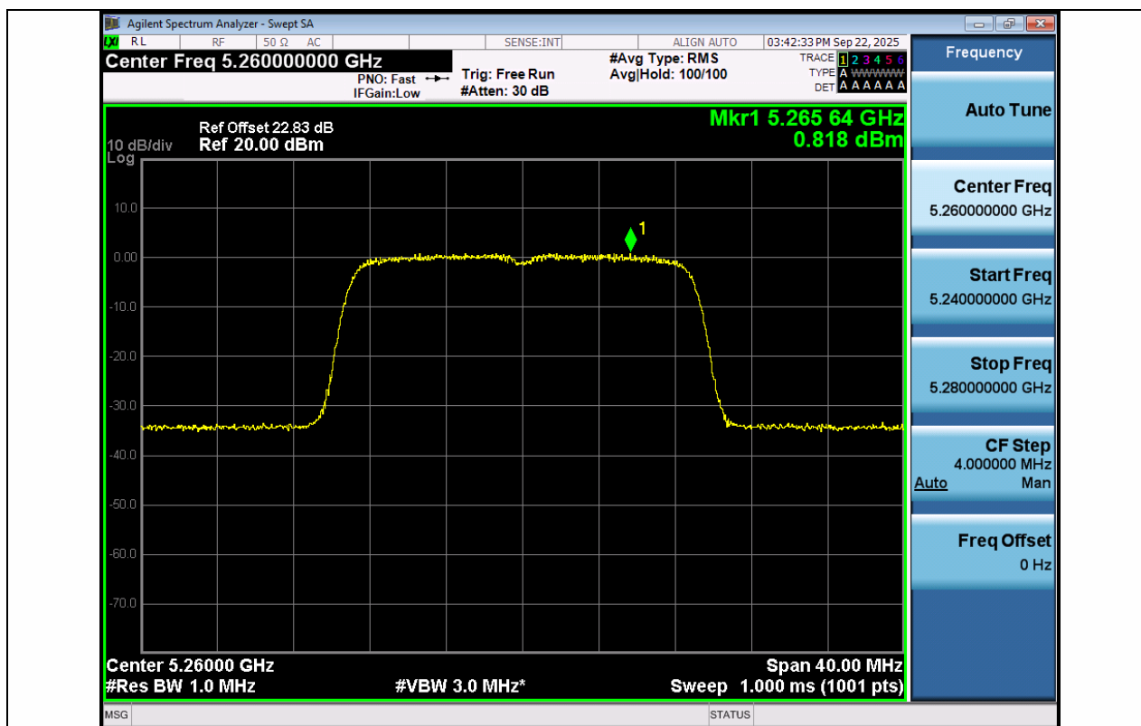
11N20MIMO-Ant1-5260-PASS
