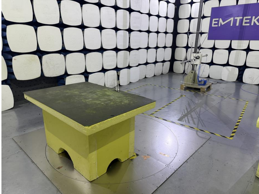
Photos of Radiation Emission Measurement Spurious Emission Test Setup (Below 1GHz)
