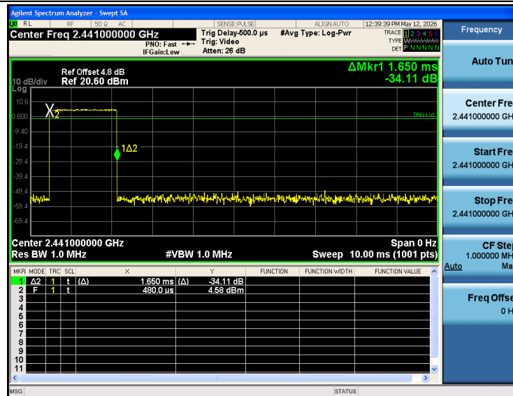
\pi/4 -DQPSK_2DH5_2441
