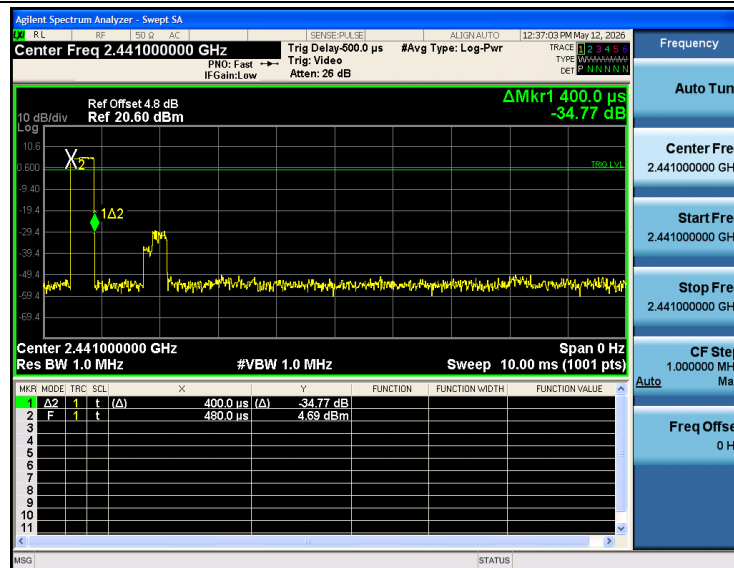
\pi/4 -DQPSK_2DH3_2441
