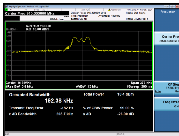
99% Bandwidth
