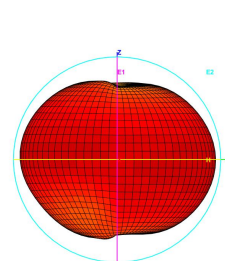
Total_3D_E2_2.45GHz
