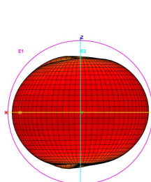
Total_3D_E1_2.4GHz
