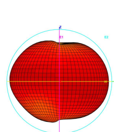
Total_3D_E2_2.4GHz
