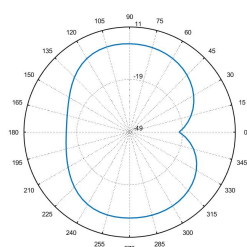
Total_Polar_E1_5.15GHz
