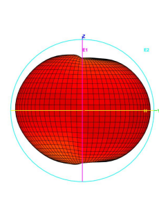
Total_3D_E2_2.5GHz
