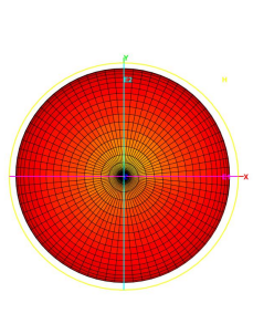
Total_3D_H_2.5GHz
