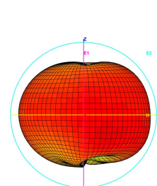
Total_3D_E2_5.15GHz
