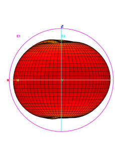
Total_3D_E1_2.5GHz
