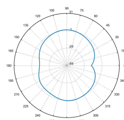
Total_Polar_E2_2.45GHz
