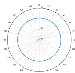
Total_Polar_H_2.45GHz
