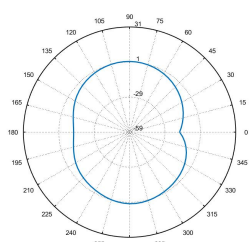
Total_Polar_E1_2.45GHz
