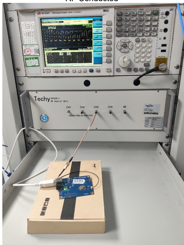
RF Conducted
