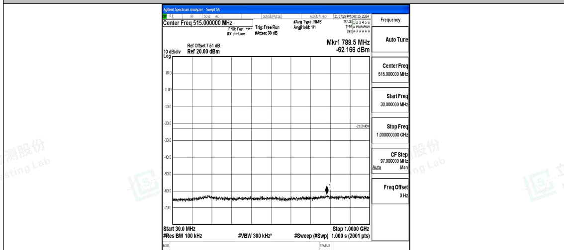
Band4_15MHz_QPSK_2025_1RB#0_30~1000_30~1000
