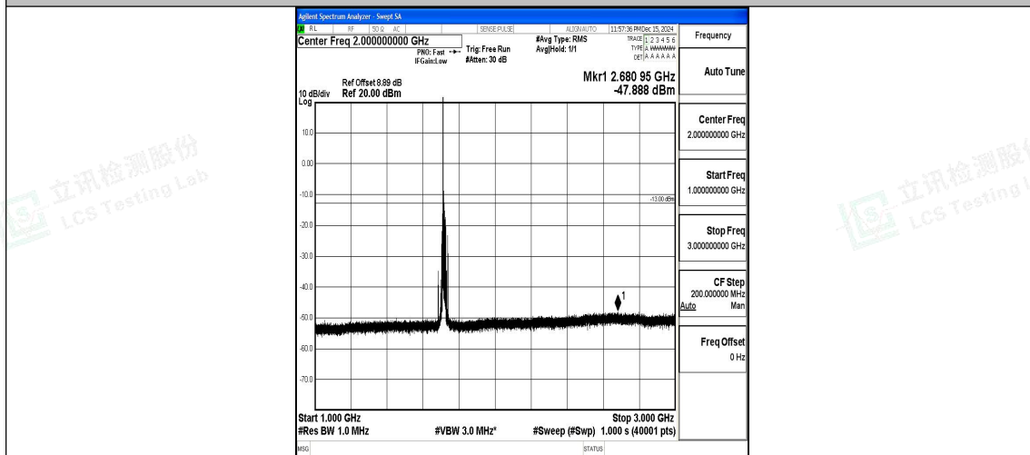
Band4_15MHz_QPSK_2025_1RB#0_1000~3000_1000~3000
