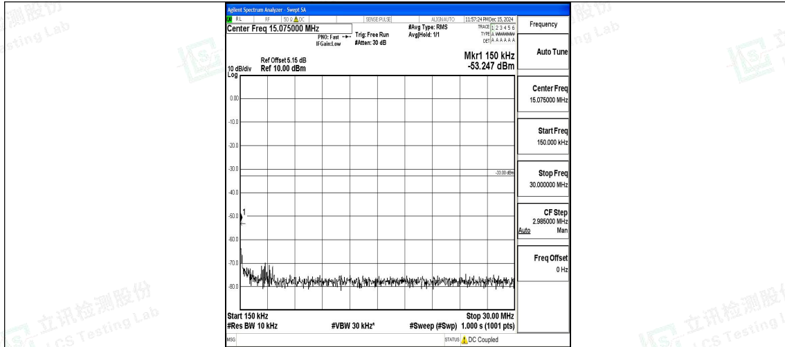
Band4_15MHz_QPSK_2025_1RB#0_0.15~30_0.15~30
