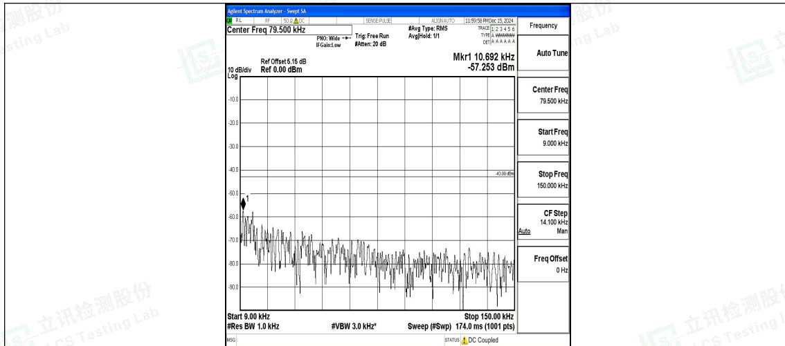
Band4_15MHz_16QAM_20325_1RB#0_0.009~0.15_0.009~0.15
