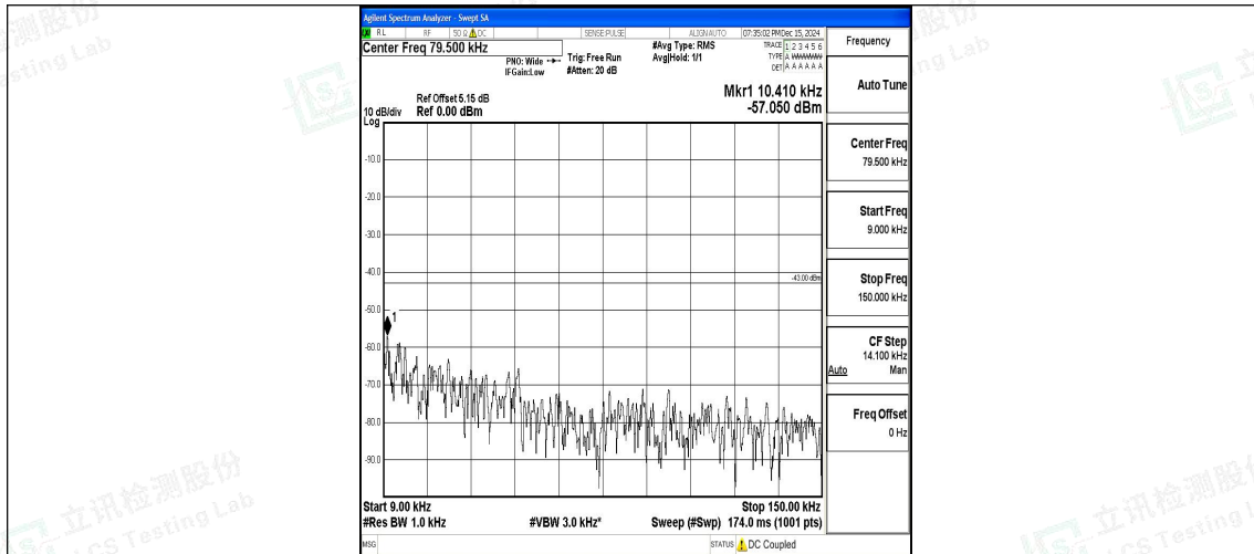
Band4_20MHz_16QAM_20050_1RB#0_0.009~0.15_0.009~0.15
