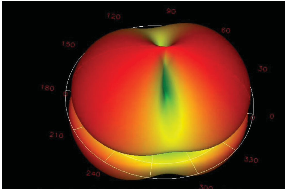
Radiation Diagram @2.441GHZ
