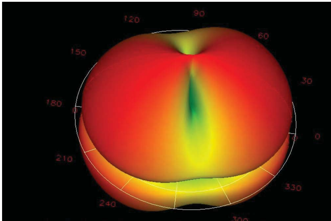
Radiation Diagram @2.480GHZ
