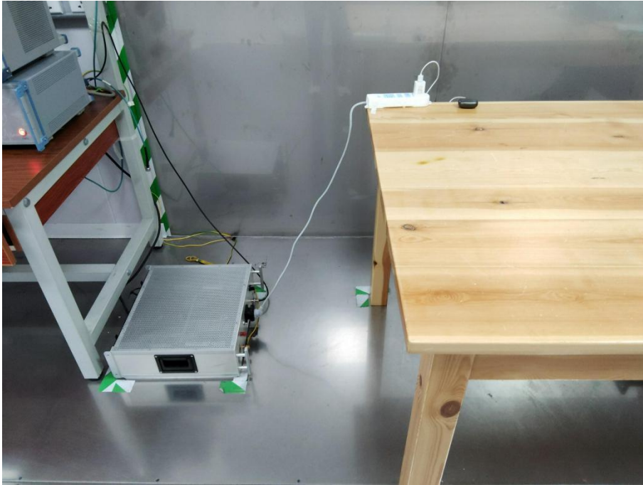
Radiated band edge emission Radiated Spurious Emission (Above 1GHz) (Right earphone)
