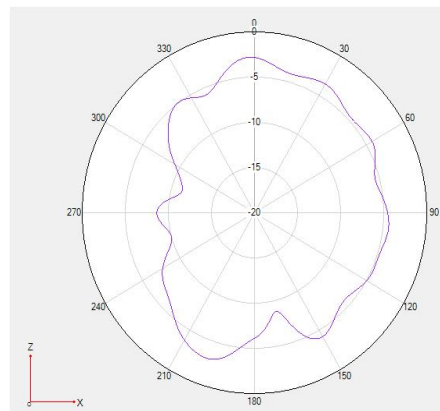
Phi 0 freq=2450MHz
