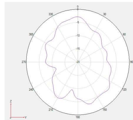
Phi 90 freq=2450MHz
