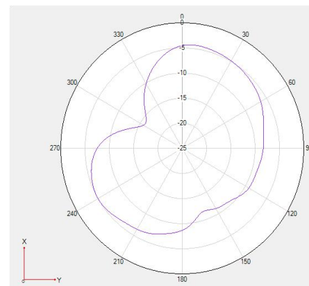
Theta 90 freq=2450MHz
