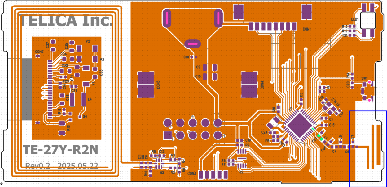
Horizontal Meandering-Line Antenna (Pattern)
