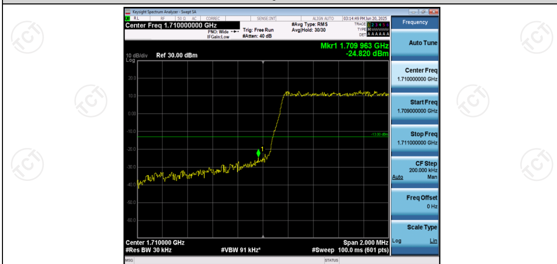
Band66-1.4MHz-16QAM-131979-6RB#0
