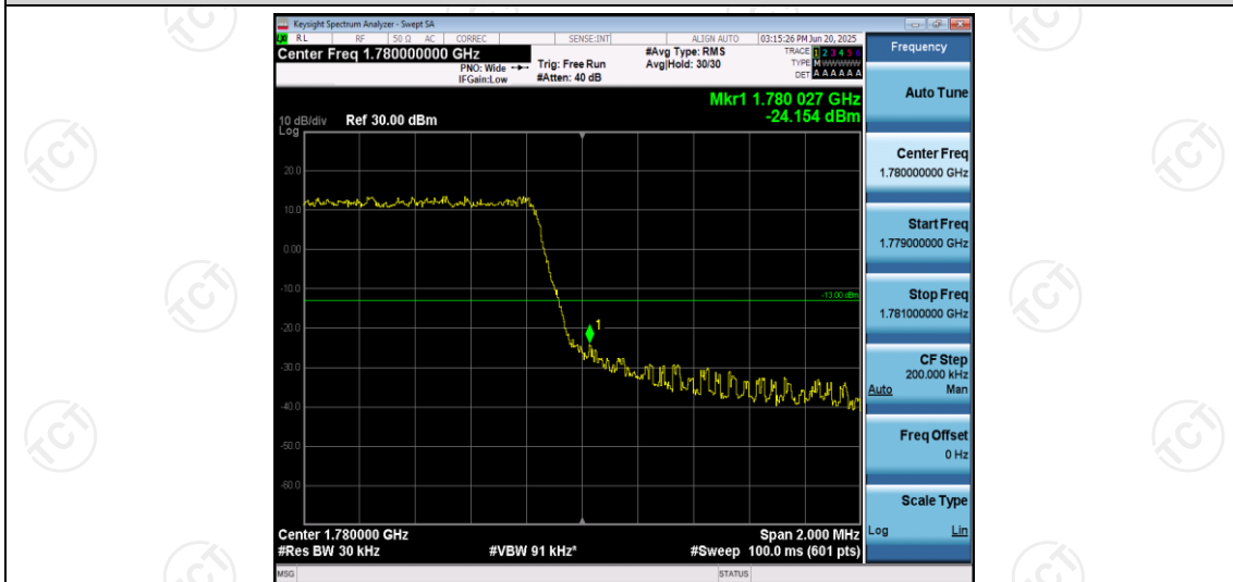
Band66-1.4MHz-QPSK-132665-6RB#0
