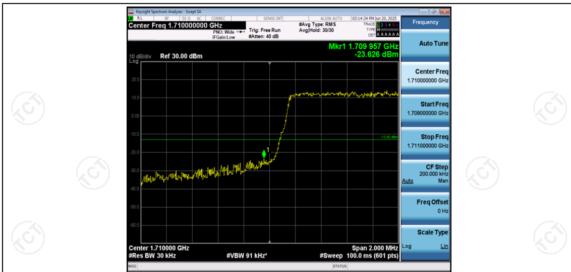
Band66-1.4MHz-QPSK-131979-6RB#0
