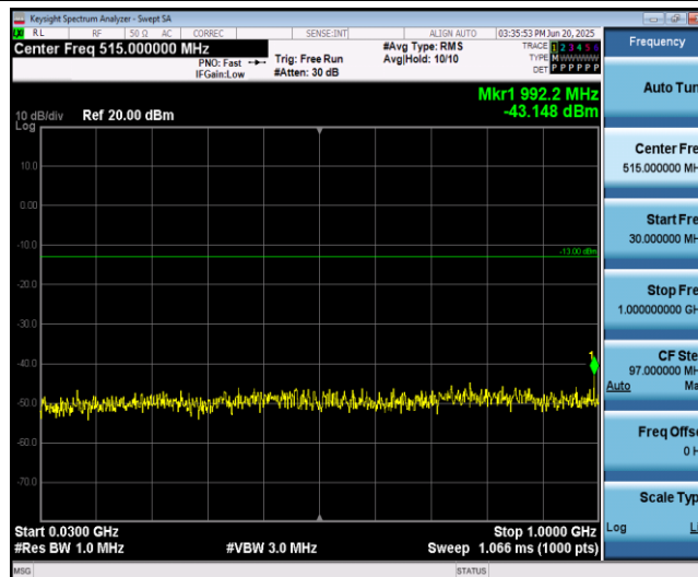
Band66-5MHz-16QAM-132322-1RB#0-Range1:30~1000MHz
