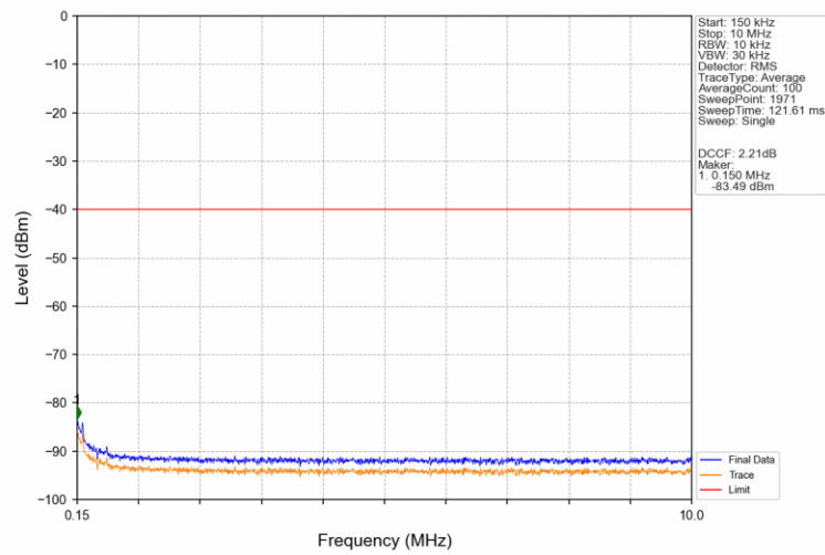
Band40b_5MHz_16QAM_LCH_2352.5MHz_RB_1_0_NTNV
