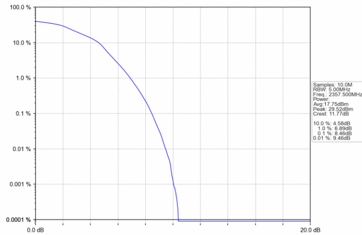
Band40b_5MHz_16QAM_HCH_2357.5MHz_RB_25_0_NTNV
