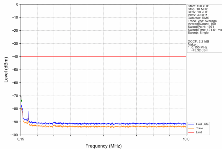
Band40b_5MHz_16QAM_MCH_2355MHz_RB_1_0_NTNV
