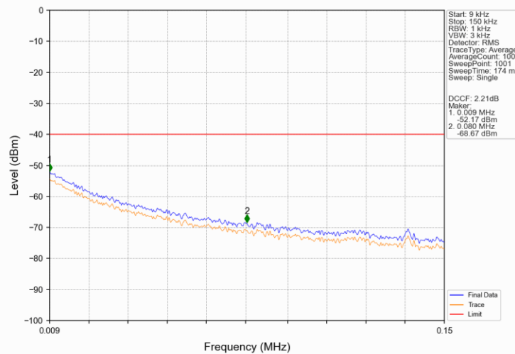
Band40b_5MHz_16QAM_HCH_2357.5MHz_RB_1_0_NTNV
