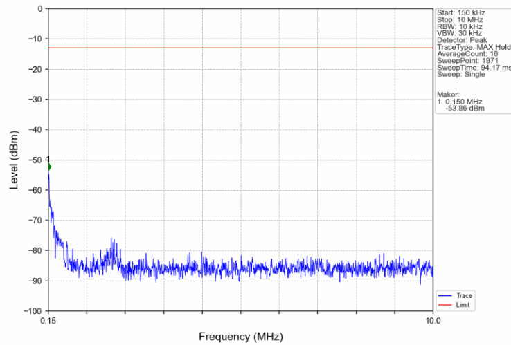
Band5_1.4MHz_16QAM_LCH_824.7MHz_RB_1_0_NTNV
