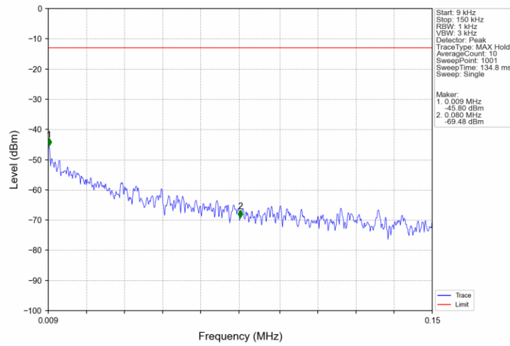
Band5_1.4MHz_QPSK_HCH_848.3MHz_RB_1_0_NTNV
