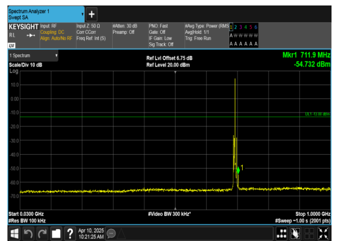
Band12-3MHz-QPSK-23025-1RB#14-30~1000-PASS
