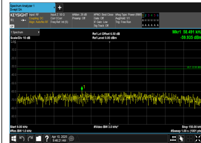
Band12-1.4MHz-QPSK-23173-1RB#0-0.009~0.15-PASS
