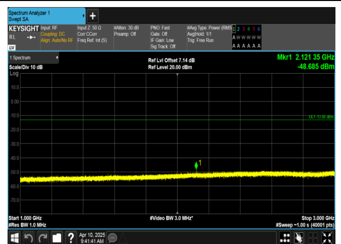
Band12-1.4MHz-16QAM-23095-1RB#0-1000~3000-PASS
