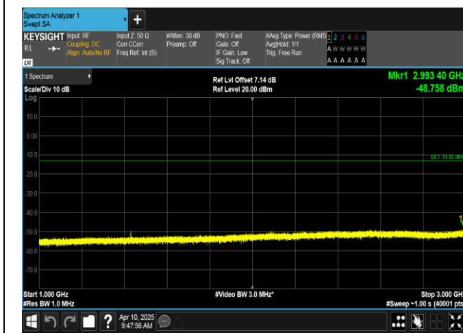
Band12-1.4MHz-16QAM-23173-1RB#0-1000~3000-PASS
