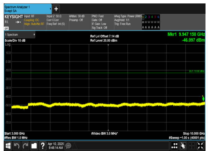
Band12-1.4MHz-16QAM-23173-1RB#0-3000~10000-PASS
