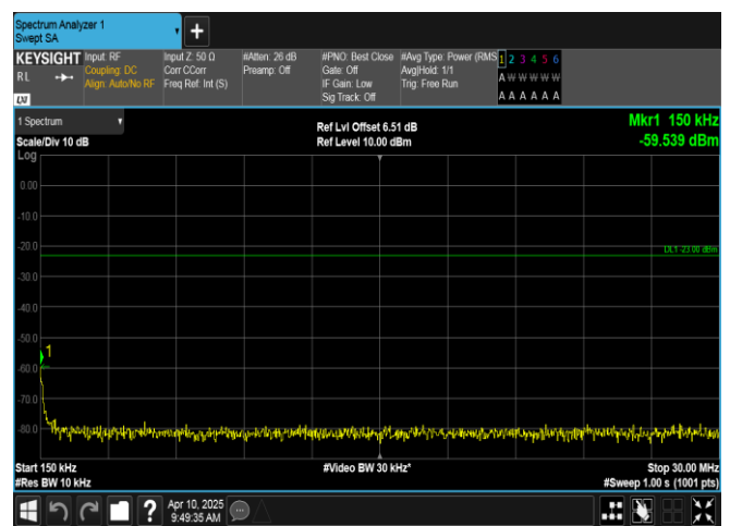
Band12-1.4MHz-16QAM-23173-1RB#5-0.15~30-PASS
