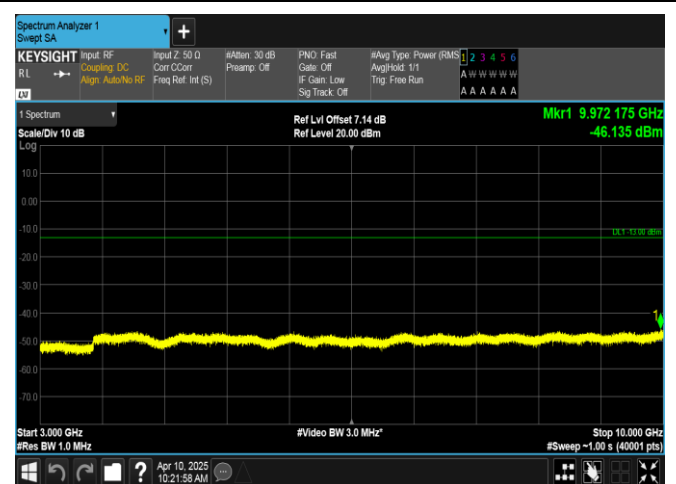
Band12-3MHz-QPSK-23025-1RB#14-3000~10000-PASS
