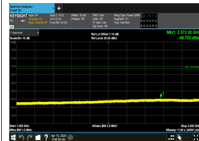
Band12-1.4MHz-QPSK-23173-1RB#5-1000~3000-PASS
