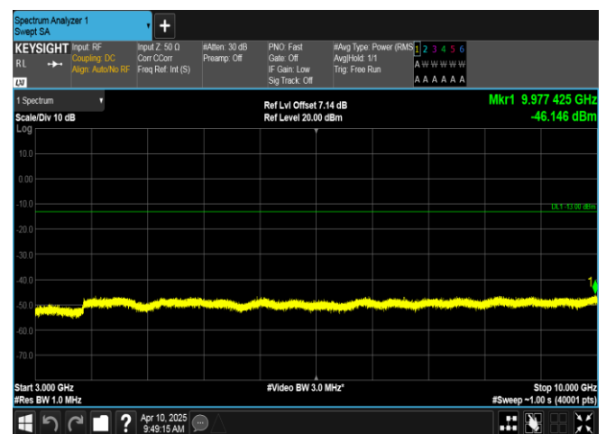
Band12-1.4MHz-QPSK-23173-1RB#5-3000~10000-PASS
