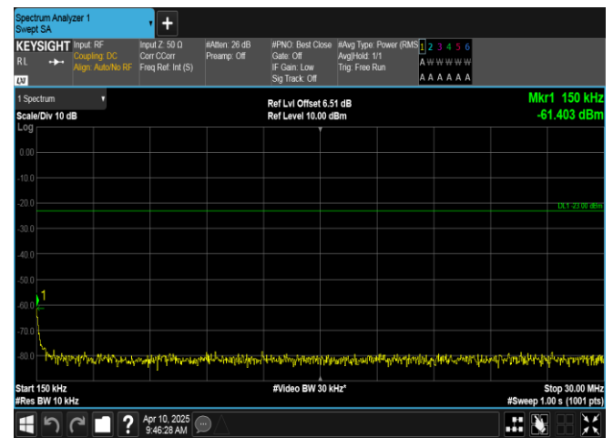
Band12-1.4MHz-QPSK-23173-1RB#0-0.15~30-PASS
