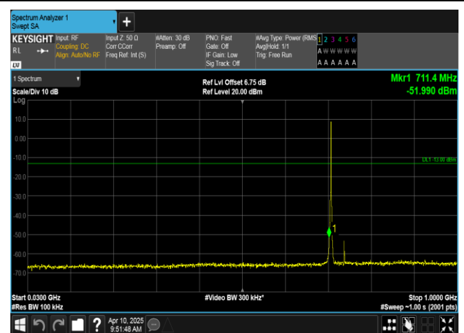
Band12-1.4MHz-16QAM-23173-6RB#0-30~1000-PASS
