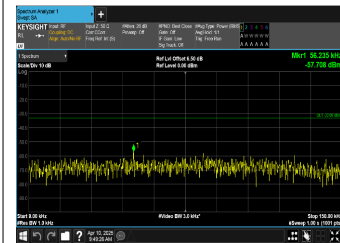
Band12-1.4MHz-16QAM-23173-1RB#5-0.009~0.15-PASS
