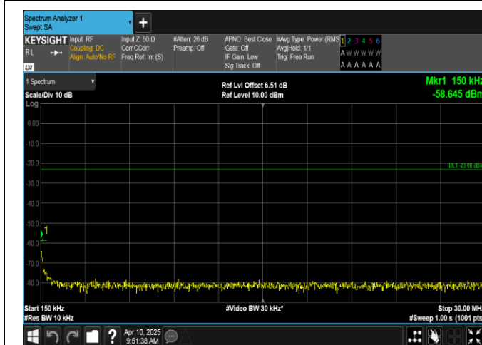
Band12-1.4MHz-16QAM-23173-6RB#0-0.15~30-PASS
