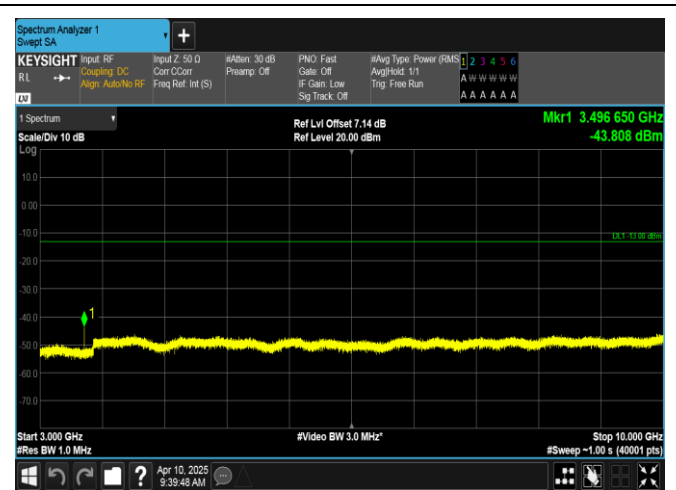
Band12-1.4MHz-16QAM-23017-6RB#0-3000~10000-PASS
