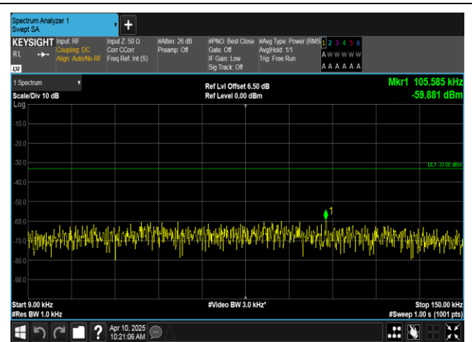
Band12-3MHz-QPSK-23025-1RB#14-0.009~0.15-PASS
