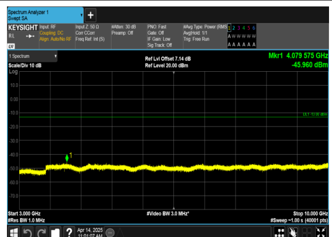
Band13-10MHz-QPSK-23230-1RB#49-3000~10000-PASS
