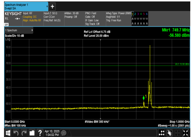
Band13-5MHz-16QAM-23230-1RB#24-30~1000-PASS
