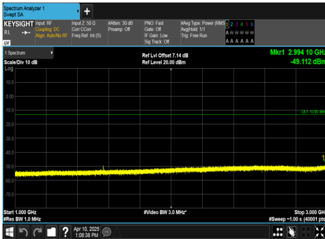
Band13-5MHz-16QAM-23255-1RB#0-1000~3000-PASS
