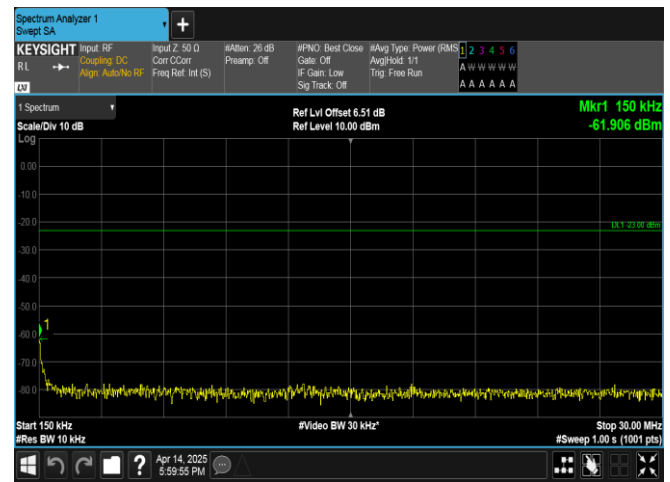
Band13-10MHz-QPSK-23230-50RB#0-0.15~30-PASS
