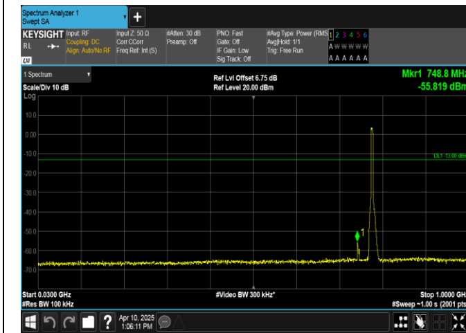
Band13-5MHz-16QAM-23230-25RB#0-30~1000-PASS
