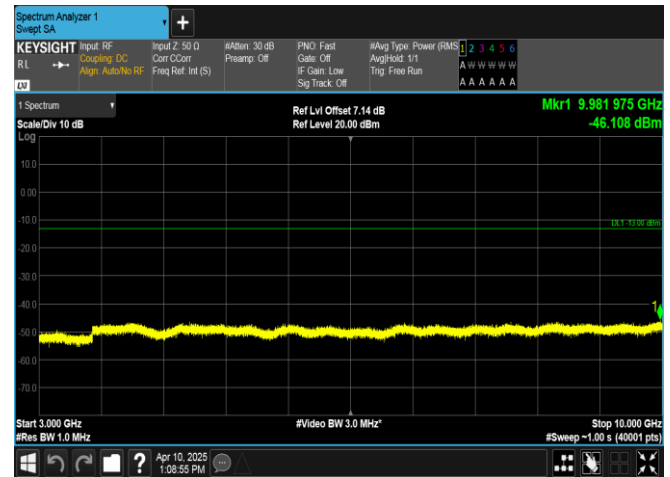
Band13-5MHz-16QAM-23255-1RB#0-3000~10000-PASS
