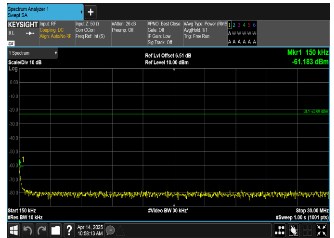
Band13-10MHz-QPSK-23230-1RB#0-0.15~30-PASS
