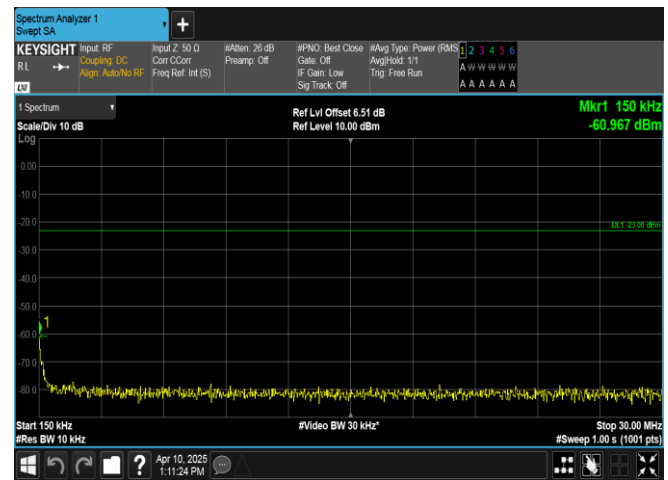
Band13-5MHz-QPSK-23255-25RB#0-0.15~30-PASS
