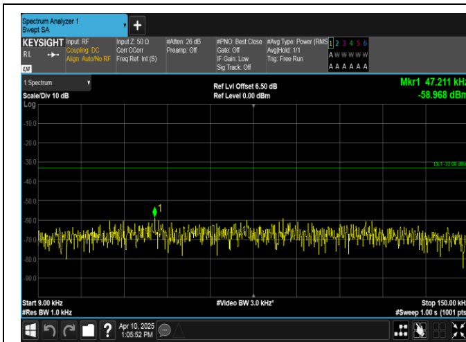
Band13-5MHz-16QAM-23230-25RB#0-0.009~0.15-PASS
