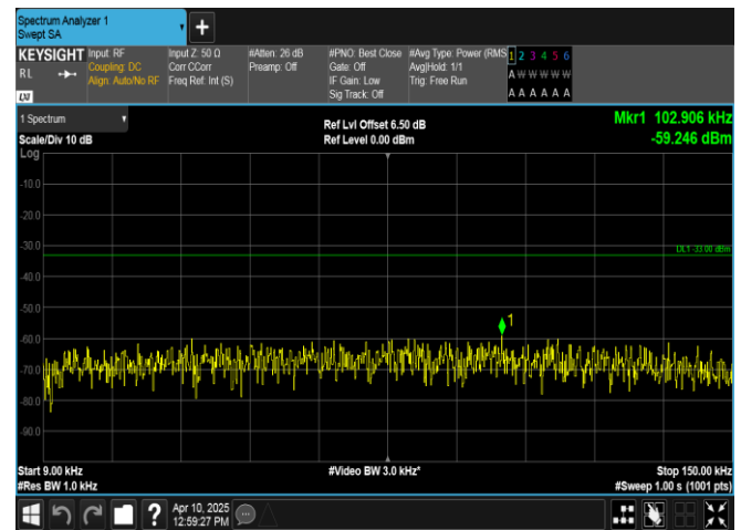
Band13-5MHz-16QAM-23205-25RB#0-0.009~0.15-PASS
