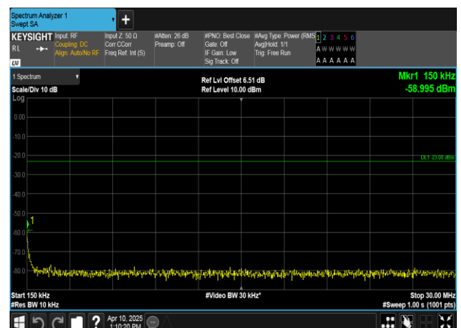
Band13-5MHz-16QAM-23255-1RB#24-0.15~30-PASS
