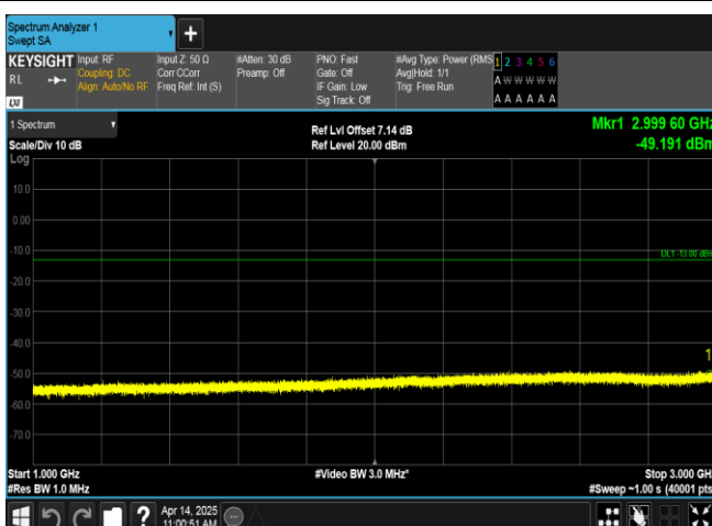
Band13-10MHz-QPSK-23230-1RB#49-1000~3000-PASS
