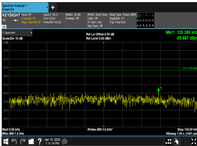
Band13-5MHz-QPSK-23255-25RB#0-0.009~0.15-PASS
