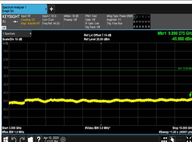
Band13-5MHz-QPSK-23255-25RB#0-3000~10000-PASS
