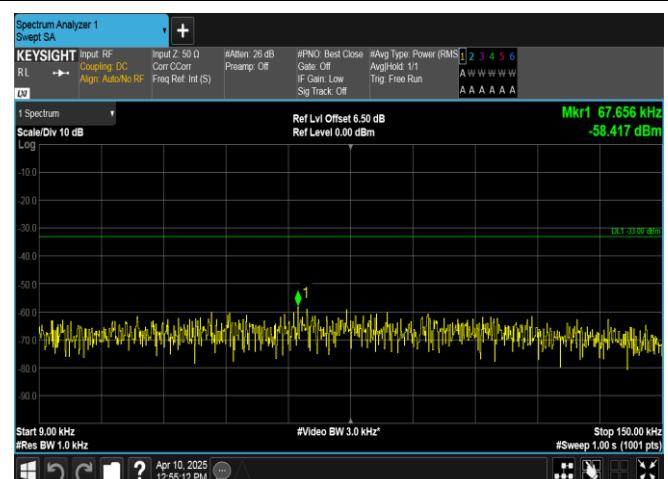
Band13-5MHz-16QAM-23205-1RB#0-0.009~0.15-PASS
