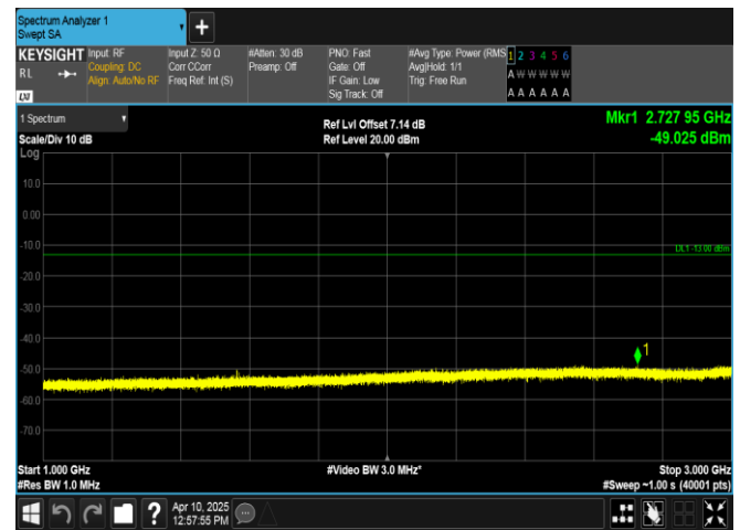
Band13-5MHz-16QAM-23205-1RB#24-1000~3000-PASS
