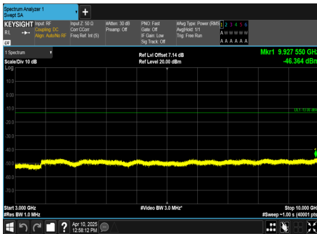
Band13-5MHz-16QAM-23205-1RB#24-3000~10000-PASS
