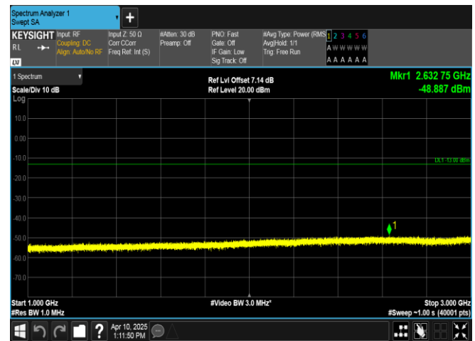
Band13-5MHz-QPSK-23255-25RB#0-1000~3000-PASS
