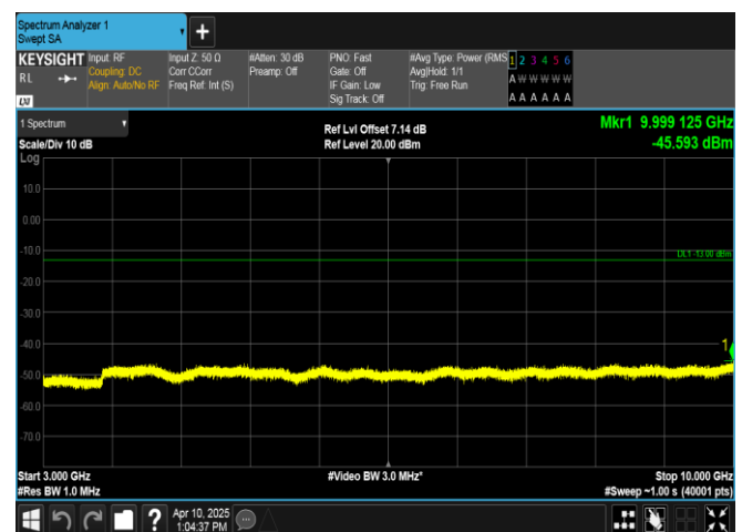
Band13-5MHz-16QAM-23230-1RB#24-3000~10000-PASS
