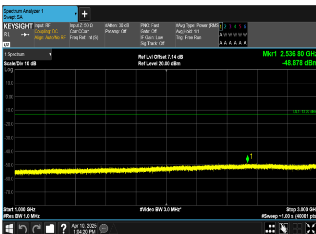
Band13-5MHz-16QAM-23230-1RB#24-1000~3000-PASS
