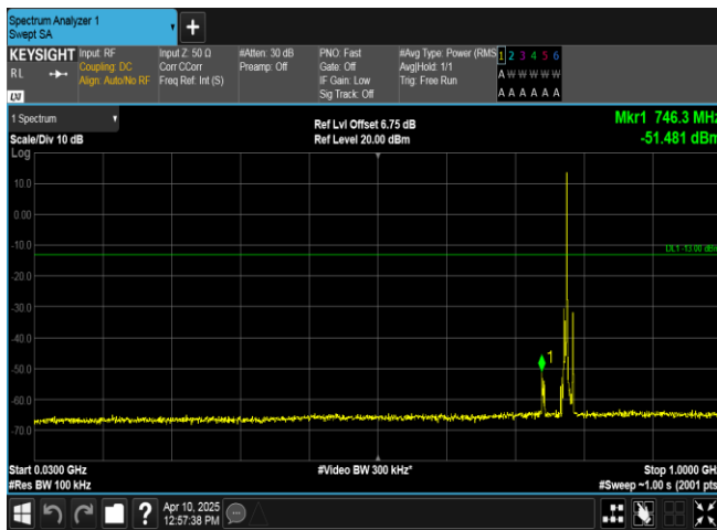
Band13-5MHz-16QAM-23205-1RB#24-30~1000-PASS
