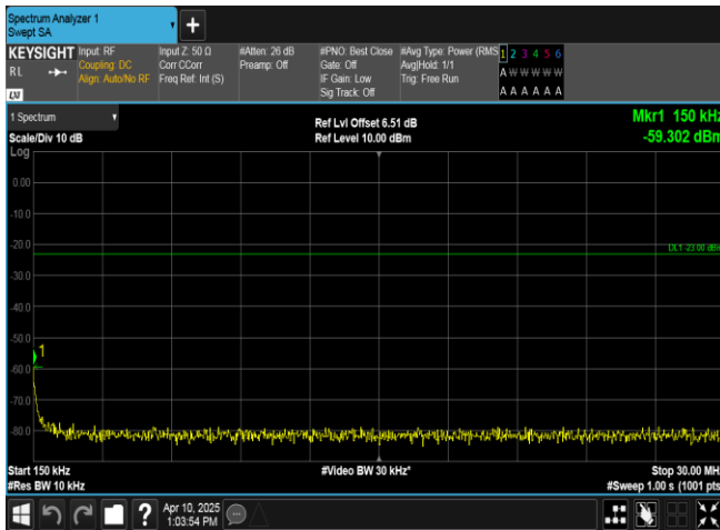
Band13-5MHz-16QAM-23230-1RB#24-0.15~30-PASS
