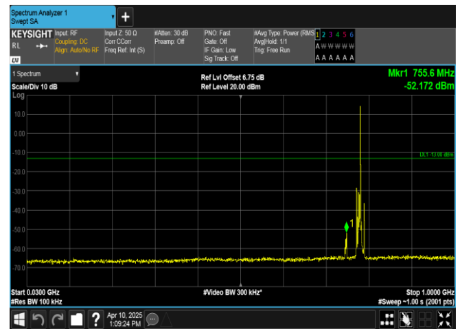
Band13-5MHz-QPSK-23255-1RB#24-30~1000-PASS
