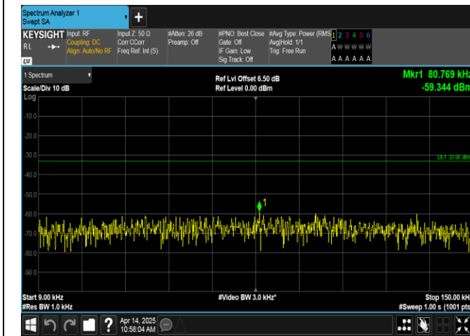
Band13-10MHz-QPSK-23230-1RB#0-0.009~0.15-PASS
