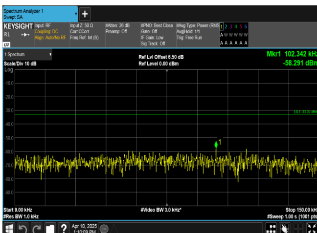
Band13-5MHz-16QAM-23255-1RB#24-0.009~0.15-PASS
