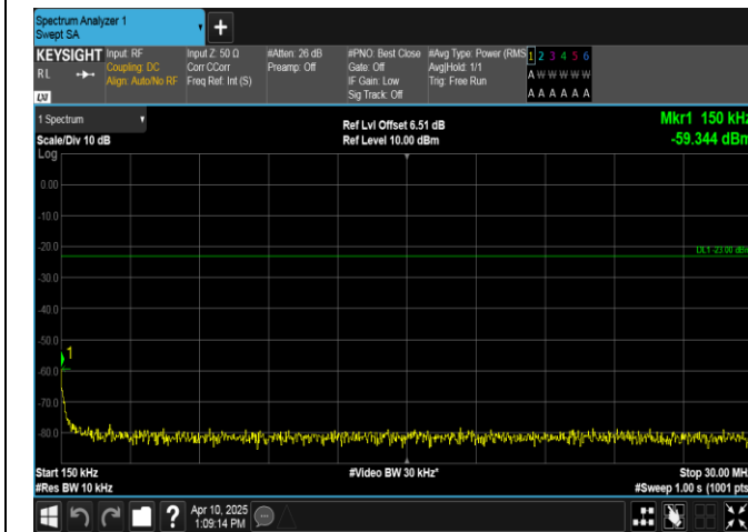
Band13-5MHz-QPSK-23255-1RB#24-0.15~30-PASS
