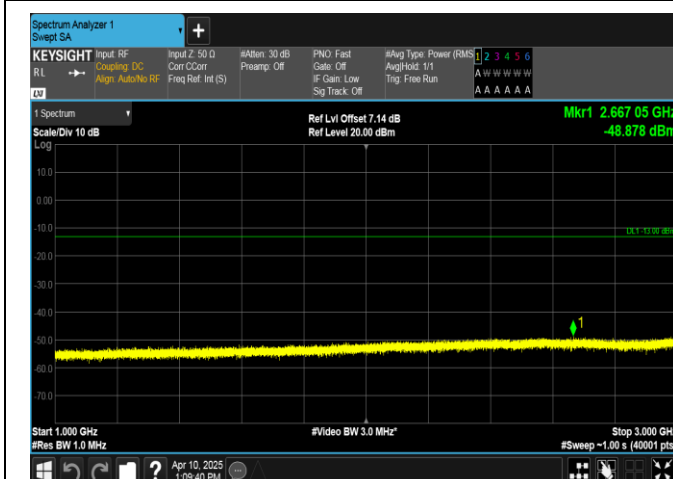
Band13-5MHz-QPSK-23255-1RB#24-1000~3000-PASS
