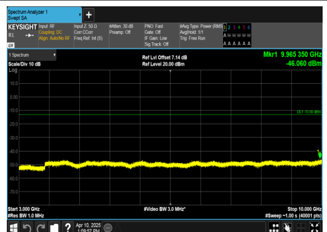
Band13-5MHz-QPSK-23255-1RB#24-3000~10000-PASS
