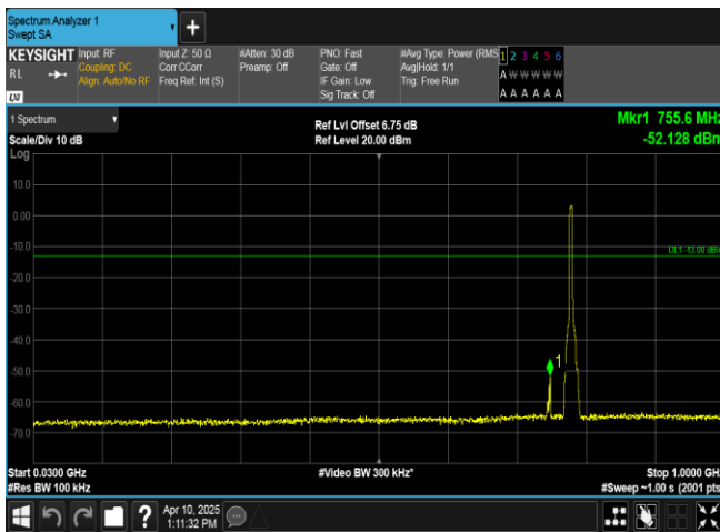
Band13-5MHz-QPSK-23255-25RB#0-30~1000-PASS
