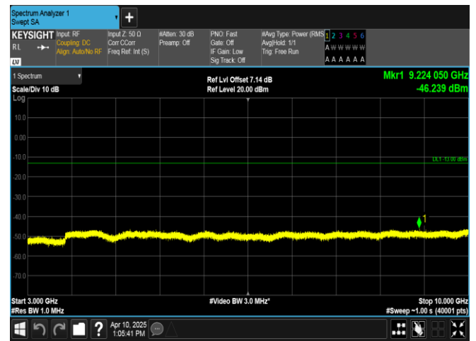
Band13-5MHz-QPSK-23230-25RB#0-3000~10000-PASS
