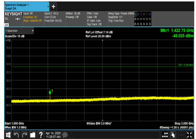
Band17-5MHz-QPSK-23825-1RB#0-1000~3000-PASS
