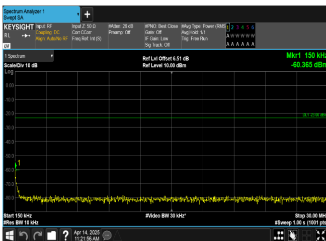
Band17-5MHz-QPSK-23790-1RB#0-0.15~30-PASS
