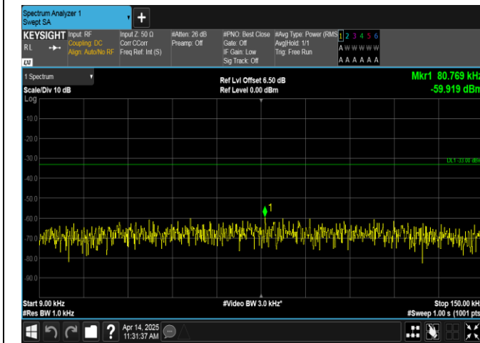
Band17-5MHz-16QAM-23825-1RB#24-0.009~0.15-PASS
