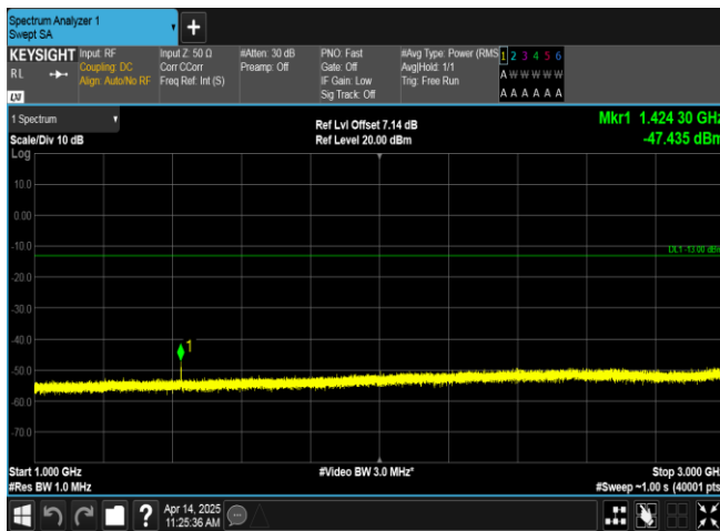
Band17-5MHz-16QAM-23790-1RB#24-1000~3000-PASS
