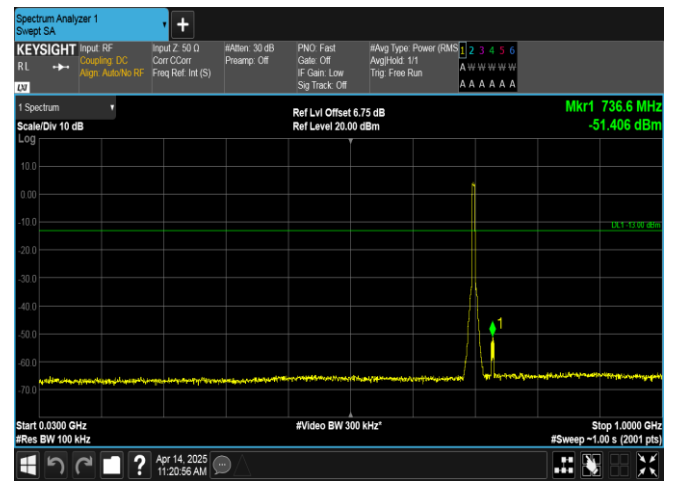
Band17-5MHz-16QAM-23755-25RB#0-30~1000-PASS
