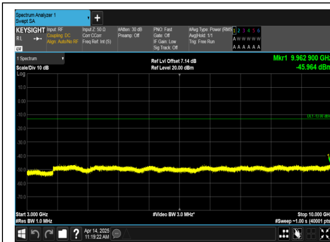
Band17-5MHz-16QAM-23755-1RB#24-3000~10000-PASS
