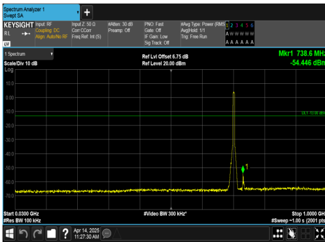
Band17-5MHz-16QAM-23790-25RB#0-30~1000-PASS
