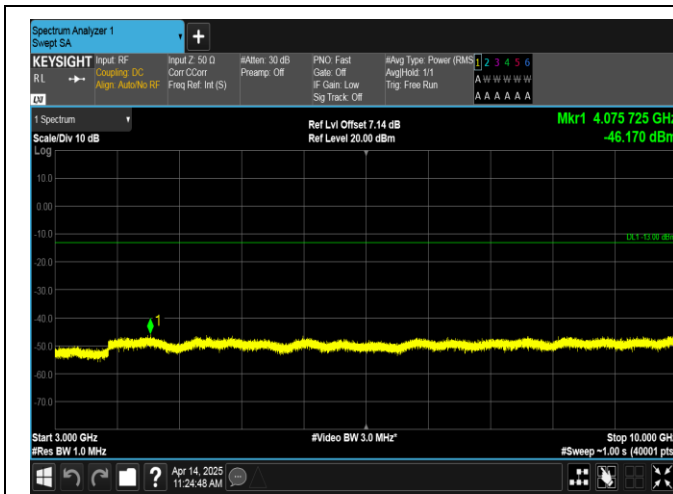
Band17-5MHz-QPSK-23790-1RB#24-3000~10000-PASS
