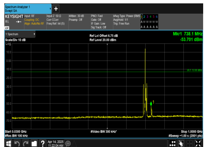
Band17-5MHz-QPSK-23790-1RB#0-30~1000-PASS
