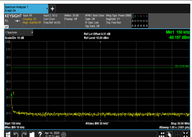
Band17-5MHz-16QAM-23790-25RB#0-0.15~30-PASS
