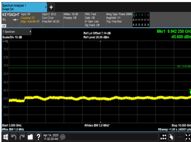
Band17-5MHz-16QAM-23825-1RB#24-3000~10000-PASS
