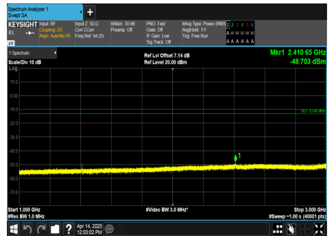
Band17-10MHz-QPSK-23780-1RB#0-1000~3000-PASS
