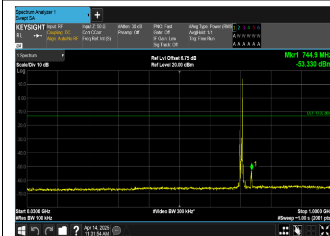
Band17-5MHz-16QAM-23825-1RB#24-30~1000-PASS
