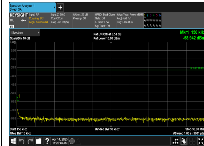
Band17-5MHz-16QAM-23755-25RB#0-0.15~30-PASS
