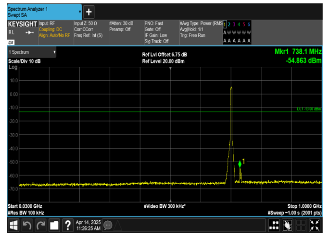
Band17-5MHz-QPSK-23790-25RB#0-30~1000-PASS
