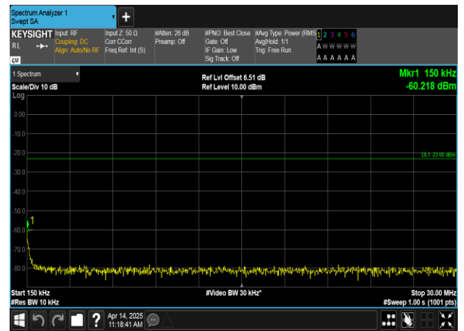
Band17-5MHz-16QAM-23755-1RB#24-0.15~30-PASS
