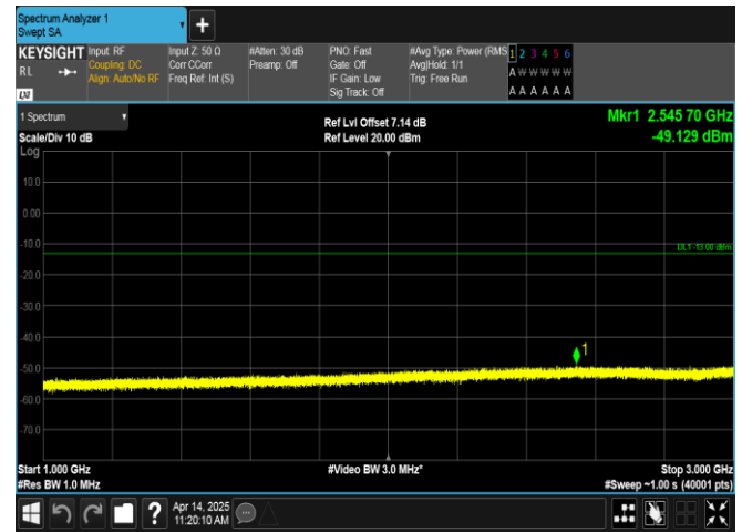
Band17-5MHz-QPSK-23755-25RB#0-1000~3000-PASS
