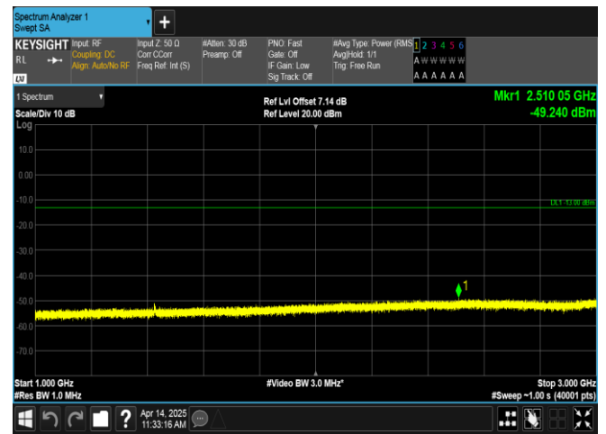
Band17-5MHz-QPSK-23825-25RB#0-1000~3000-PASS
