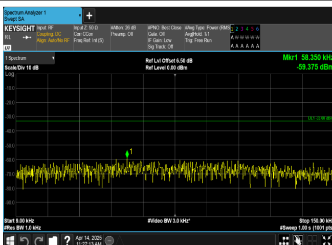
Band17-5MHz-16QAM-23790-25RB#0-0.009~0.15-PASS
