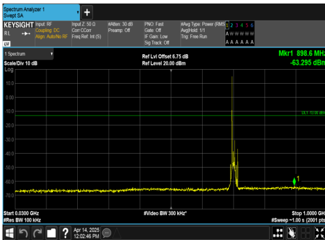
Band17-10MHz-QPSK-23780-1RB#0-30~1000-PASS
