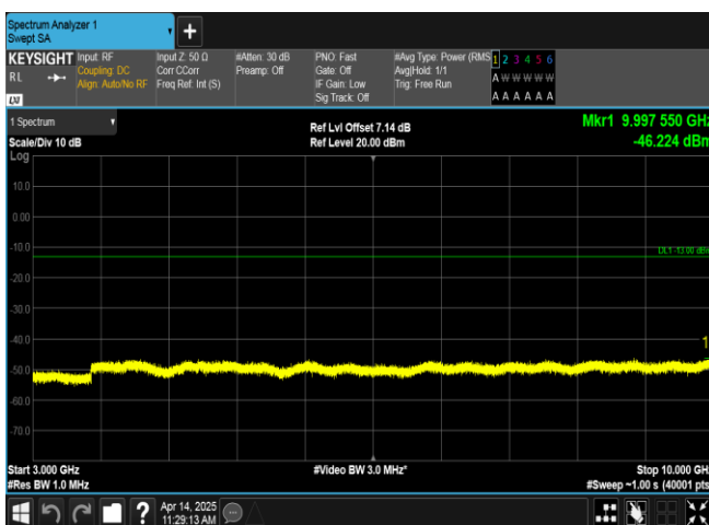
Band17-5MHz-QPSK-23825-1RB#0-3000~10000-PASS
