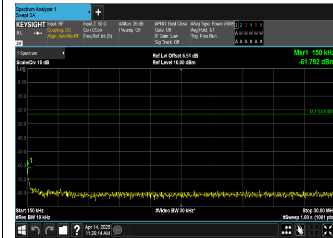
Band17-5MHz-QPSK-23790-25RB#0-0.15~30-PASS
