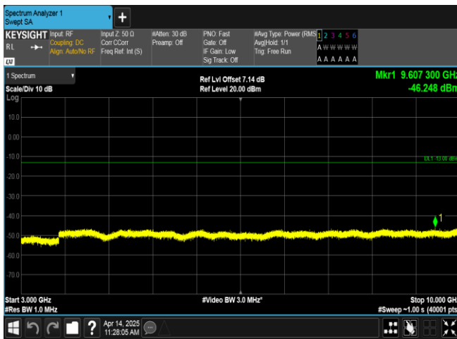
Band17-5MHz-16QAM-23790-25RB#0-3000~10000-PASS
