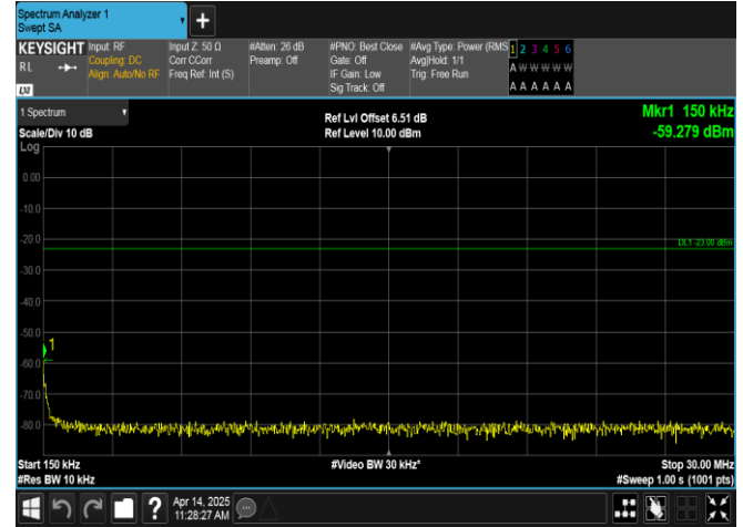
Band17-5MHz-QPSK-23825-1RB#0-0.15~30-PASS
