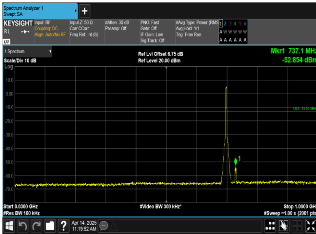
Band17-5MHz-QPSK-23755-25RB#0-30~1000-PASS
