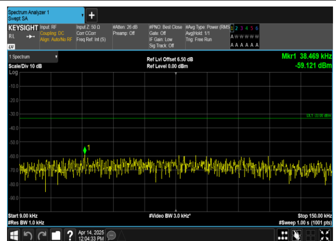
Band17-10MHz-QPSK-23780-1RB#49-0.009~0.15-PASS
