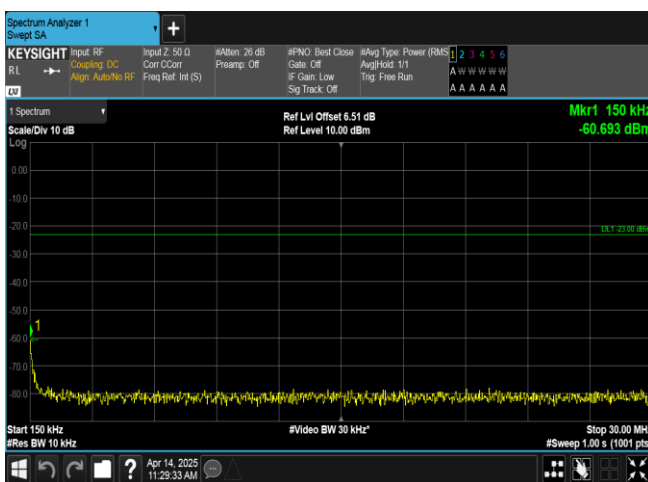
Band17-5MHz-16QAM-23825-1RB#0-0.15~30-PASS
