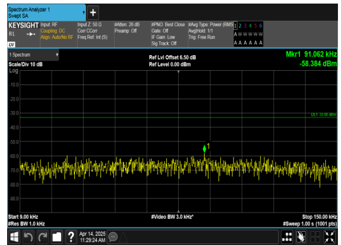
Band17-5MHz-16QAM-23825-1RB#0-0.009~0.15-PASS
