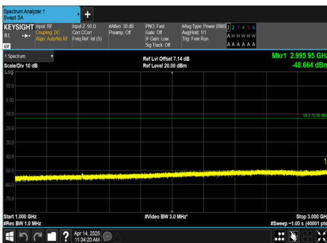
Band17-5MHz-16QAM-23825-25RB#0-1000~3000-PASS
