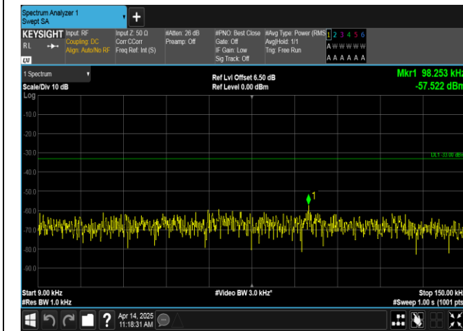
Band17-5MHz-16QAM-23755-1RB#24-0.009~0.15-PASS
