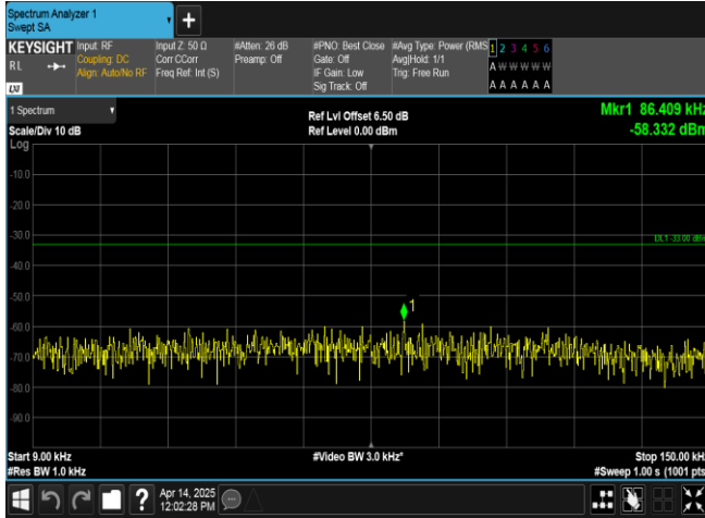
Band17-10MHz-QPSK-23780-1RB#0-0.009~0.15-PASS
