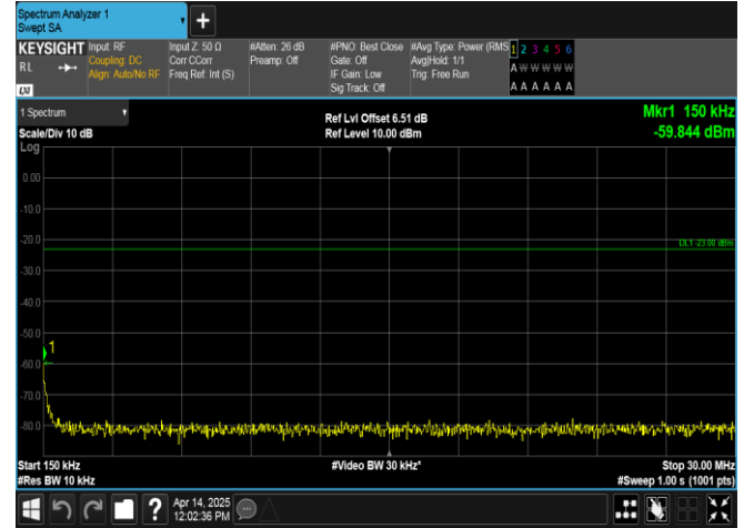
Band17-10MHz-QPSK-23780-1RB#0-0.15~30-PASS
