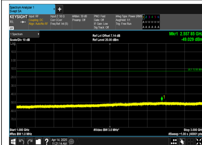
Band17-5MHz-16QAM-23755-25RB#0-1000~3000-PASS
