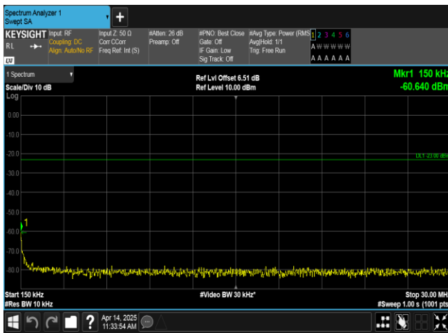
Band17-5MHz-16QAM-23825-25RB#0-0.15~30-PASS
