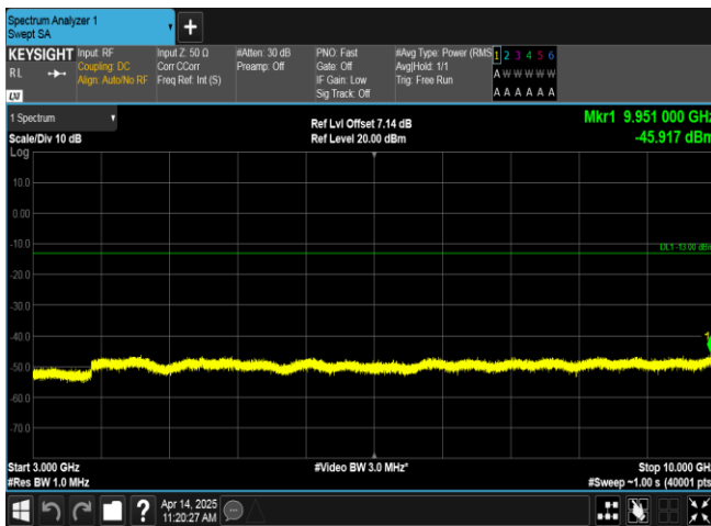
Band17-5MHz-QPSK-23755-25RB#0-3000~10000-PASS
