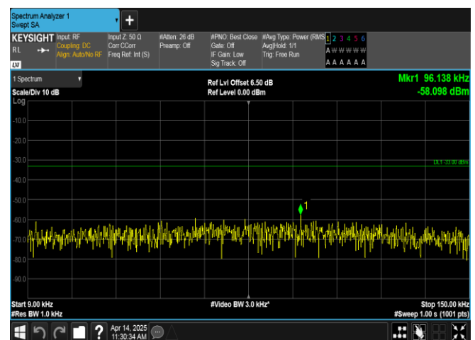
Band17-5MHz-QPSK-23825-1RB#24-0.009~0.15-PASS
