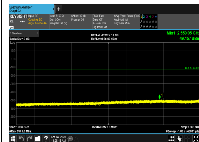
Band17-5MHz-QPSK-23790-25RB#0-1000~3000-PASS
