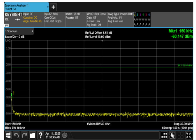
Band17-5MHz-16QAM-23825-1RB#24-0.15~30-PASS
