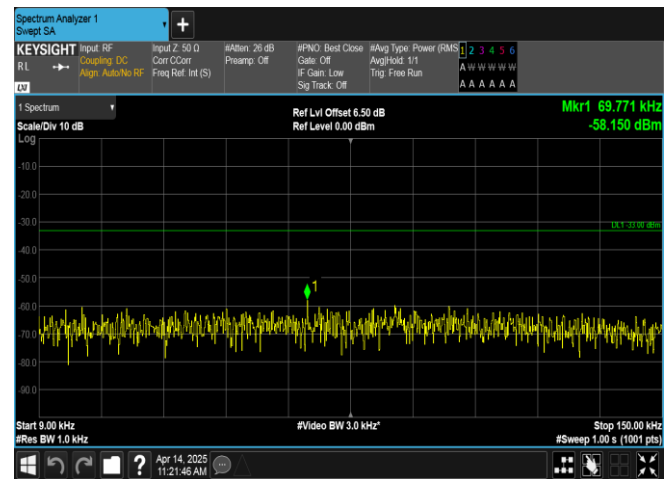
Band17-5MHz-QPSK-23790-1RB#0-0.009~0.15-PASS
