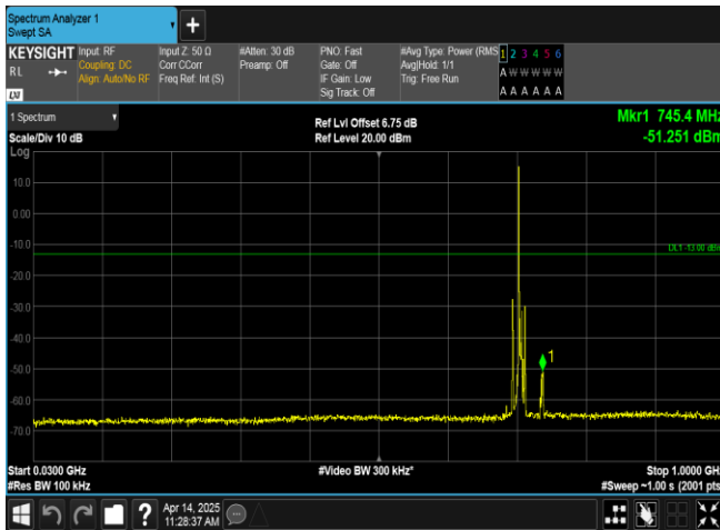
Band17-5MHz-QPSK-23825-1RB#0-30~1000-PASS
