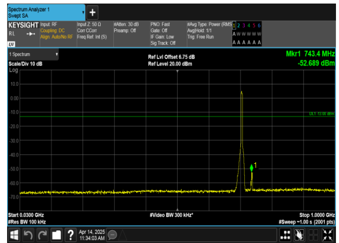
Band17-5MHz-16QAM-23825-25RB#0-30~1000-PASS
