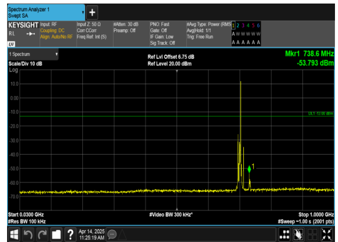
Band17-5MHz-16QAM-23790-1RB#24-30~1000-PASS
