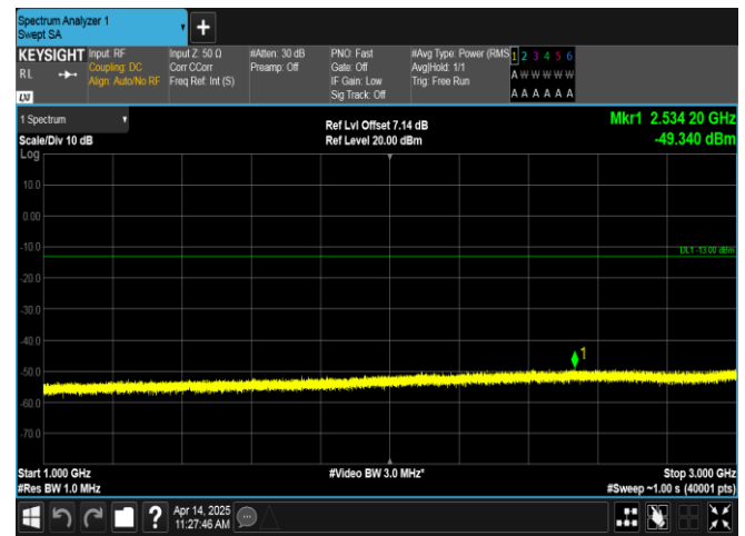
Band17-5MHz-16QAM-23790-25RB#0-1000~3000-PASS
