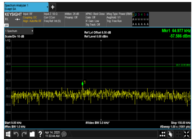
Band17-5MHz-16QAM-23825-25RB#0-0.009~0.15-PASS
