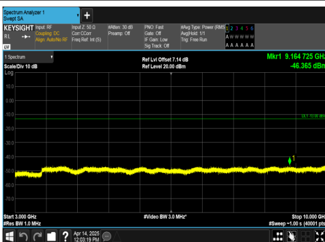
Band17-10MHz-QPSK-23780-1RB#0-3000~10000-PASS
