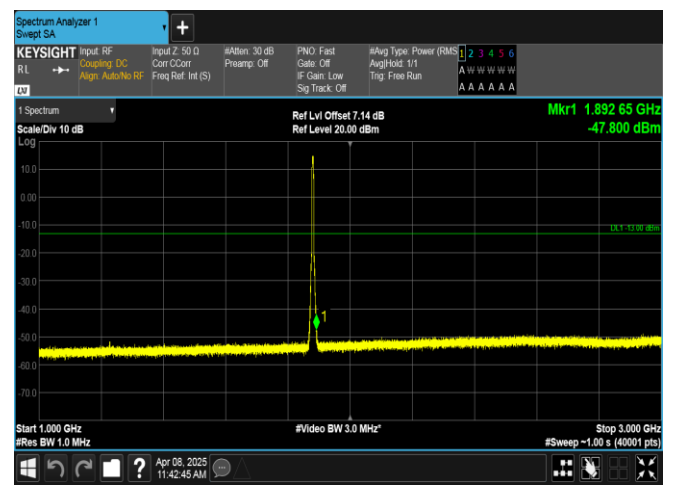
Band2-5MHz-16QAM-18900-25RB#0-1000~3000-PASS
