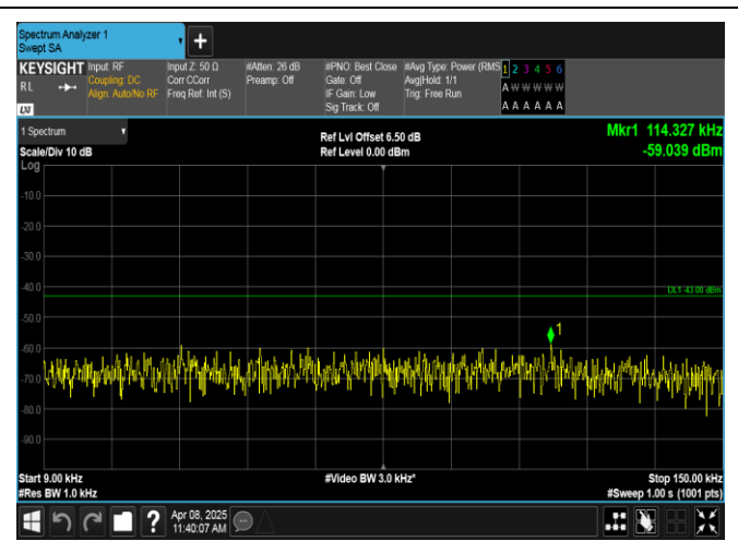
Band2-5MHz-16QAM-18900-1RB#24-0.009~0.15-PASS
