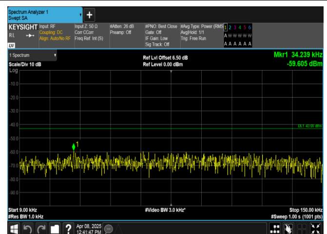
Band2-10MHz-QPSK-18900-1RB#0-0.009~0.15-PASS
