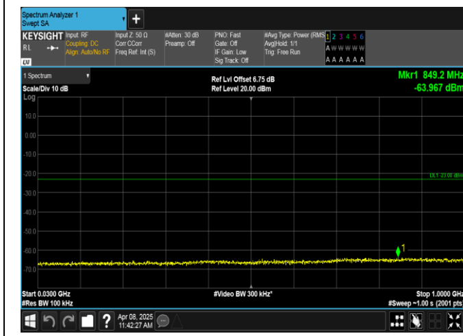
Band2-5MHz-16QAM-18900-25RB#0-30~1000-PASS
