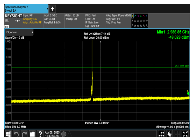
Band2-5MHz-QPSK-19175-1RB#0-1000~3000-PASS
