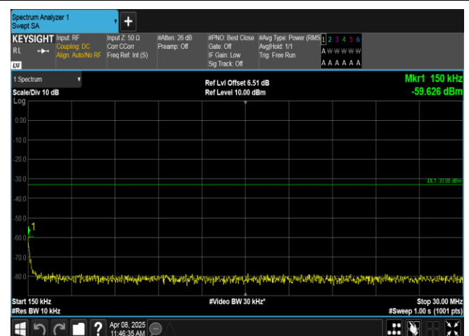
Band2-5MHz-16QAM-19175-1RB#24-0.15~30-PASS
