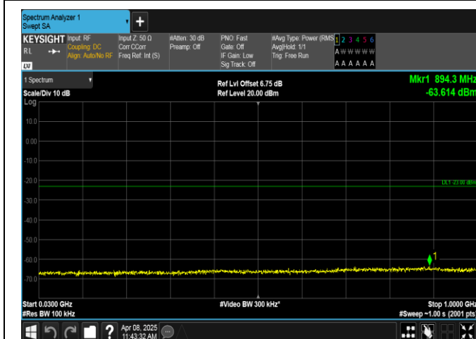
Band2-5MHz-QPSK-19175-1RB#0-30~1000-PASS
