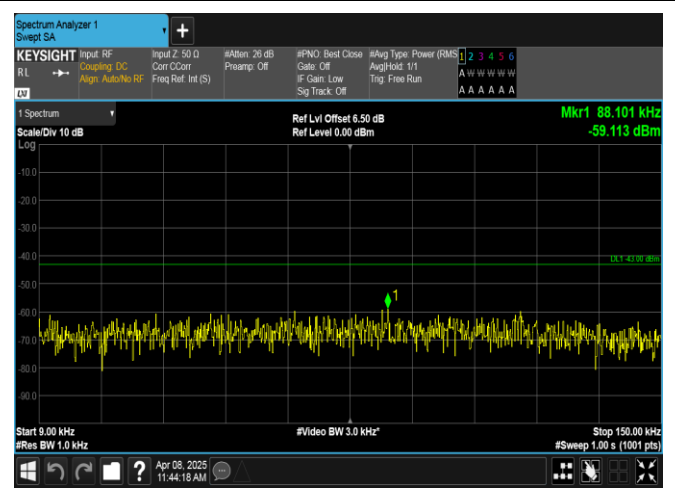
Band2-5MHz-16QAM-19175-1RB#0-0.009~0.15-PASS
