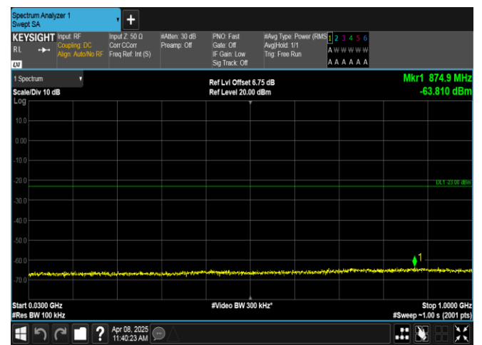
Band2-5MHz-16QAM-18900-1RB#24-30~1000-PASS
