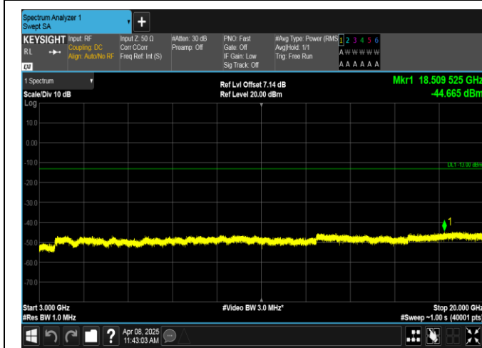
Band2-5MHz-16QAM-18900-25RB#0-3000~20000-PASS
