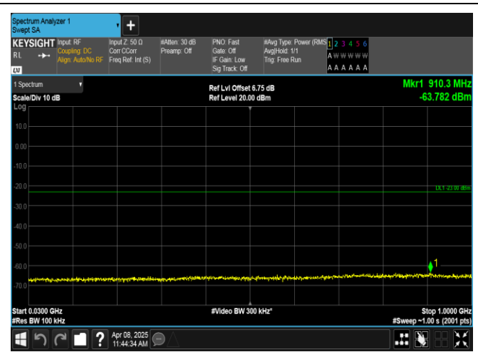
Band2-5MHz-16QAM-19175-1RB#0-30~1000-PASS
