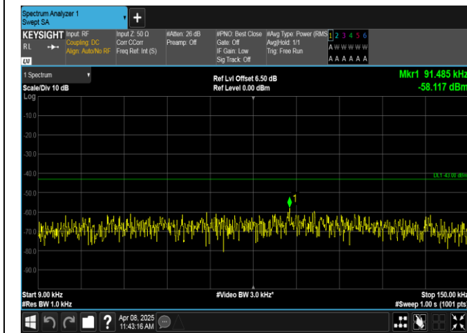
Band2-5MHz-QPSK-19175-1RB#0-0.009~0.15-PASS
