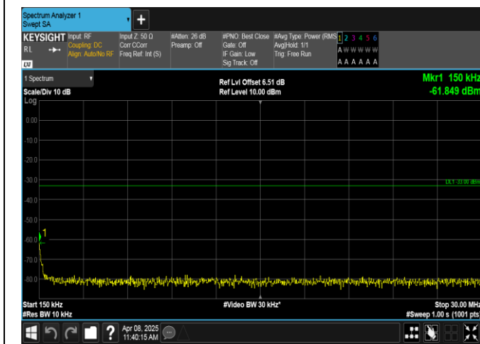
Band2-5MHz-16QAM-18900-1RB#24-0.15~30-PASS
