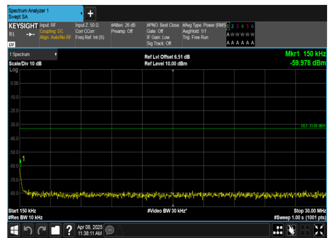
Band2-5MHz-16QAM-18900-1RB#0-0.15~30-PASS
