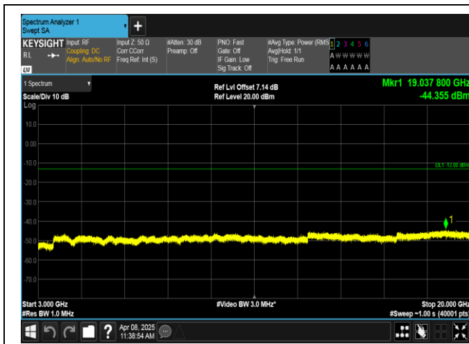
Band2-5MHz-16QAM-18900-1RB#0-3000~20000-PASS
