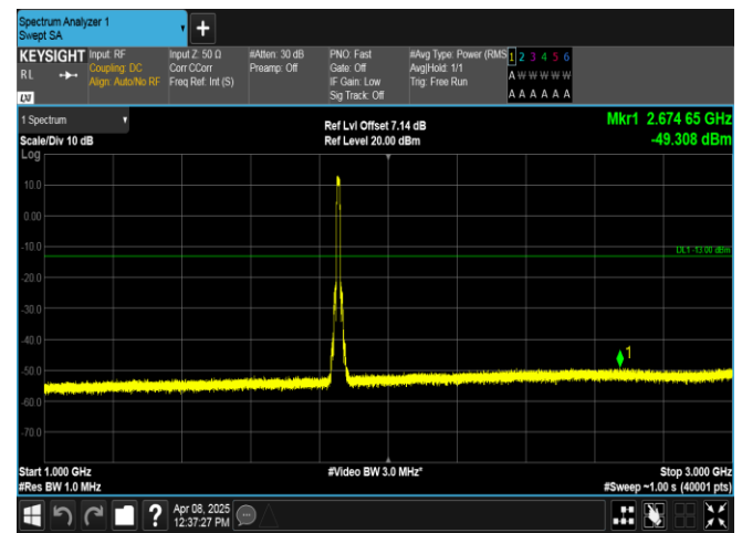
Band2-10MHz-QPSK-18650-50RB#0-1000~3000-PASS
