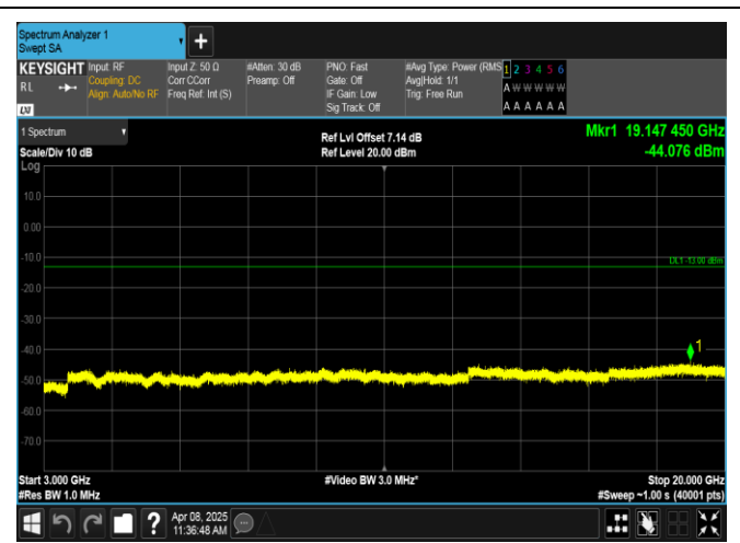
Band2-5MHz-16QAM-18625-25RB#0-3000~20000-PASS
