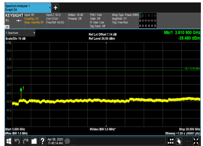
Band2-5MHz-16QAM-19175-1RB#0-3000~20000-PASS
