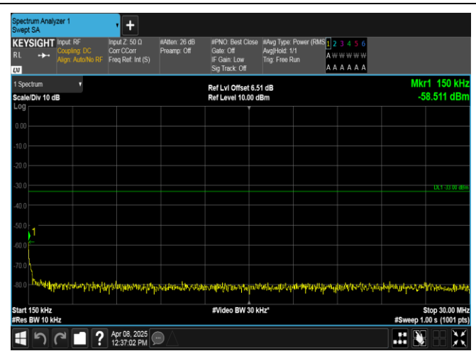
Band2-10MHz-QPSK-18650-50RB#0-0.15~30-PASS
