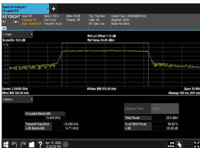
Band38-15MHz-16QAM-38000-75RB#0-PASS
