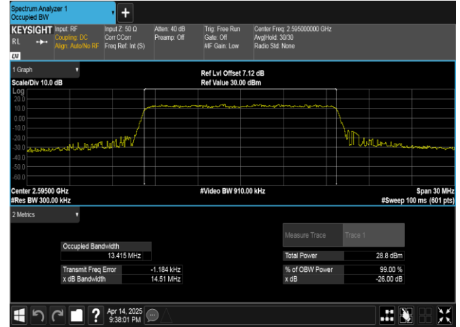
Band38-15MHz-QPSK-38000-75RB#0-PASS
