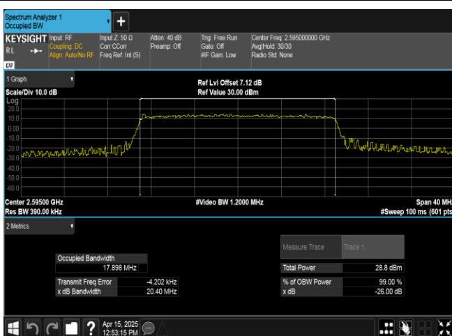
Band38-20MHz-16QAM-38000-100RB#0-PASS
