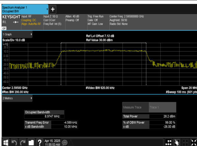
Band38-10MHz-16QAM-38000-50RB#0-PASS
