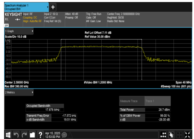
Band38-20MHz-16QAM-37850-100RB#0-PASS
