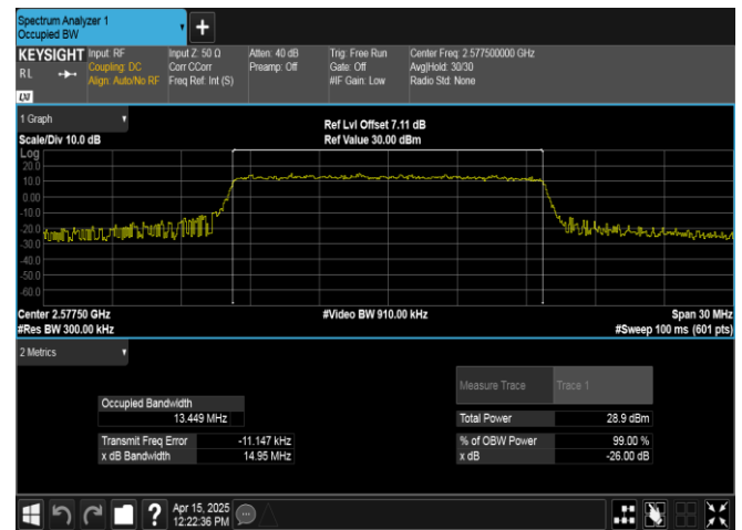
Band38-15MHz-16QAM-37825-75RB#0-PASS
