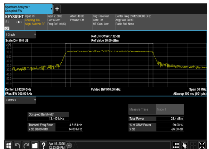
Band38-15MHz-16QAM-38175-75RB#0-PASS
