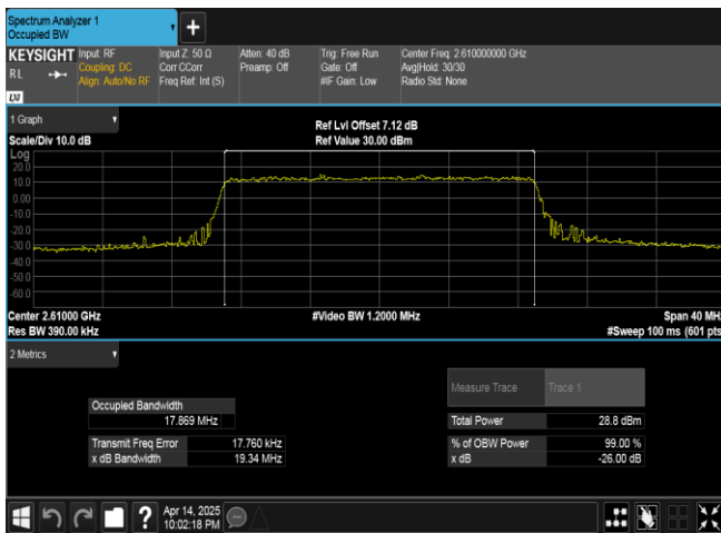
Band38-20MHz-QPSK-38150-100RB#0-PASS
