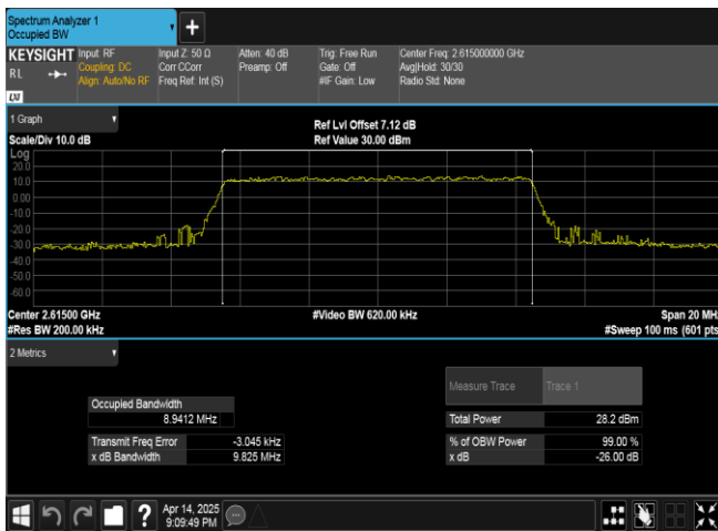
Band38-10MHz-QPSK-38200-50RB#0-PASS
