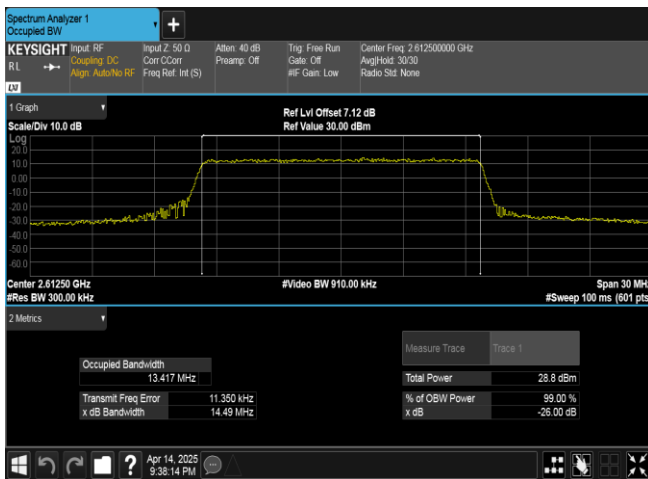
Band38-15MHz-QPSK-38175-75RB#0-PASS
