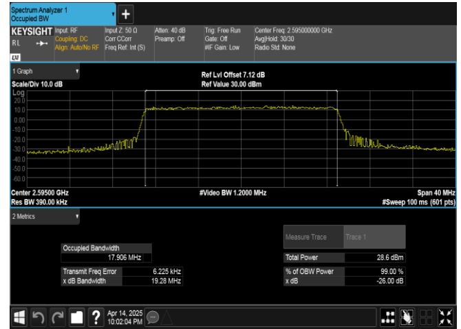
Band38-20MHz-QPSK-38000-100RB#0-PASS
