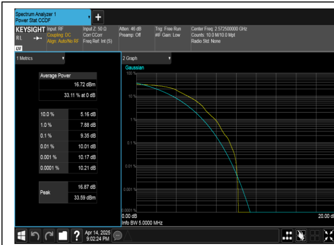
Band38-5MHz-QPSK-37775-1RB#0-PASS
