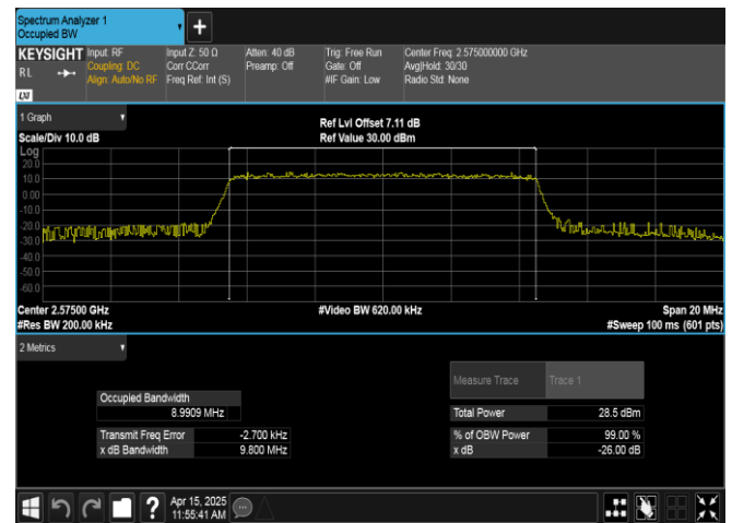
Band38-10MHz-16QAM-37800-50RB#0-PASS
