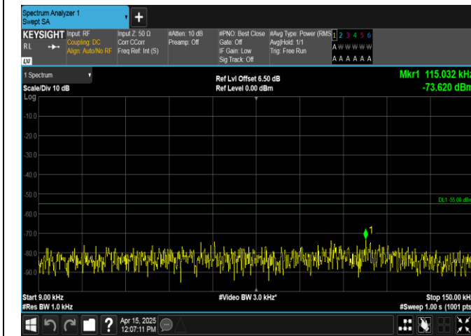
Band38-10MHz-16QAM-38000-50RB#0-0.009~0.15-PASS
