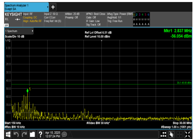
Band38-10MHz-16QAM-38000-50RB#0-0.15~30-PASS
