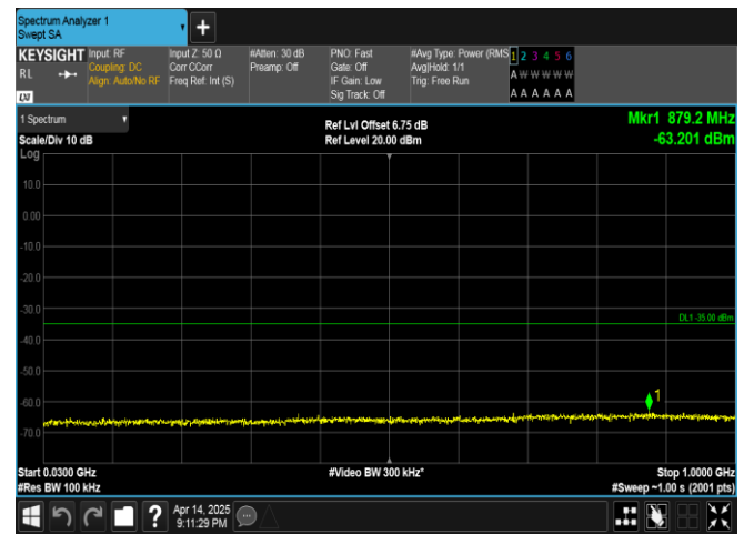
Band38-10MHz-16QAM-37800-1RB#0-30~1000-PASS
