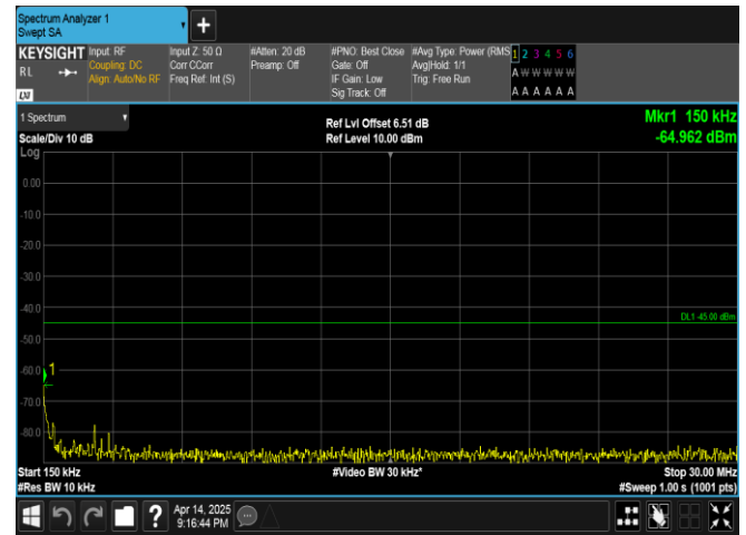
Band38-10MHz-QPSK-38000-1RB#49-0.15~30-PASS
