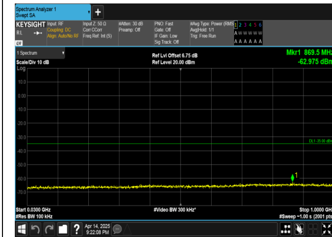
Band38-10MHz-16QAM-38200-1RB#49-30~1000-PASS
