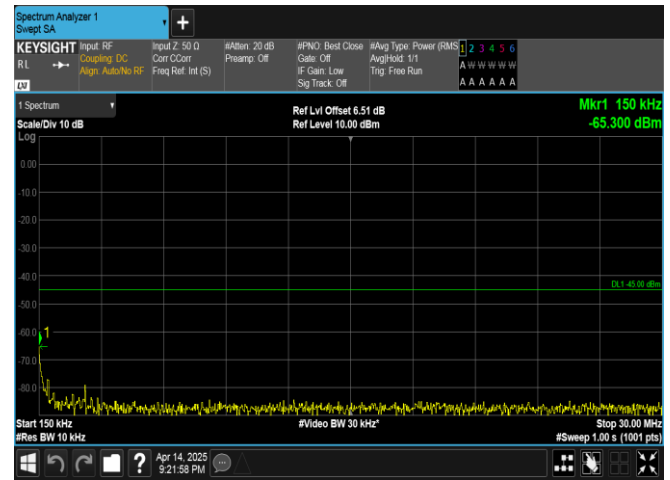
Band38-10MHz-16QAM-38200-1RB#49-0.15~30-PASS
