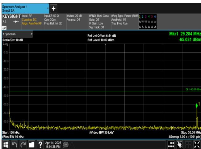
Band38-10MHz-QPSK-38000-1RB#0-0.15~30-PASS
