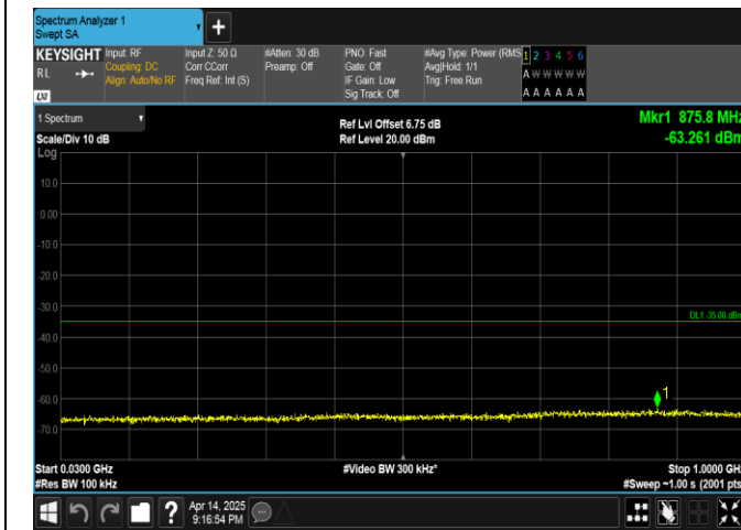
Band38-10MHz-QPSK-38000-1RB#49-30~1000-PASS
