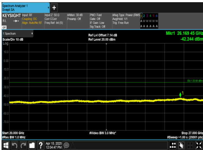
Band38-10MHz-QPSK-37800-50RB#0-20000~27000-PASS
