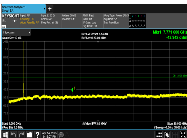
Band38-10MHz-QPSK-38000-1RB#0-1000~20000-PASS
