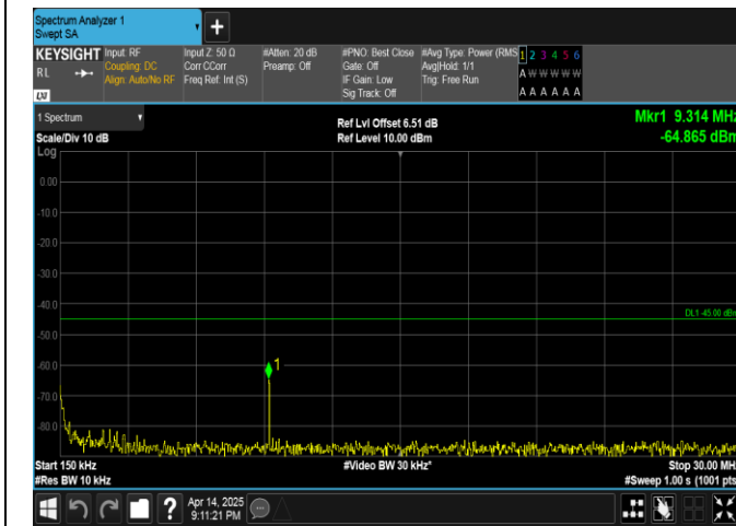
Band38-10MHz-16QAM-37800-1RB#0-0.15~30-PASS
