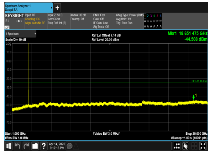
Band38-10MHz-QPSK-38000-1RB#49-1000~20000-PASS
