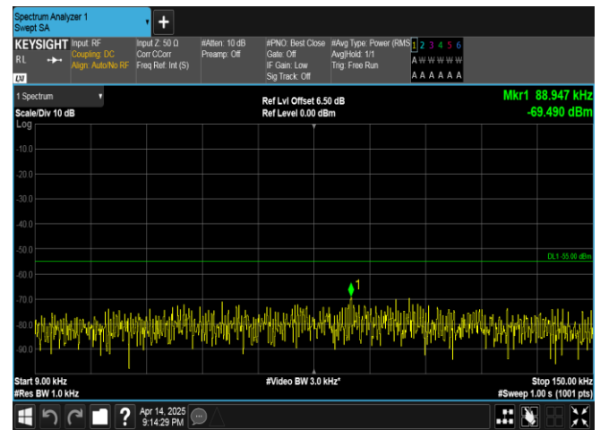
Band38-10MHz-QPSK-38000-1RB#0-0.009~0.15-PASS
