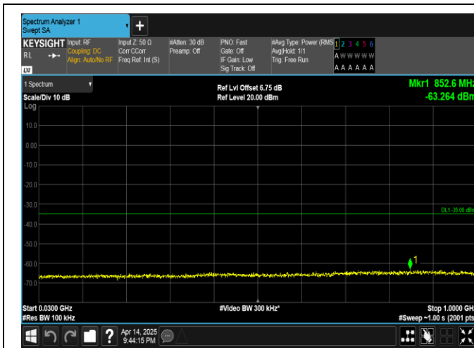
Band38-15MHz-16QAM-38000-1RB#0-30~1000-PASS
