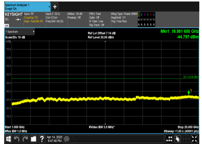
Band38-15MHz-QPSK-38175-1RB#0-1000~20000-PASS
