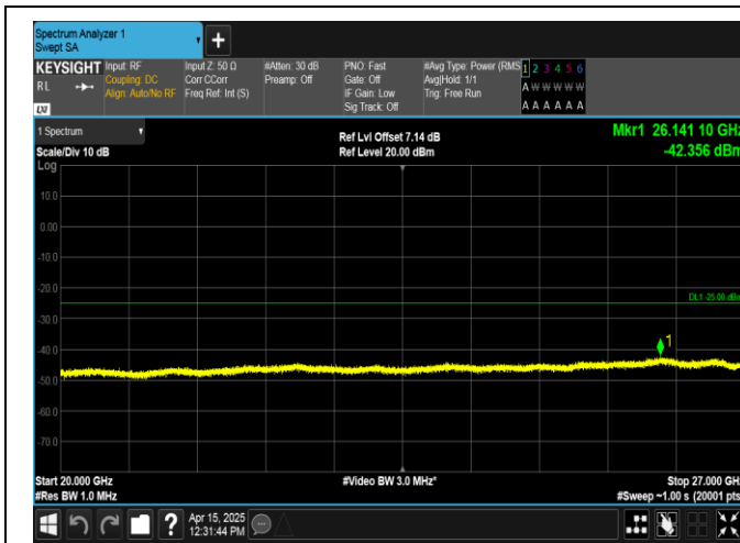
Band38-15MHz-QPSK-37825-75RB#0-20000~27000-PASS
