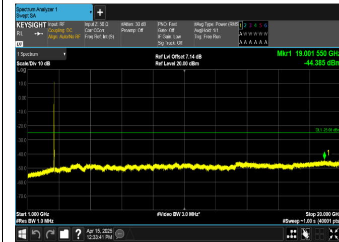
Band38-15MHz-QPSK-38000-75RB#0-1000~20000-PASS
