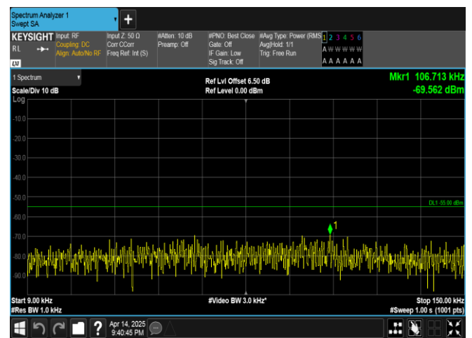
Band38-15MHz-QPSK-37825-1RB#74-0.009~0.15-PASS
