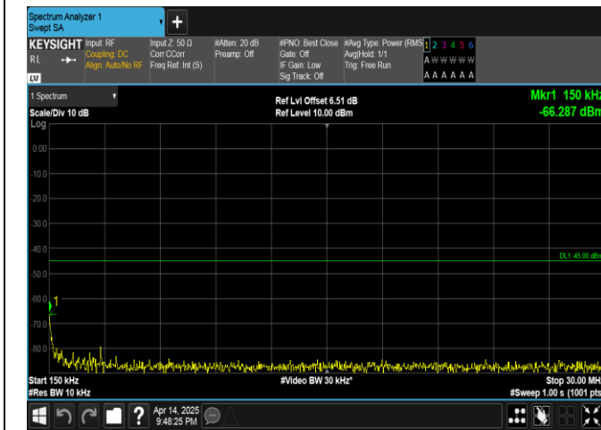
Band38-15MHz-16QAM-38175-1RB#0-0.15~30-PASS
