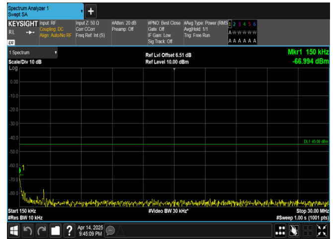
Band38-15MHz-QPSK-38000-1RB#74-0.15~30-PASS
