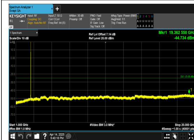
Band38-15MHz-16QAM-37825-1RB#0-1000~20000-PASS
