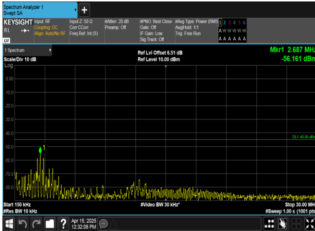
Band38-15MHz-16QAM-37825-75RB#0-0.15~30-PASS
