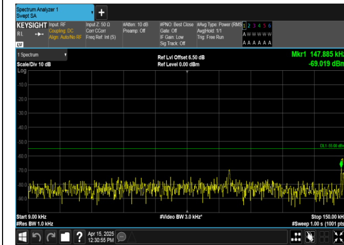
Band38-15MHz-QPSK-37825-75RB#0-0.009~0.15-PASS
