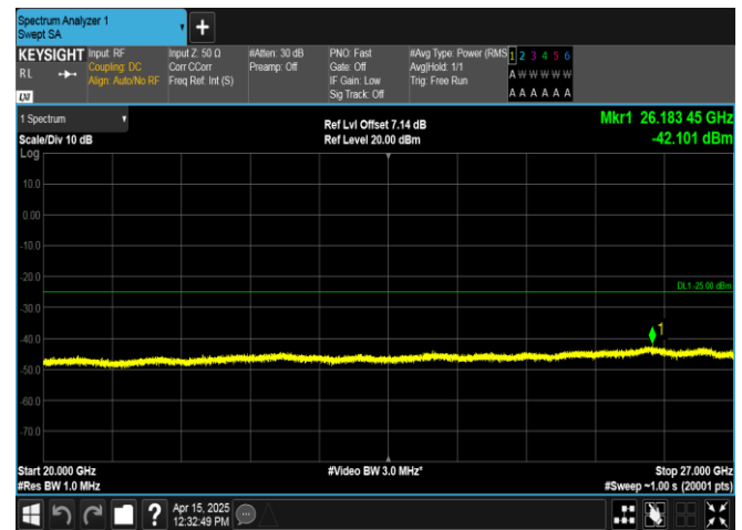
Band38-15MHz-16QAM-37825-75RB#0-20000~27000-PASS
