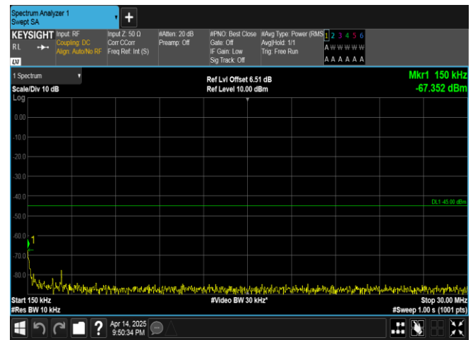
Band38-15MHz-16QAM-38175-1RB#74-0.15~30-PASS
