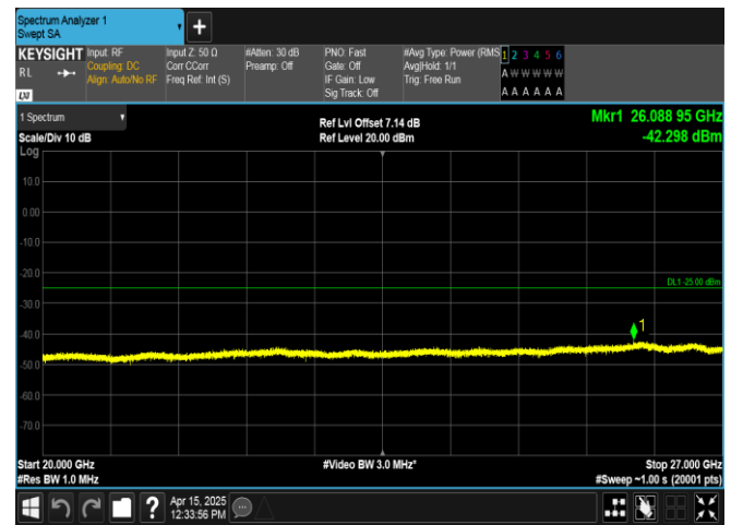
Band38-15MHz-QPSK-38000-75RB#0-20000~27000-PASS
