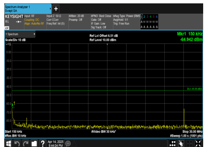
Band38-15MHz-16QAM-38000-1RB#0-0.15~30-PASS
