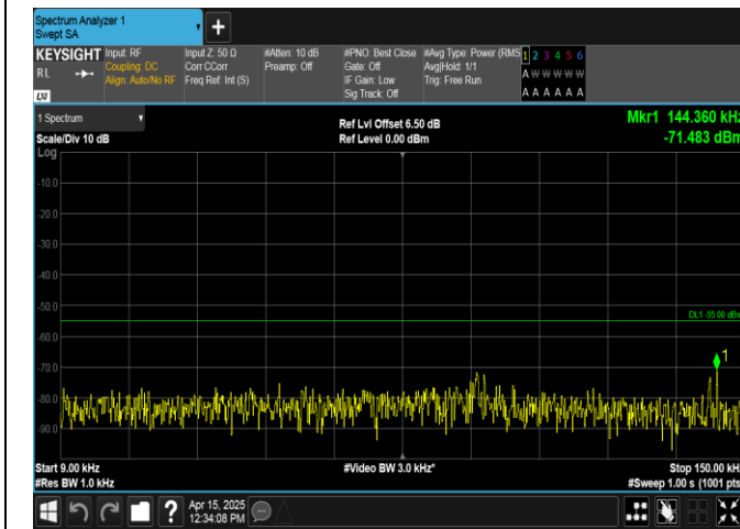
Band38-15MHz-16QAM-38000-75RB#0-0.009~0.15-PASS
