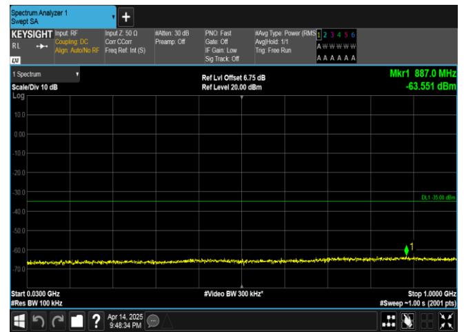
Band38-15MHz-16QAM-38175-1RB#0-30~1000-PASS
