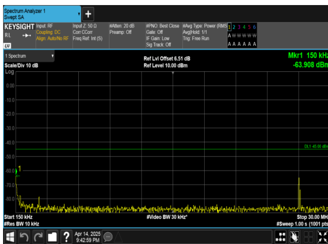
Band38-15MHz-QPSK-38000-1RB#0-0.15~30-PASS
