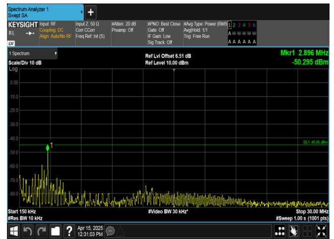
Band38-15MHz-QPSK-37825-75RB#0-0.15~30-PASS
