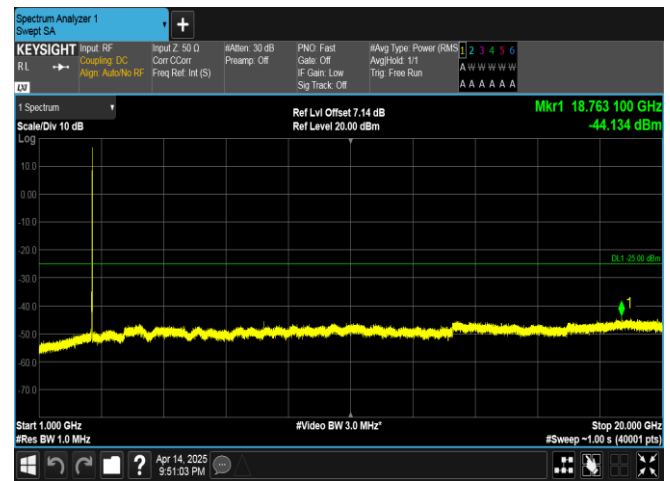
Band38-15MHz-16QAM-38175-1RB#74-1000~20000-PASS
