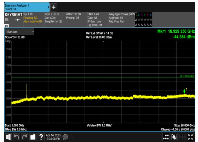
Band38-15MHz-QPSK-37825-1RB#0-1000~20000-PASS
