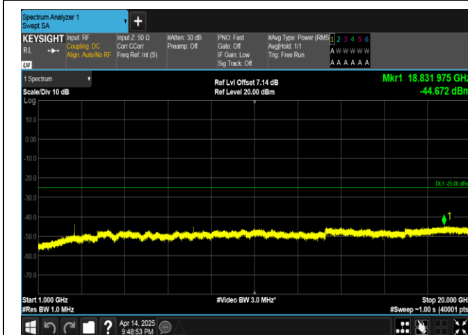
Band38-15MHz-16QAM-38175-1RB#0-1000~20000-PASS
