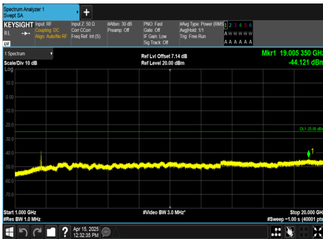
Band38-15MHz-16QAM-37825-75RB#0-1000~20000-PASS
