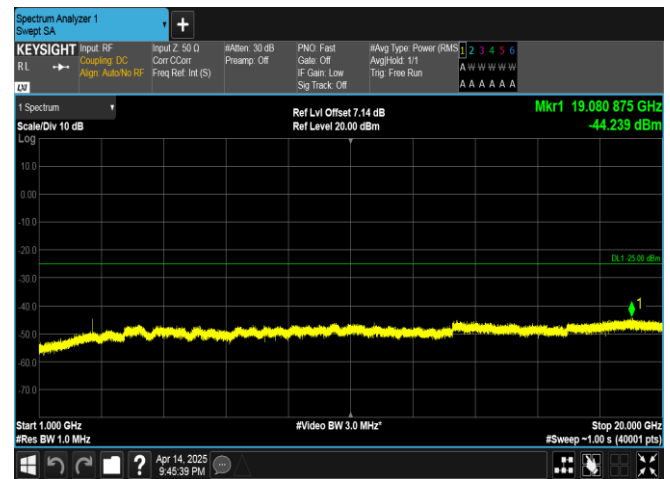
Band38-15MHz-QPSK-38000-1RB#74-1000~20000-PASS
