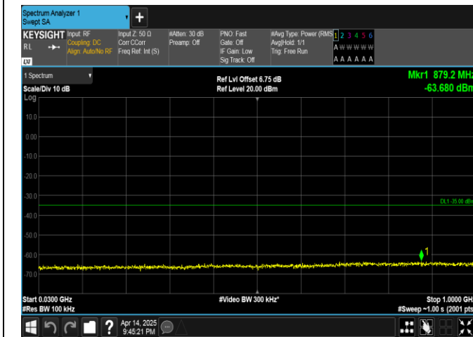
Band38-15MHz-QPSK-38000-1RB#74-30~1000-PASS
