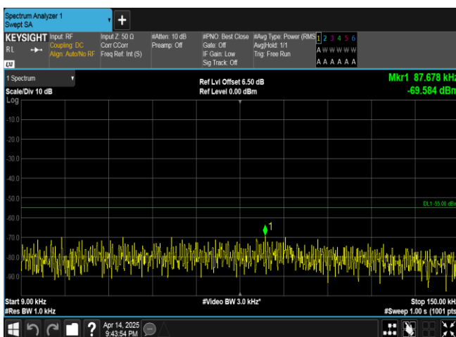
Band38-15MHz-16QAM-38000-1RB#0-0.009~0.15-PASS
