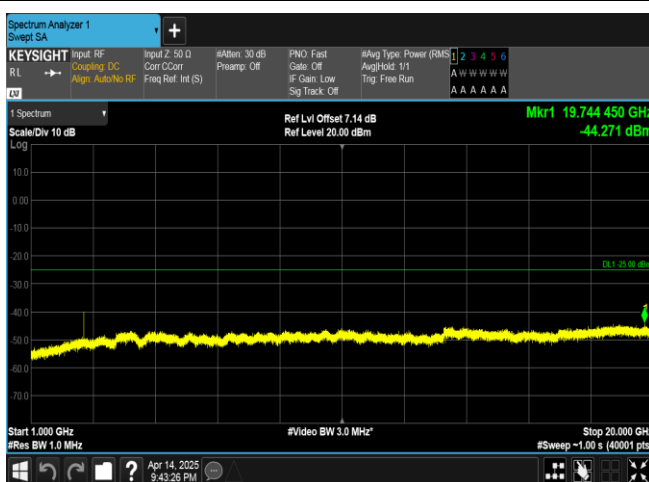
Band38-15MHz-QPSK-38000-1RB#0-1000~20000-PASS
