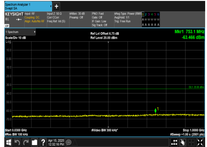
Band38-15MHz-16QAM-37825-75RB#0-30~1000-PASS
