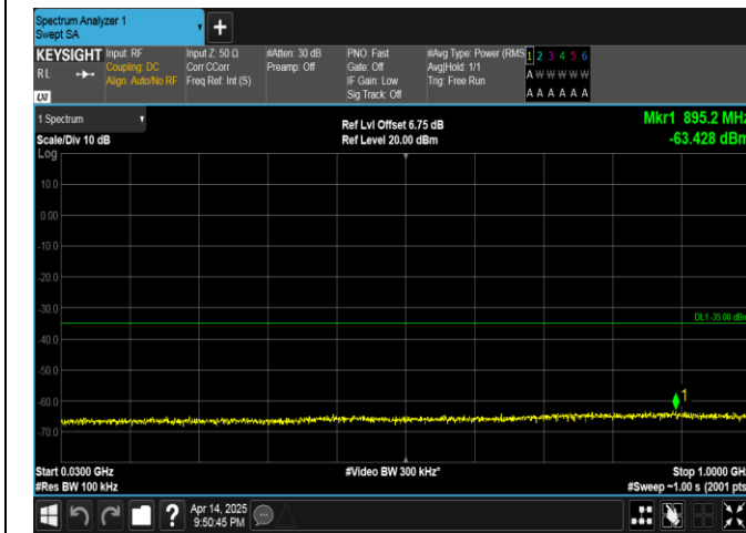
Band38-15MHz-16QAM-38175-1RB#74-30~1000-PASS
