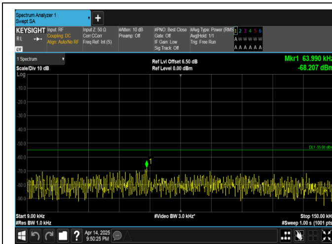
Band38-15MHz-16QAM-38175-1RB#74-0.009~0.15-PASS
