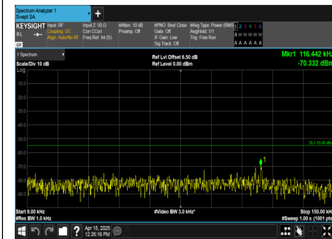
Band38-15MHz-QPSK-38175-75RB#0-0.009~0.15-PASS
