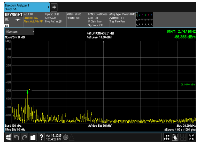
Band38-15MHz-16QAM-38000-75RB#0-0.15~30-PASS
