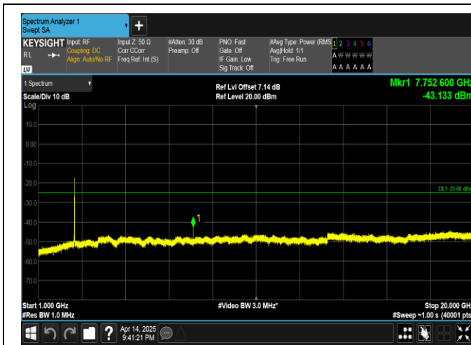
Band38-15MHz-QPSK-37825-1RB#74-1000~20000-PASS
