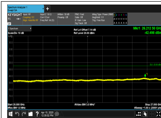
Band38-15MHz-16QAM-38000-75RB#0-20000~27000-PASS
