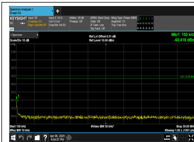
Band4-5MHz-QPSK-20375-1RB#24-0.15~30-PASS
