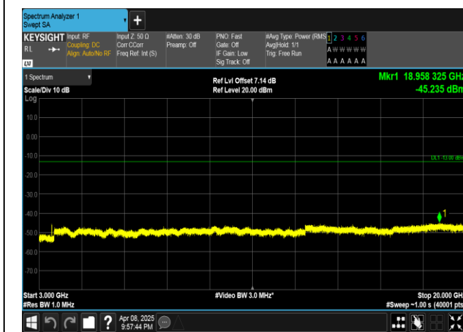
Band4-5MHz-QPSK-20375-25RB#0-3000~20000-PASS
