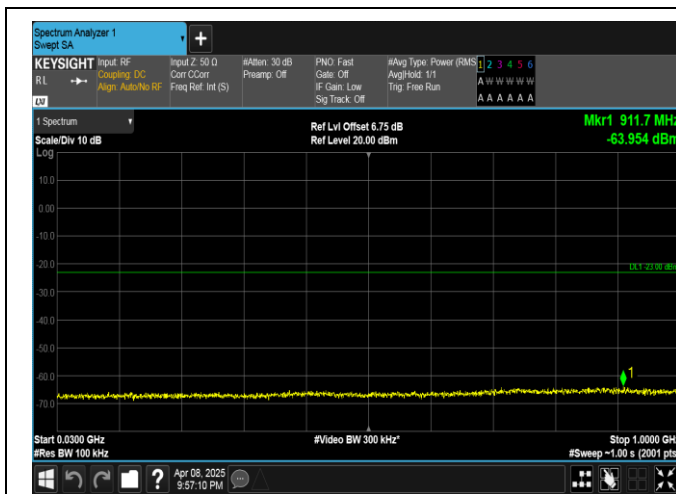
Band4-5MHz-QPSK-20375-25RB#0-30~1000-PASS
