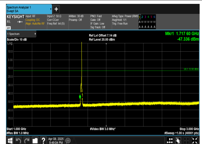
Band4-5MHz-QPSK-20175-1RB#24-1000~3000-PASS
