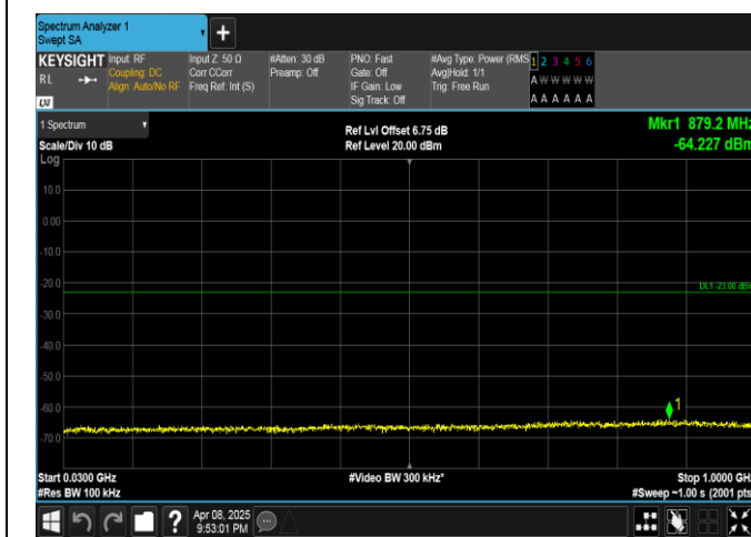
Band4-5MHz-QPSK-20375-1RB#0-30~1000-PASS
