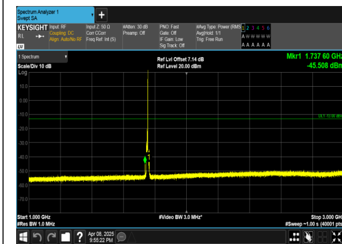
Band4-5MHz-QPSK-20375-1RB#24-1000~3000-PASS
