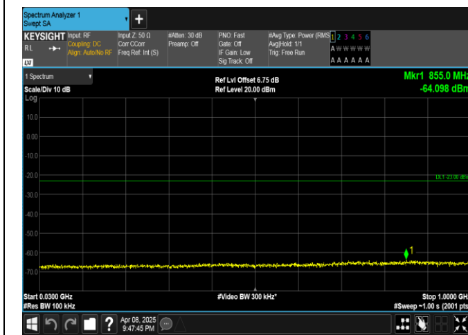
Band4-5MHz-16QAM-20175-1RB#0-30~1000-PASS
