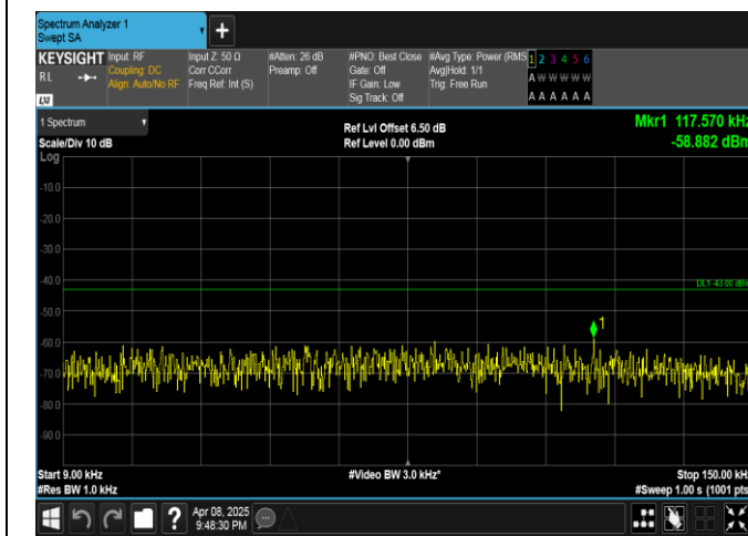
Band4-5MHz-QPSK-20175-1RB#24-0.009~0.15-PASS
