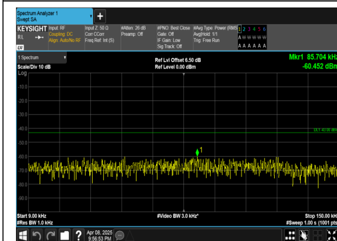
Band4-5MHz-QPSK-20375-25RB#0-0.009~0.15-PASS
