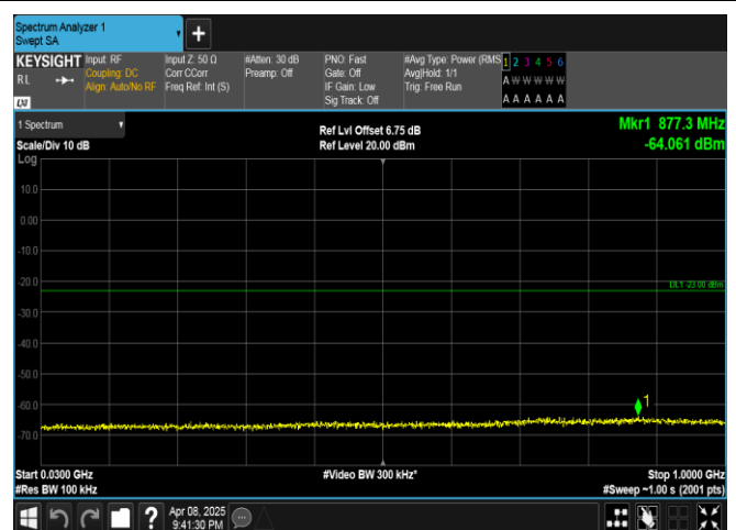
Band4-5MHz-16QAM-19975-1RB#0-30~1000-PASS
