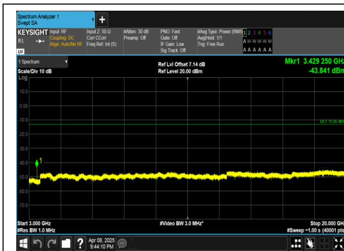
Band4-5MHz-16QAM-19975-1RB#24-3000~20000-PASS
