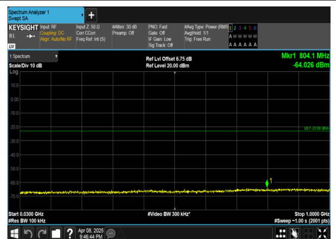
Band4-5MHz-QPSK-20175-1RB#0-30~1000-PASS
