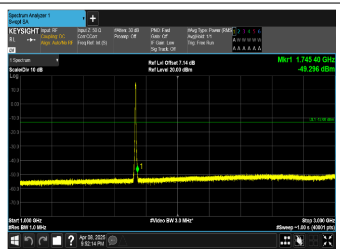
Band4-5MHz-16QAM-20175-25RB#0-1000~3000-PASS
