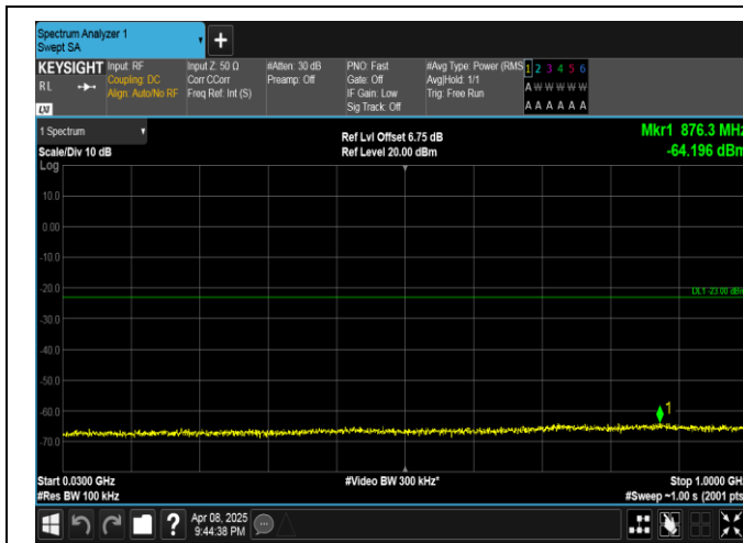
Band4-5MHz-QPSK-19975-25RB#0-30~1000-PASS
