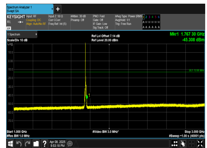
Band4-5MHz-QPSK-20375-1RB#0-1000~3000-PASS
