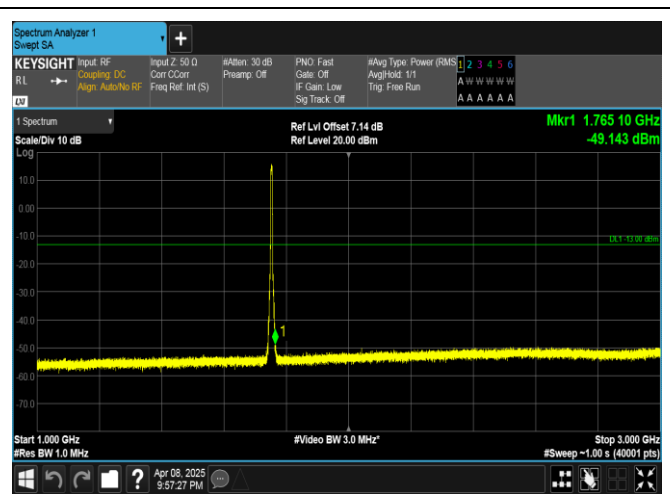
Band4-5MHz-QPSK-20375-25RB#0-1000~3000-PASS
