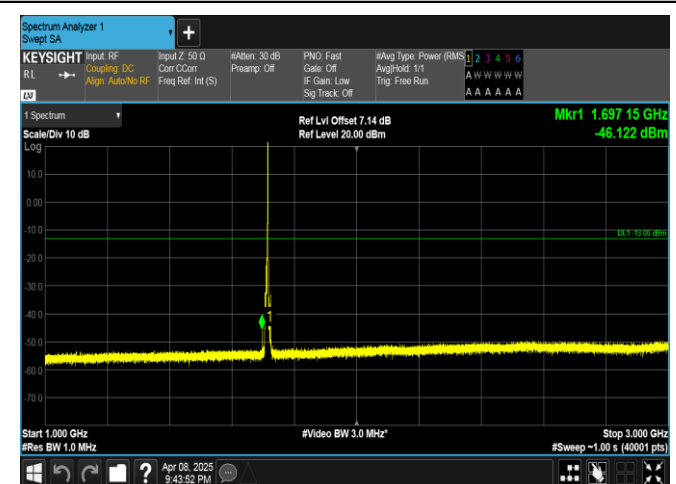
Band4-5MHz-16QAM-19975-1RB#24-1000~3000-PASS
