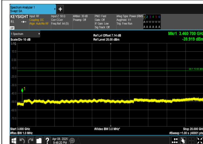
Band4-5MHz-16QAM-20175-1RB#0-3000~20000-PASS
