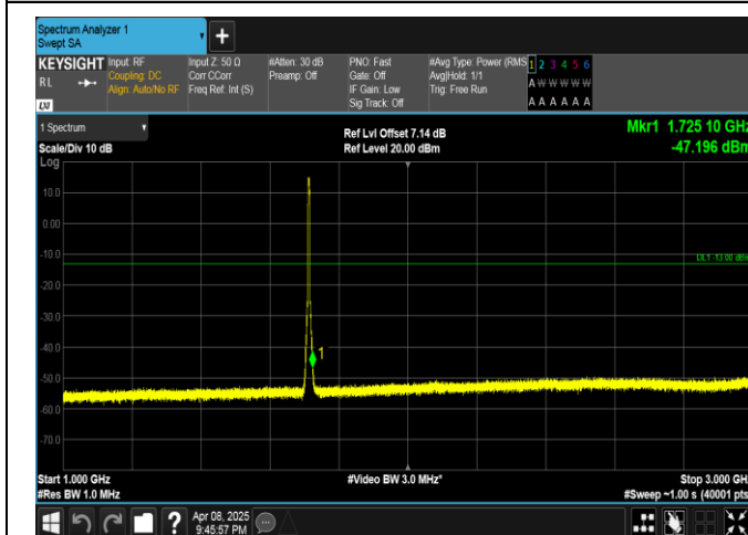
Band4-5MHz-16QAM-19975-25RB#0-1000~3000-PASS
