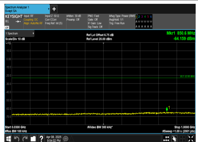
Band4-5MHz-16QAM-20375-1RB#0-30~1000-PASS
