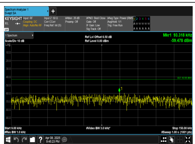
Band4-5MHz-16QAM-19975-25RB#0-0.009~0.15-PASS
