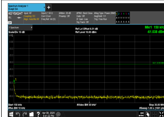
Band4-5MHz-16QAM-19975-1RB#0-0.15~30-PASS
