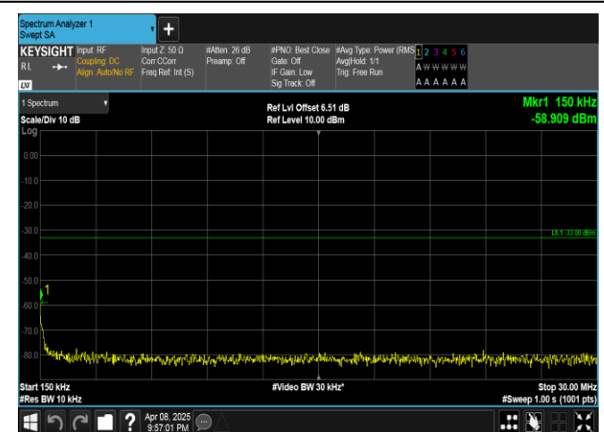
Band4-5MHz-QPSK-20375-25RB#0-0.15~30-PASS
