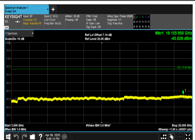
Band4-5MHz-16QAM-19975-25RB#0-3000~20000-PASS
