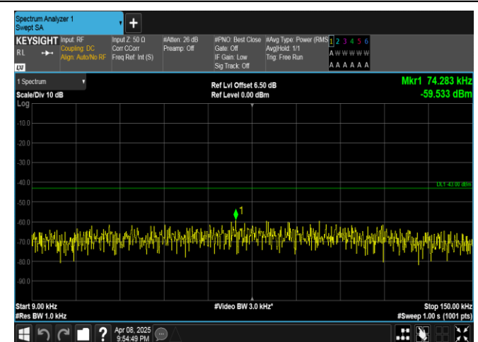
Band4-5MHz-QPSK-20375-1RB#24-0.009~0.15-PASS
