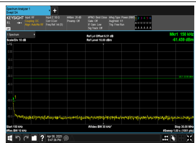
Band4-5MHz-16QAM-20175-1RB#0-0.15~30-PASS
