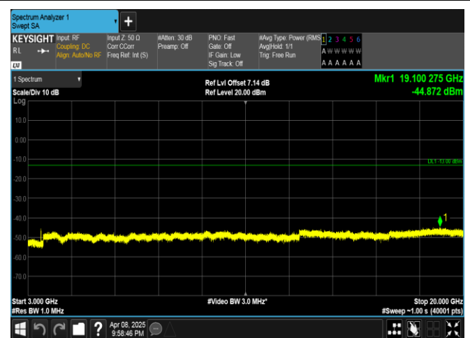
Band4-5MHz-16QAM-20375-25RB#0-3000~20000-PASS
