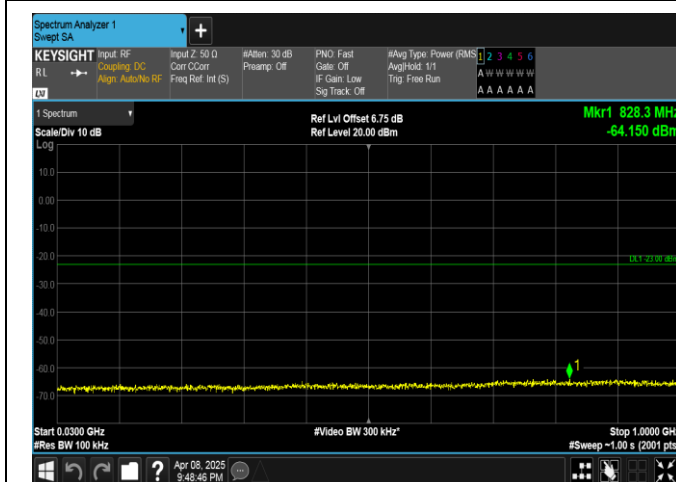
Band4-5MHz-QPSK-20175-1RB#24-30~1000-PASS
