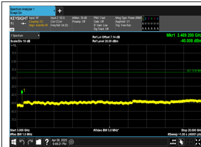
Band4-5MHz-QPSK-20175-1RB#24-3000~20000-PASS
