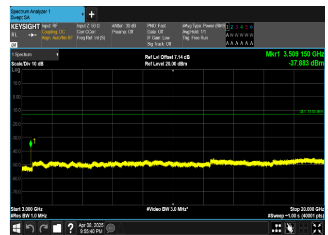
Band4-5MHz-QPSK-20375-1RB#24-3000~20000-PASS
