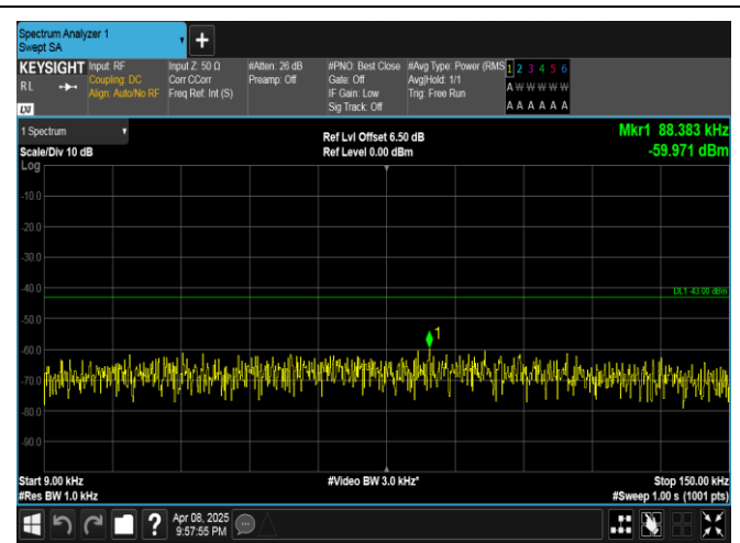
Band4-5MHz-16QAM-20375-25RB#0-0.009~0.15-PASS
