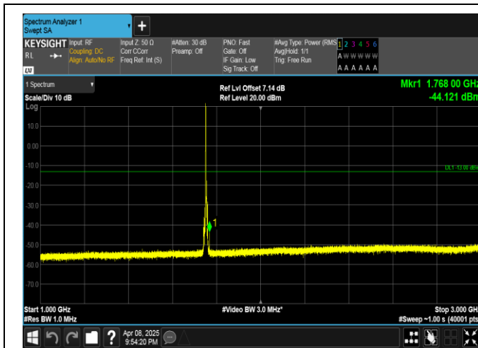
Band4-5MHz-16QAM-20375-1RB#0-1000~3000-PASS
