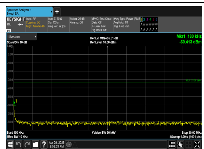
Band4-5MHz-QPSK-20375-1RB#0-0.15~30-PASS
