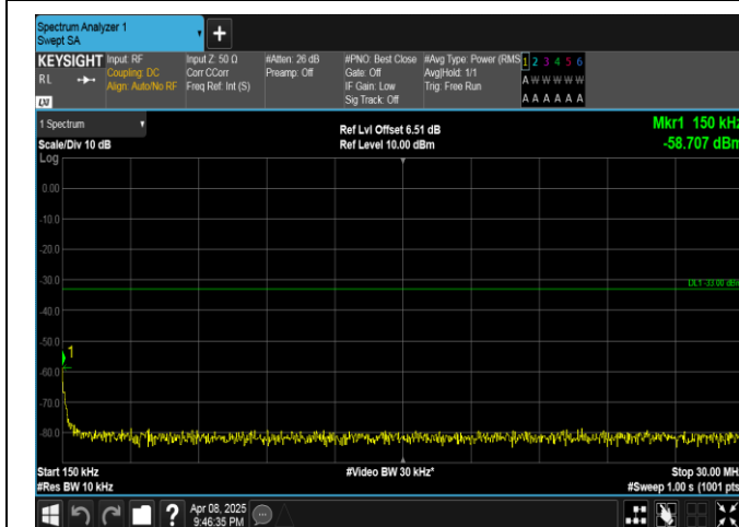
Band4-5MHz-QPSK-20175-1RB#0-0.15~30-PASS
