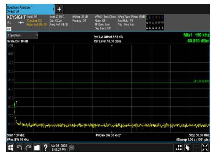
Band4-5MHz-16QAM-19975-1RB#24-0.15~30-PASS
