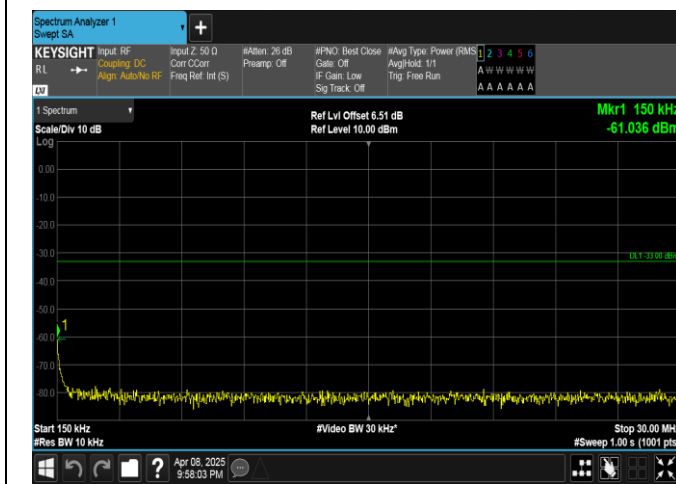
Band4-5MHz-16QAM-20375-25RB#0-0.15~30-PASS
