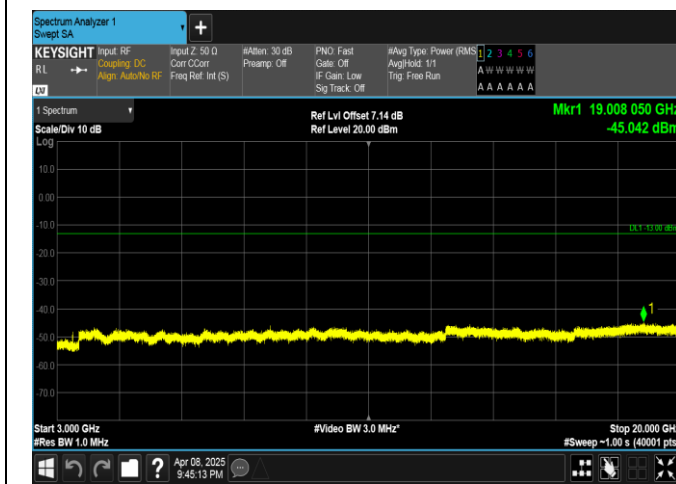
Band4-5MHz-QPSK-19975-25RB#0-3000~20000-PASS
