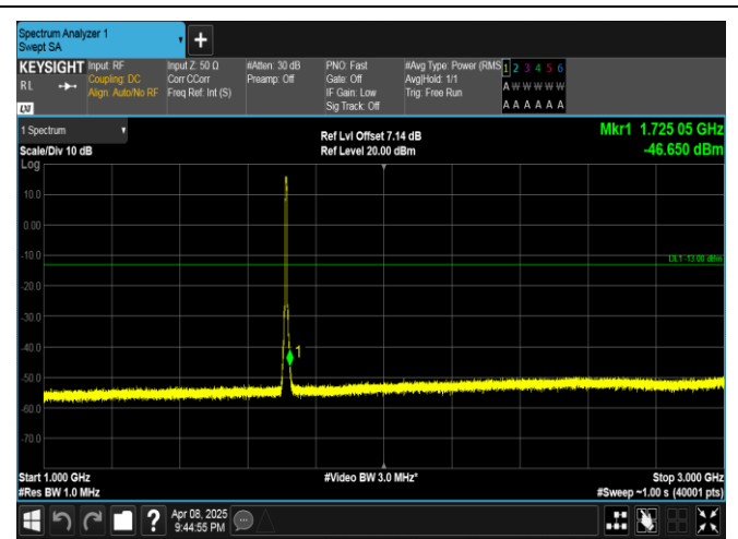
Band4-5MHz-QPSK-19975-25RB#0-1000~3000-PASS
