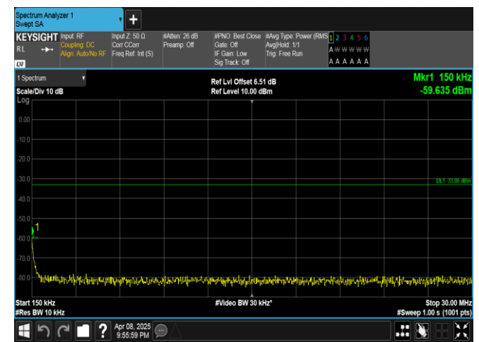
Band4-5MHz-16QAM-20375-1RB#24-0.15~30-PASS
