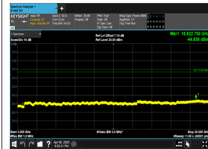
Band4-5MHz-16QAM-20175-25RB#0-3000~20000-PASS
