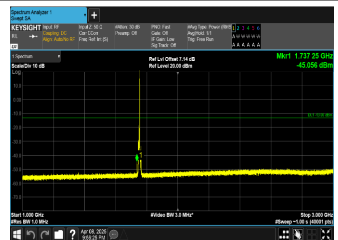
Band4-5MHz-16QAM-20375-1RB#24-1000~3000-PASS
