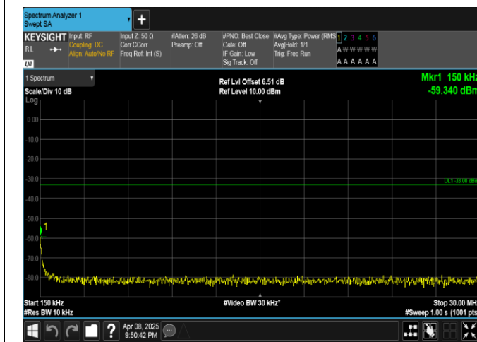
Band4-5MHz-QPSK-20175-25RB#0-0.15~30-PASS
