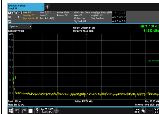
Band4-5MHz-16QAM-19975-25RB#0-0.15~30-PASS
