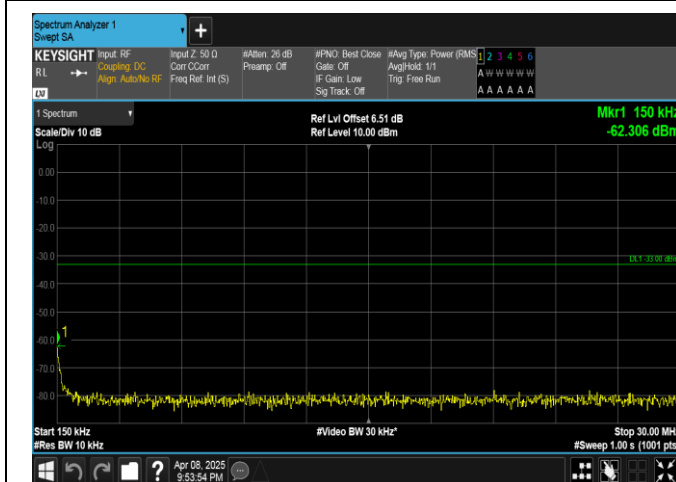
Band4-5MHz-16QAM-20375-1RB#0-0.15~30-PASS
