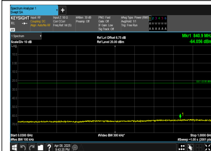
Band4-5MHz-16QAM-19975-1RB#24-30~1000-PASS
