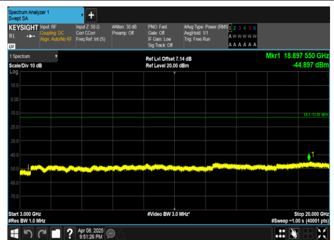
Band4-5MHz-QPSK-20175-25RB#0-3000~20000-PASS
