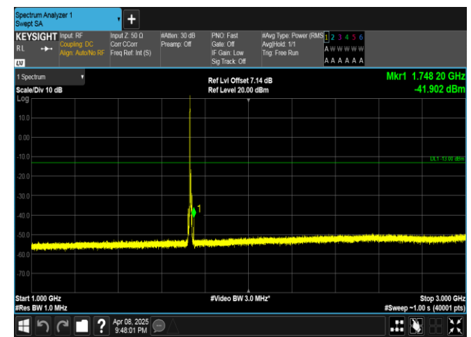
Band4-5MHz-16QAM-20175-1RB#0-1000~3000-PASS
