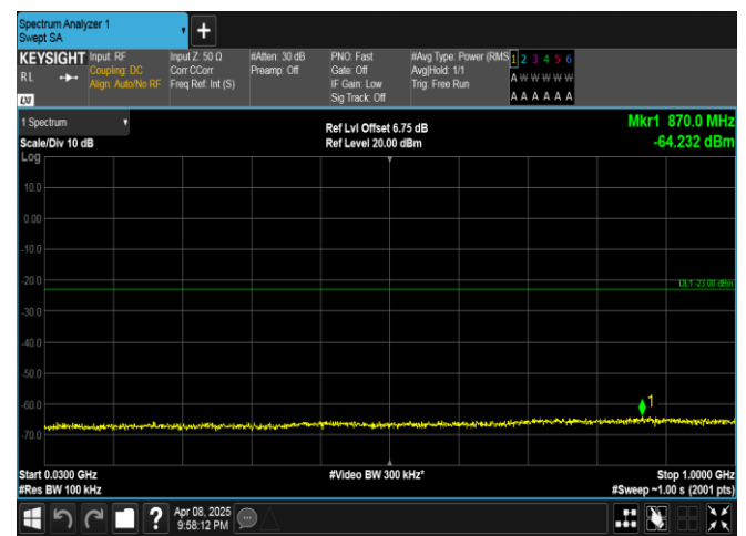
Band4-5MHz-16QAM-20375-25RB#0-30~1000-PASS
