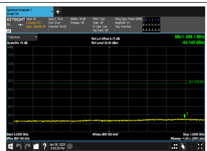
Band4-5MHz-QPSK-20375-1RB#24-30~1000-PASS
