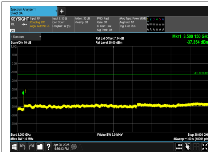
Band4-5MHz-16QAM-20375-1RB#24-3000~20000-PASS
