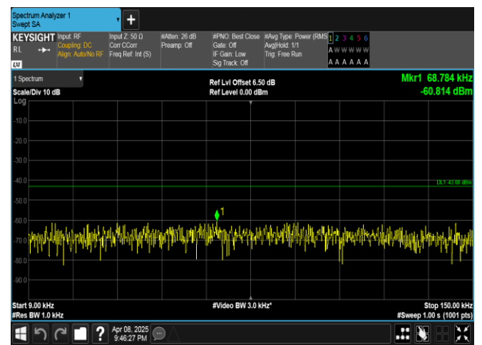
Band4-5MHz-QPSK-20175-1RB#0-0.009~0.15-PASS
