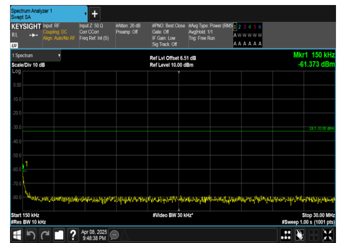
Band4-5MHz-QPSK-20175-1RB#24-0.15~30-PASS
