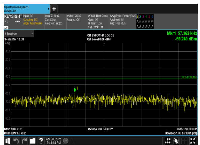
Band4-5MHz-16QAM-19975-1RB#0-0.009~0.15-PASS
