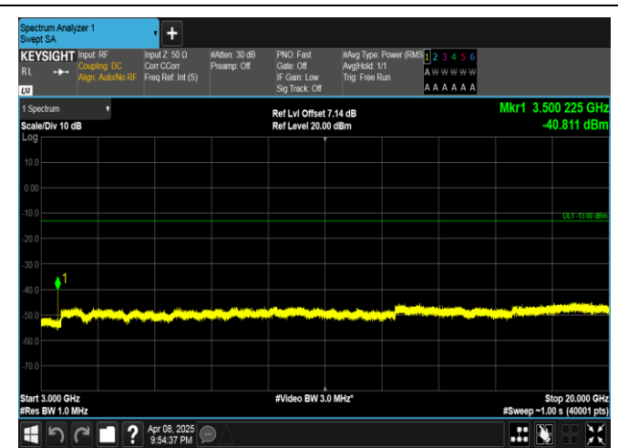
Band4-5MHz-16QAM-20375-1RB#0-3000~20000-PASS
