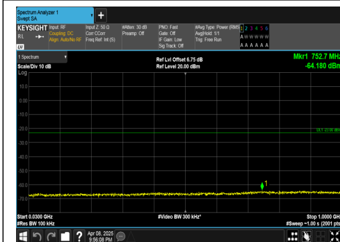
Band4-5MHz-16QAM-20375-1RB#24-30~1000-PASS
