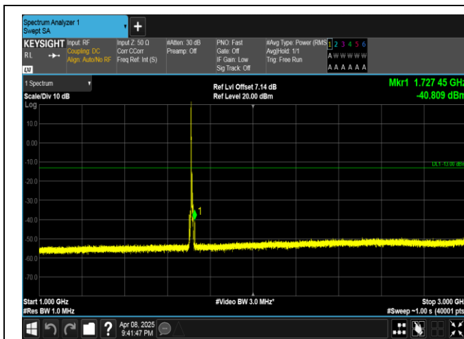
Band4-5MHz-16QAM-19975-1RB#0-1000~3000-PASS
