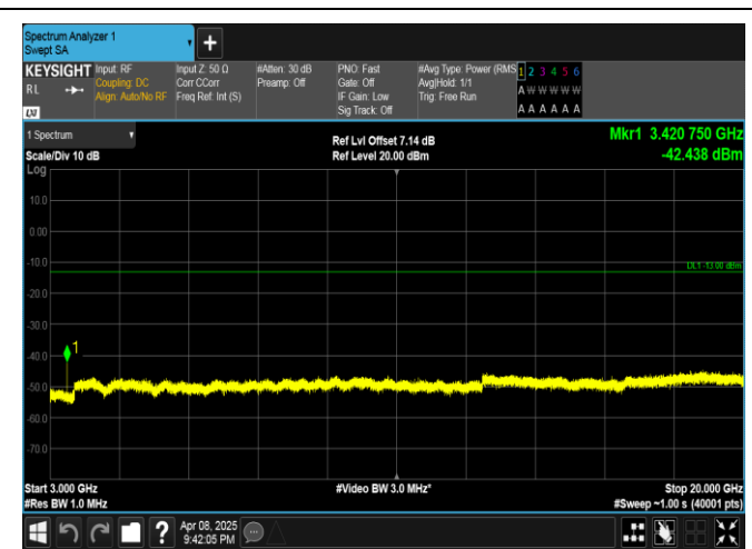
Band4-5MHz-16QAM-19975-1RB#0-3000~20000-PASS
