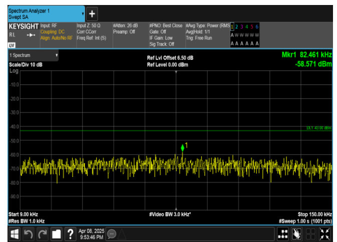
Band4-5MHz-16QAM-20375-1RB#0-0.009~0.15-PASS
