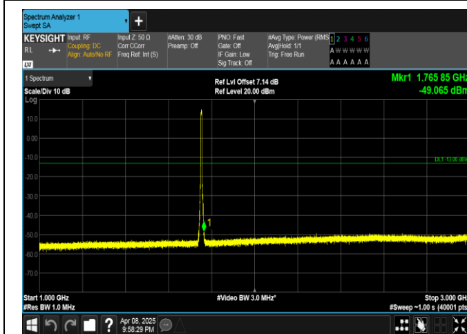
Band4-5MHz-16QAM-20375-25RB#0-1000~3000-PASS
