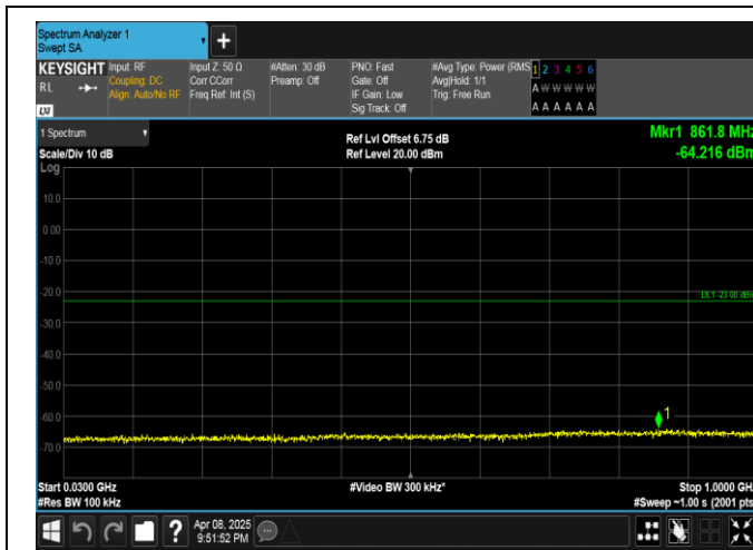
Band4-5MHz-16QAM-20175-25RB#0-30~1000-PASS
