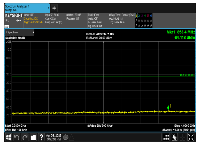
Band4-5MHz-QPSK-20175-25RB#0-30~1000-PASS
