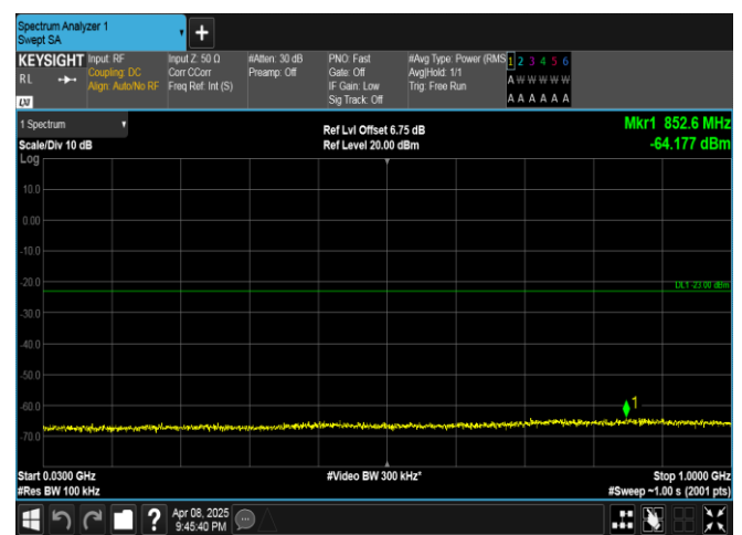
Band4-5MHz-16QAM-19975-25RB#0-30~1000-PASS
