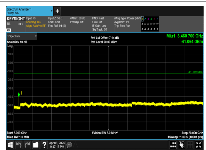
Band4-5MHz-QPSK-20175-1RB#0-3000~20000-PASS
