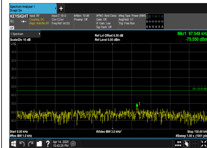
Band41-5MHz-16QAM-40620-25RB#0-0.009~0.15-PASS
