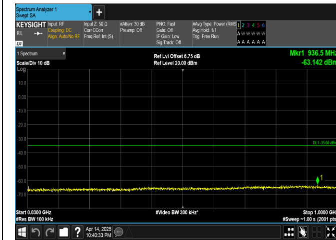
Band41-5MHz-QPSK-40620-1RB#24-30~1000-PASS
