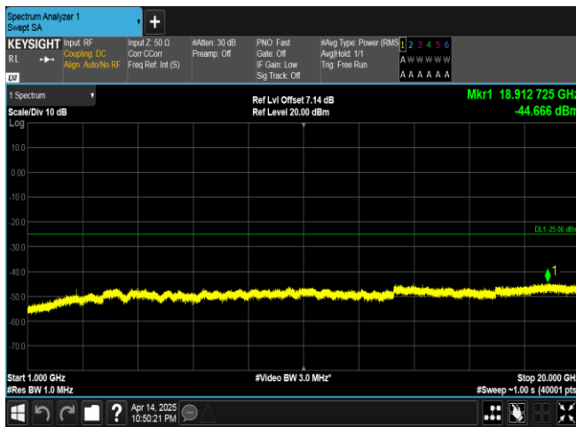
Band41-5MHz-16QAM-41565-25RB#0-1000~20000-PASS
