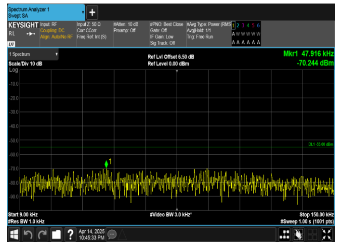
Band41-5MHz-16QAM-41565-1RB#0-0.009~0.15-PASS
