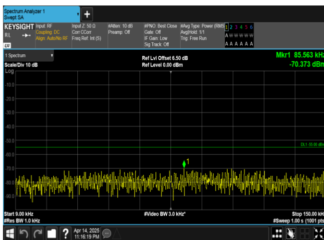
Band41-10MHz-QPSK-39700-1RB#0-0.009~0.15-PASS
