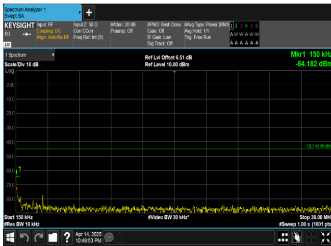
Band41-5MHz-16QAM-41565-25RB#0-0.15~30-PASS
