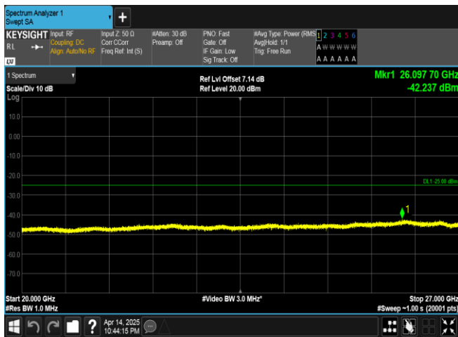
Band41-5MHz-16QAM-40620-25RB#0-20000~27000-PASS
