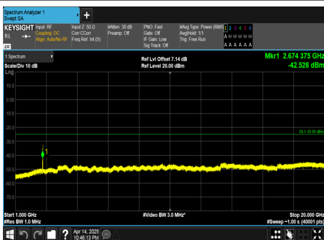
Band41-5MHz-16QAM-41565-1RB#0-1000~20000-PASS
