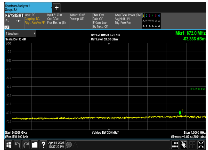
Band41-5MHz-16QAM-39675-25RB#0-30~1000-PASS
