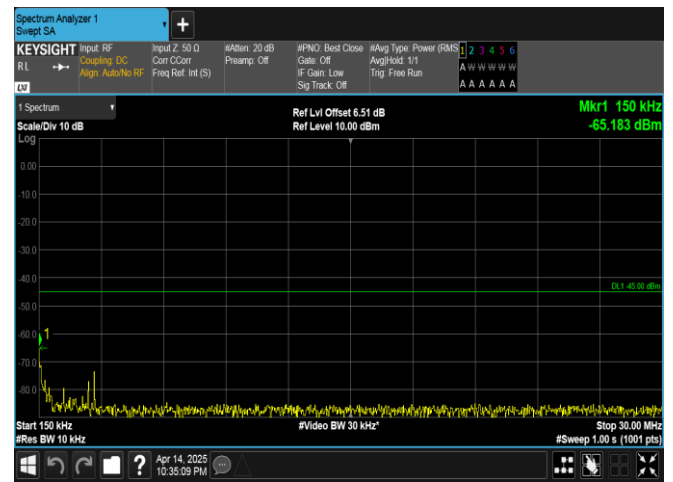
Band41-5MHz-16QAM-39675-1RB#24-0.15~30-PASS
