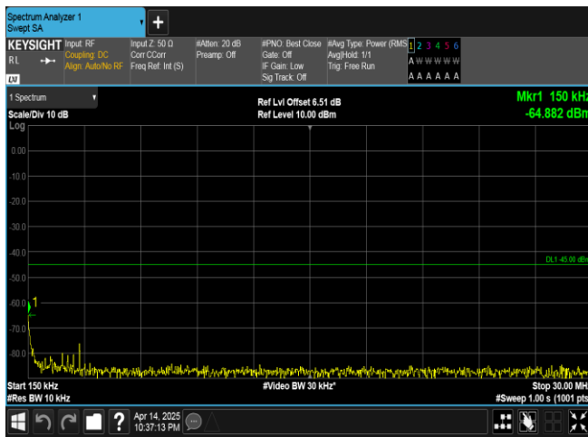
Band41-5MHz-16QAM-39675-25RB#0-0.15~30-PASS
