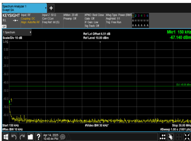
Band41-5MHz-16QAM-41565-1RB#0-0.15~30-PASS
