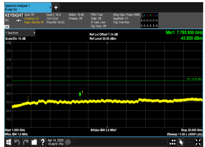
Band41-5MHz-QPSK-40620-1RB#24-1000~20000-PASS
