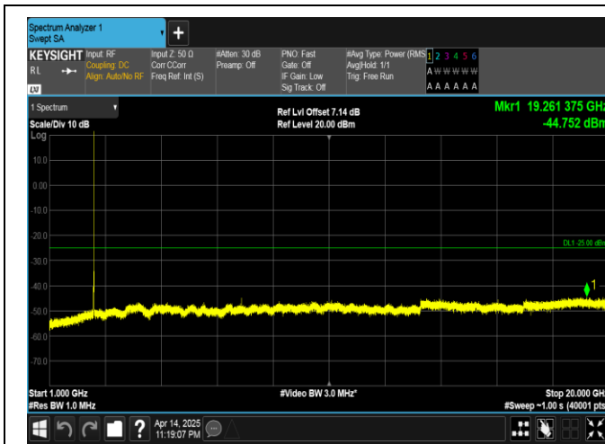
Band41-10MHz-QPSK-39700-1RB#49-1000~20000-PASS
