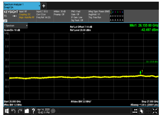
Band41-5MHz-16QAM-40620-1RB#24-20000~27000-PASS
