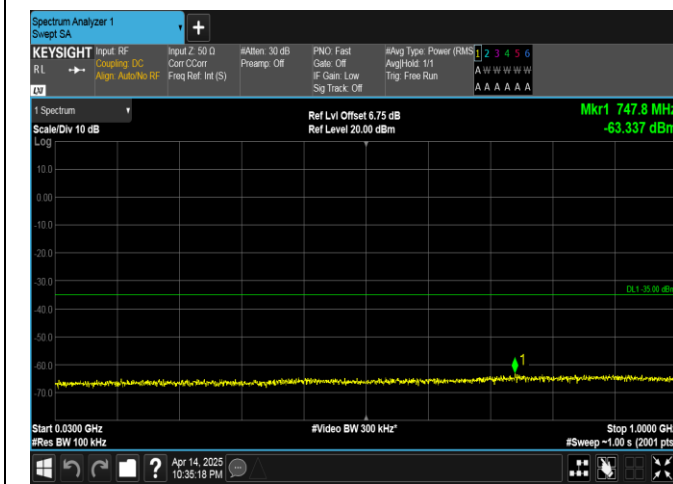
Band41-5MHz-16QAM-39675-1RB#24-30~1000-PASS
