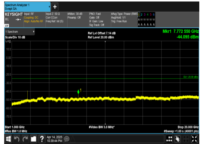
Band41-5MHz-16QAM-40620-1RB#0-1000~20000-PASS
