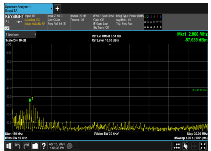
Band41-15MHz-16QAM-40620-75RB#0-0.15~30-PASS
