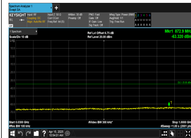
Band41-15MHz-16QAM-39725-1RB#74-30~1000-PASS
