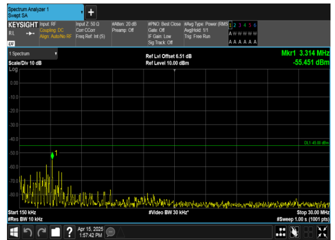
Band41-15MHz-QPSK-41515-75RB#0-0.15~30-PASS
