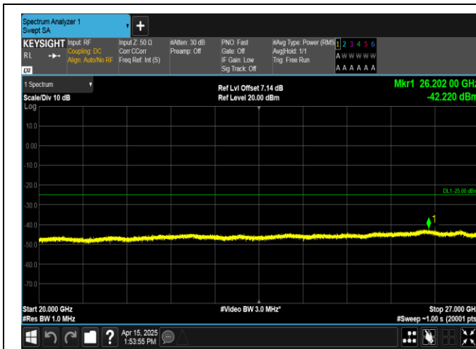
Band41-15MHz-QPSK-39725-75RB#0-20000~27000-PASS
