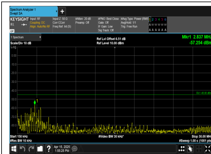
Band41-15MHz-QPSK-40620-75RB#0-0.15~30-PASS
