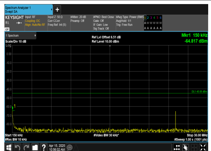
Band41-15MHz-16QAM-40620-1RB#0-0.15~30-PASS
