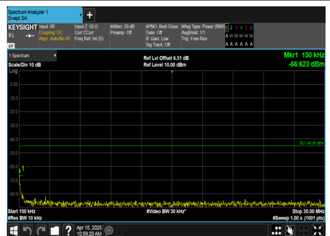
Band41-15MHz-QPSK-41515-1RB#0-0.15~30-PASS
