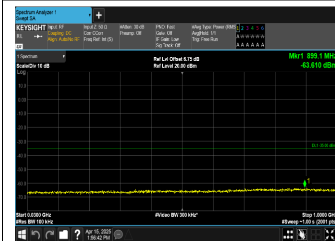
Band41-15MHz-16QAM-40620-75RB#0-30~1000-PASS
