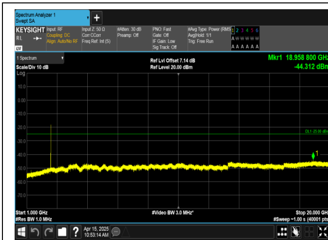
Band41-15MHz-QPSK-39725-1RB#74-1000~20000-PASS
