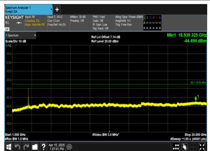
Band41-15MHz-16QAM-40620-75RB#0-1000~20000-PASS
