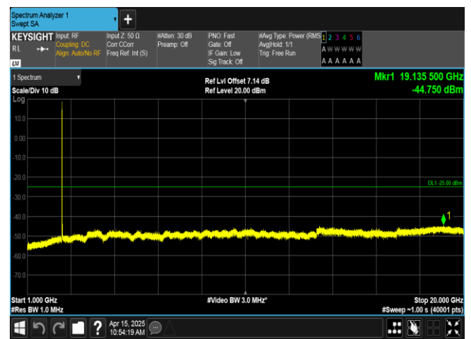
Band41-15MHz-16QAM-39725-1RB#74-1000~20000-PASS
