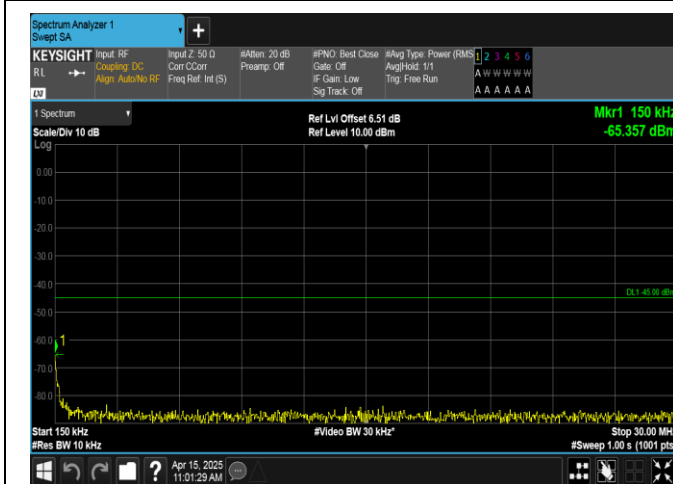
Band41-15MHz-QPSK-41515-1RB#74-0.15~30-PASS
