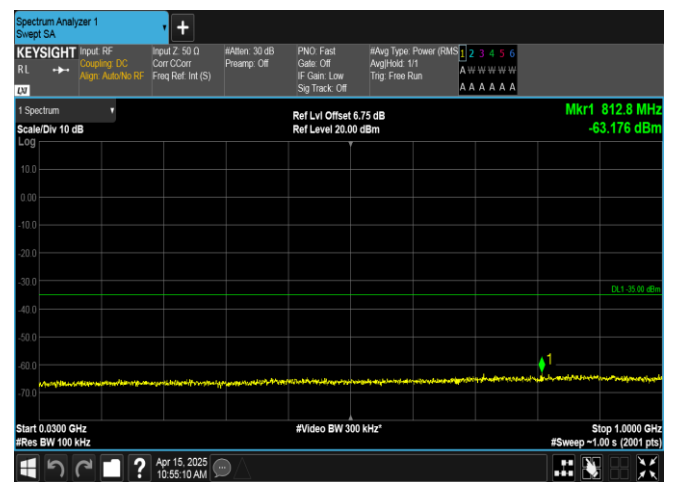
Band41-15MHz-QPSK-40620-1RB#0-30~1000-PASS
