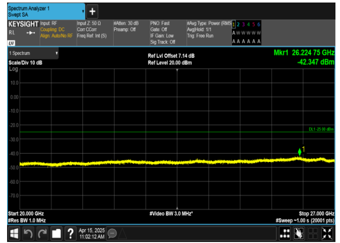
Band41-15MHz-QPSK-41515-1RB#74-20000~27000-PASS
