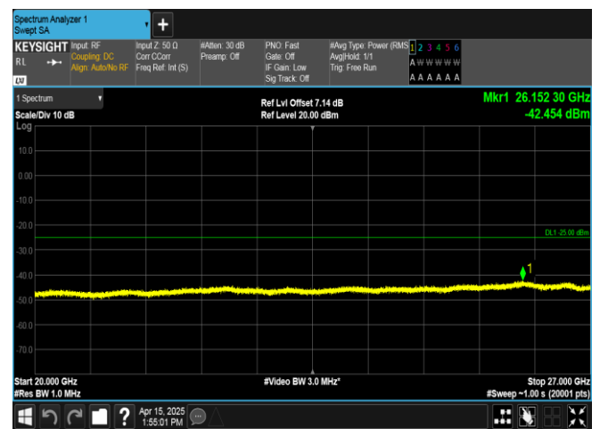
Band41-15MHz-16QAM-39725-75RB#0-20000~27000-PASS
