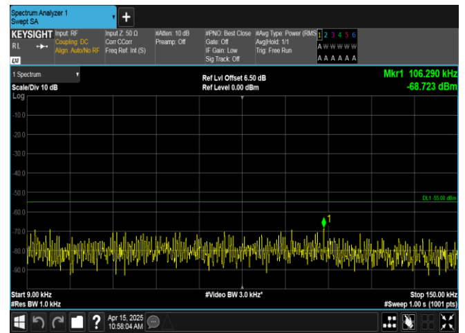
Band41-15MHz-16QAM-40620-1RB#74-0.009~0.15-PASS
