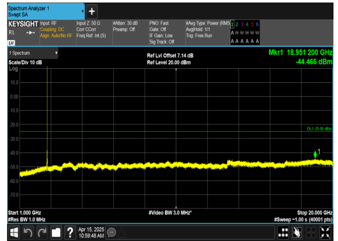
Band41-15MHz-QPSK-41515-1RB#0-1000~20000-PASS
