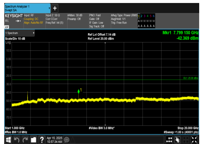
Band41-15MHz-QPSK-40620-1RB#74-1000~20000-PASS
