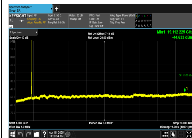
Band41-15MHz-16QAM-41515-1RB#0-1000~20000-PASS
