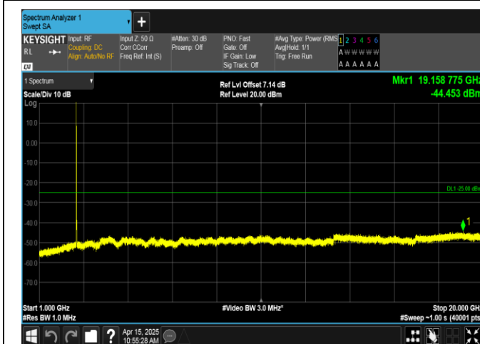
Band41-15MHz-QPSK-40620-1RB#0-1000~20000-PASS
