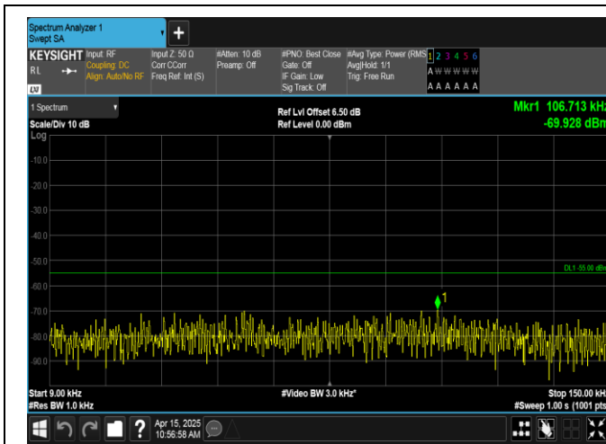
Band41-15MHz-QPSK-40620-1RB#74-0.009~0.15-PASS
