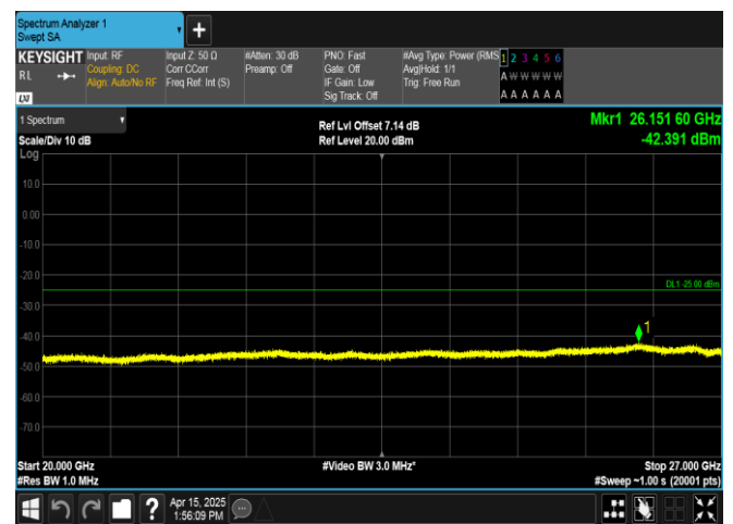
Band41-15MHz-QPSK-40620-75RB#0-20000~27000-PASS
