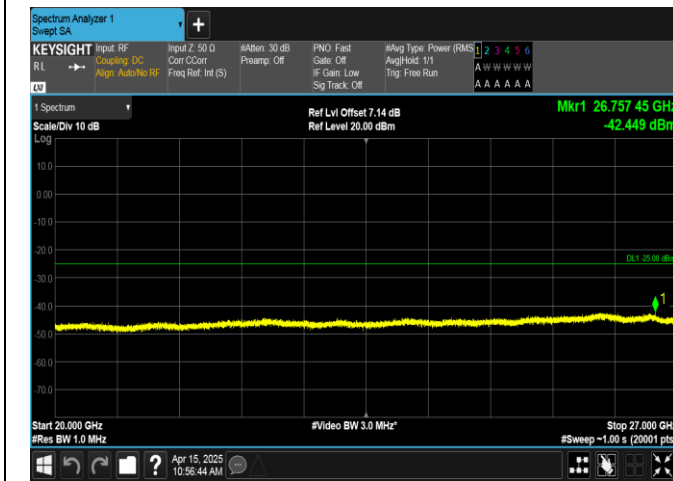
Band41-15MHz-16QAM-40620-1RB#0-20000~27000-PASS
