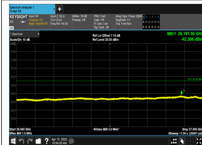
Band41-15MHz-16QAM-39725-1RB#74-20000~27000-PASS
