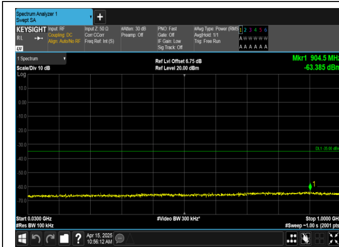
Band41-15MHz-16QAM-40620-1RB#0-30~1000-PASS
