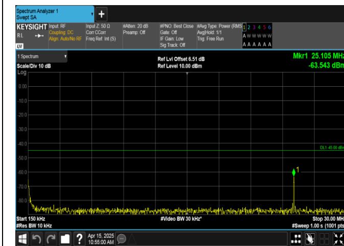
Band41-15MHz-QPSK-40620-1RB#0-0.15~30-PASS
