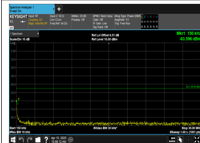
Band41-15MHz-16QAM-40620-1RB#74-0.15~30-PASS
