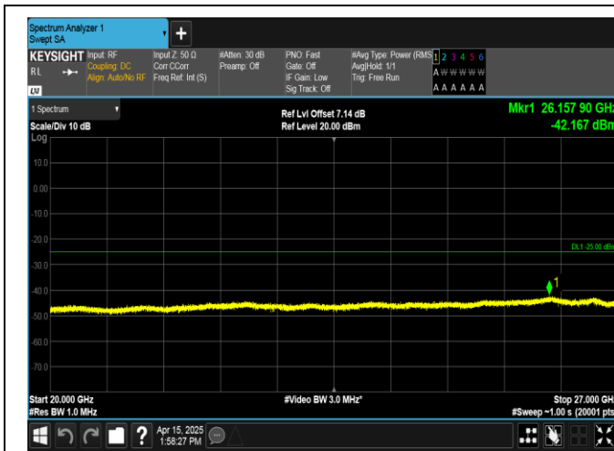
Band41-15MHz-QPSK-41515-75RB#0-20000~27000-PASS
