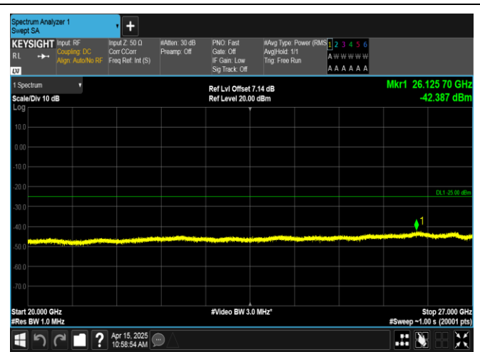
Band41-15MHz-16QAM-40620-1RB#74-20000~27000-PASS
