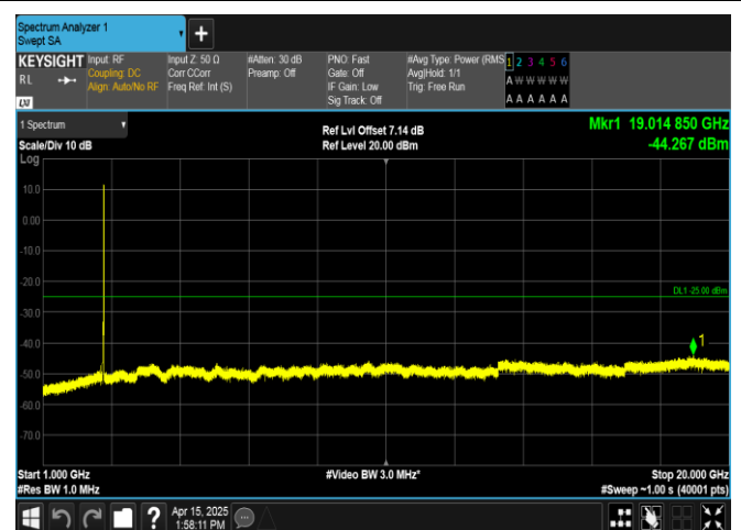
Band41-15MHz-QPSK-41515-75RB#0-1000~20000-PASS
