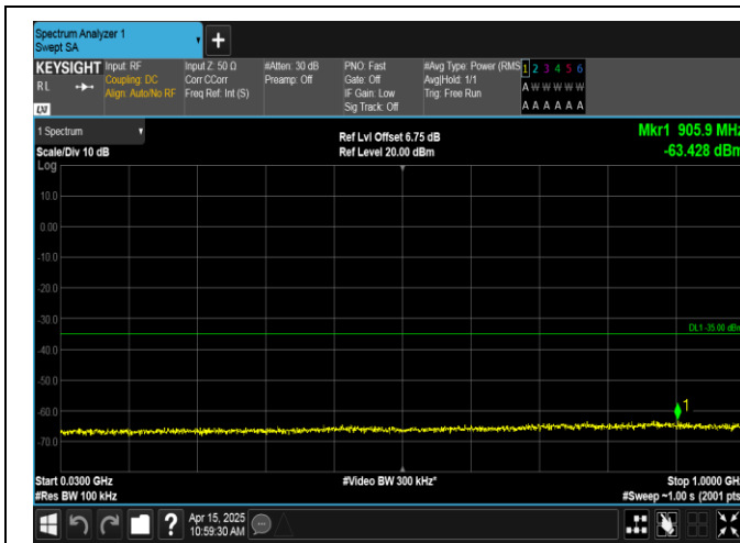
Band41-15MHz-QPSK-41515-1RB#0-30~1000-PASS
