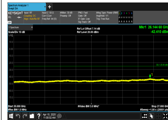
Band41-15MHz-QPSK-41515-1RB#0-20000~27000-PASS
