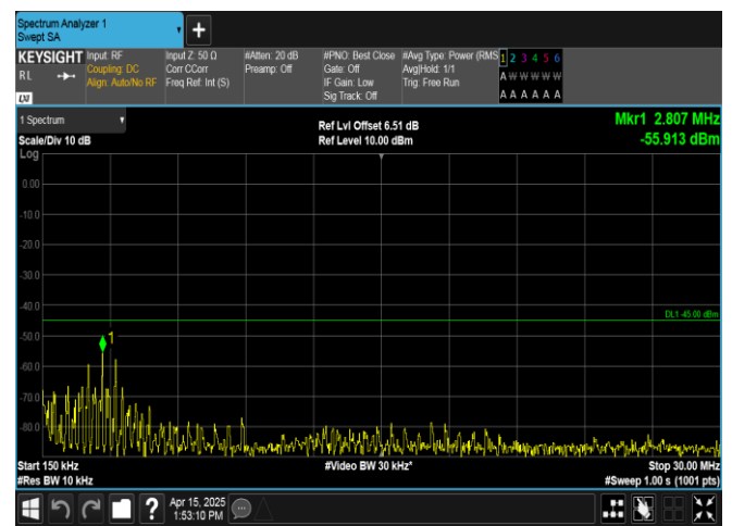
Band41-15MHz-QPSK-39725-75RB#0-0.15~30-PASS
