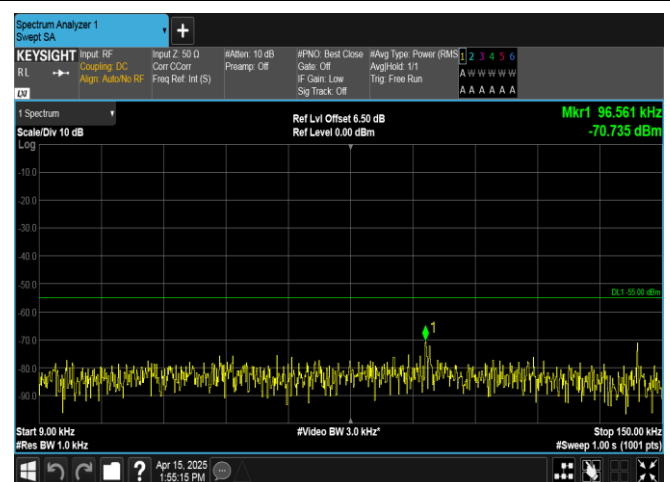
Band41-15MHz-QPSK-40620-75RB#0-0.009~0.15-PASS
