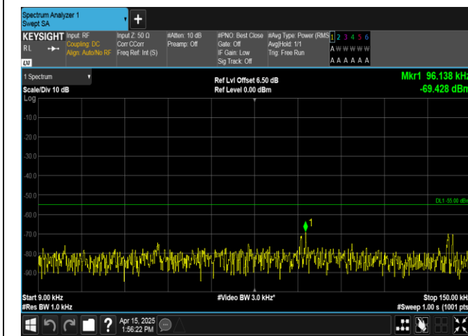
Band41-15MHz-16QAM-40620-75RB#0-0.009~0.15-PASS
