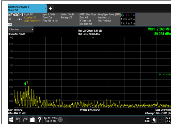
Band41-15MHz-16QAM-39725-75RB#0-0.15~30-PASS
