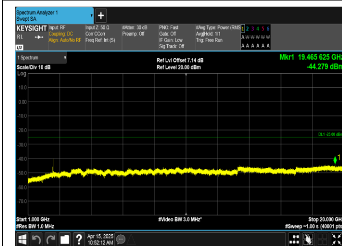
Band41-15MHz-16QAM-39725-1RB#0-1000~20000-PASS
