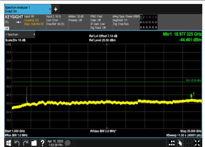
Band41-15MHz-QPSK-39725-75RB#0-1000~20000-PASS
