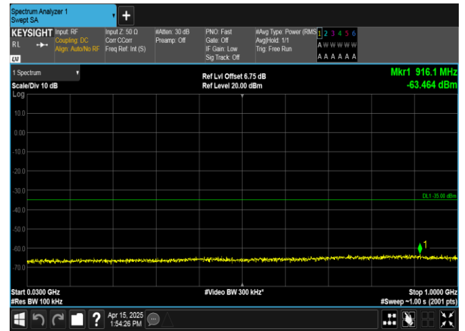
Band41-15MHz-16QAM-39725-75RB#0-30~1000-PASS
