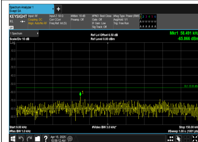
Band41-15MHz-QPSK-41515-1RB#0-0.009~0.15-PASS
