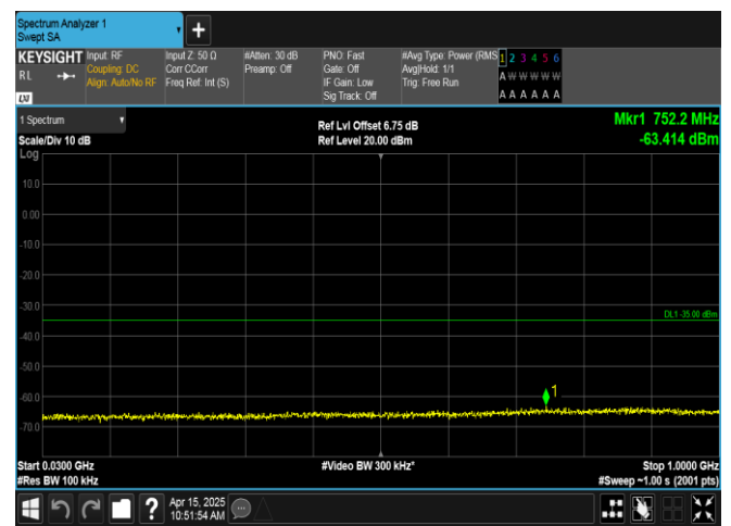
Band41-15MHz-16QAM-39725-1RB#0-30~1000-PASS
