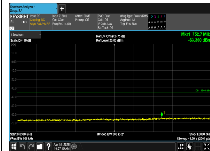
Band41-15MHz-QPSK-40620-1RB#74-30~1000-PASS
