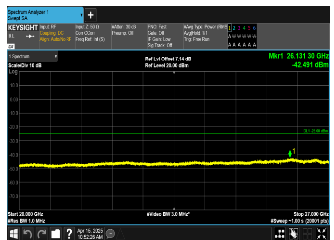
Band41-15MHz-16QAM-39725-1RB#0-20000~27000-PASS
