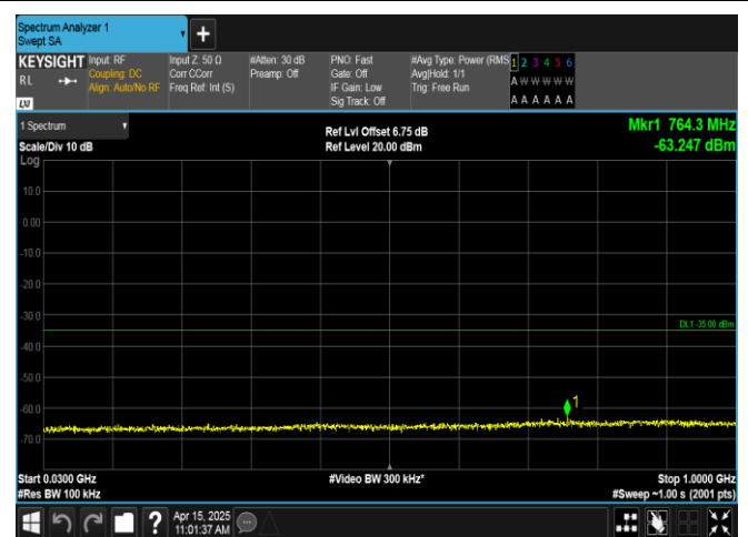
Band41-15MHz-QPSK-41515-1RB#74-30~1000-PASS
