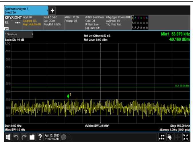
Band41-15MHz-16QAM-41515-1RB#0-0.009~0.15-PASS
