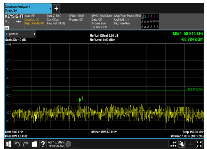
Band41-15MHz-QPSK-41515-1RB#74-0.009~0.15-PASS
