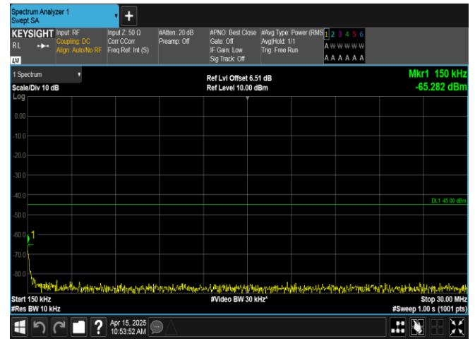
Band41-15MHz-16QAM-39725-1RB#74-0.15~30-PASS
