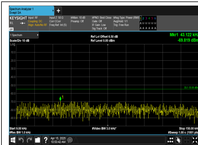
Band41-15MHz-16QAM-39725-1RB#74-0.009~0.15-PASS
