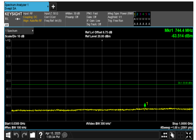
Band41-15MHz-QPSK-40620-75RB#0-30~1000-PASS
