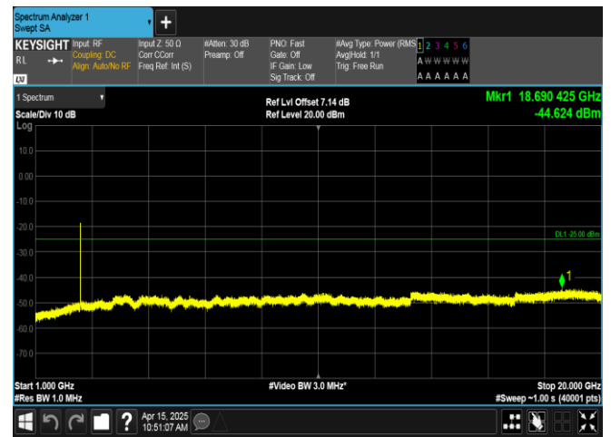
Band41-15MHz-QPSK-39725-1RB#0-1000~20000-PASS
