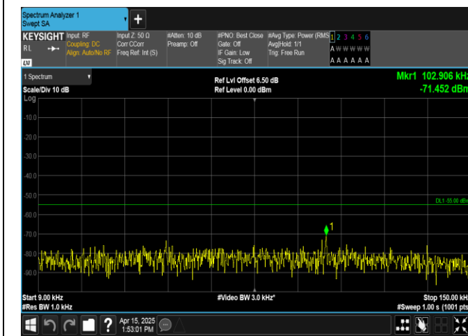
Band41-15MHz-QPSK-39725-75RB#0-0.009~0.15-PASS
