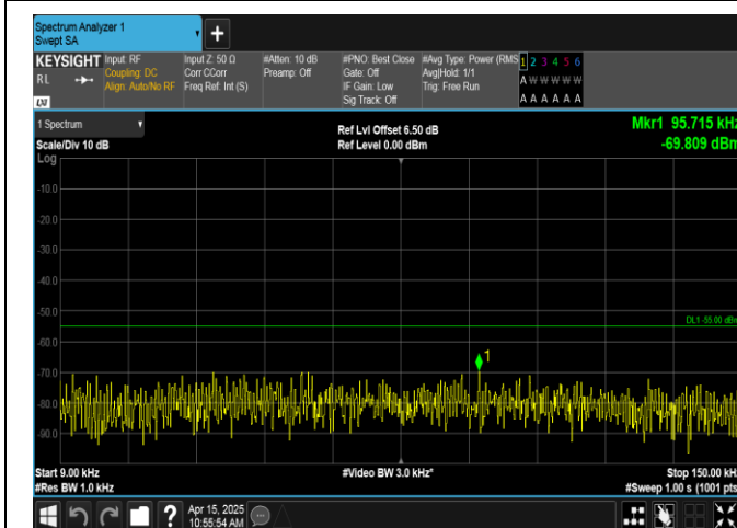
Band41-15MHz-16QAM-40620-1RB#0-0.009~0.15-PASS
