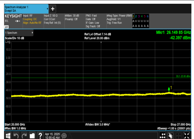
Band41-15MHz-QPSK-40620-1RB#0-20000~27000-PASS
