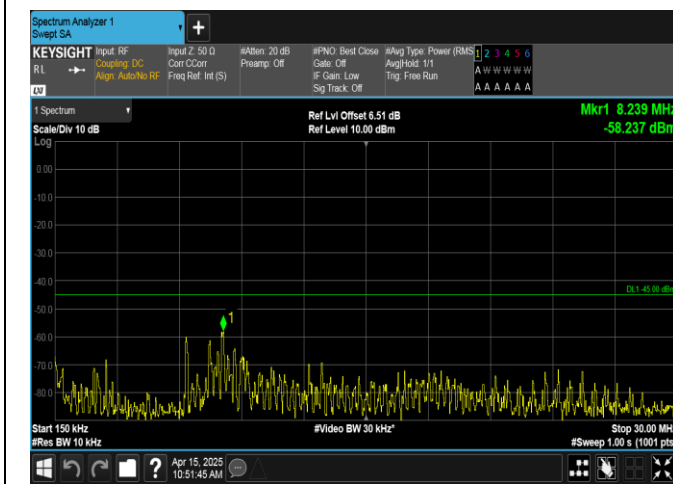
Band41-15MHz-16QAM-39725-1RB#0-0.15~30-PASS
