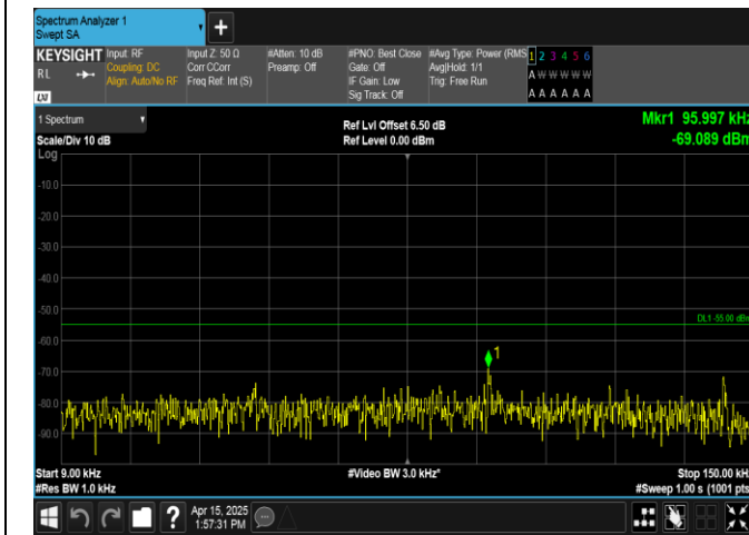
Band41-15MHz-QPSK-41515-75RB#0-0.009~0.15-PASS
