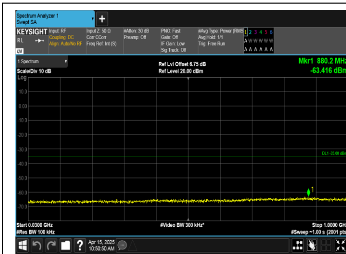
Band41-15MHz-QPSK-39725-1RB#0-30~1000-PASS
