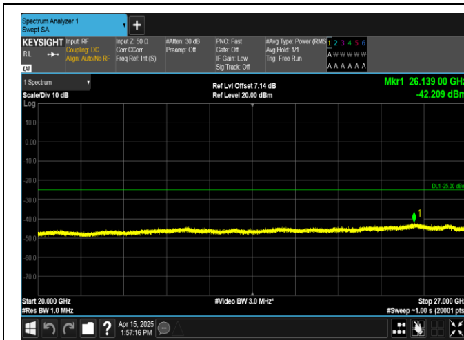
Band41-15MHz-16QAM-40620-75RB#0-20000~27000-PASS
