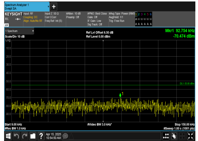
Band41-15MHz-QPSK-40620-1RB#0-0.009~0.15-PASS
