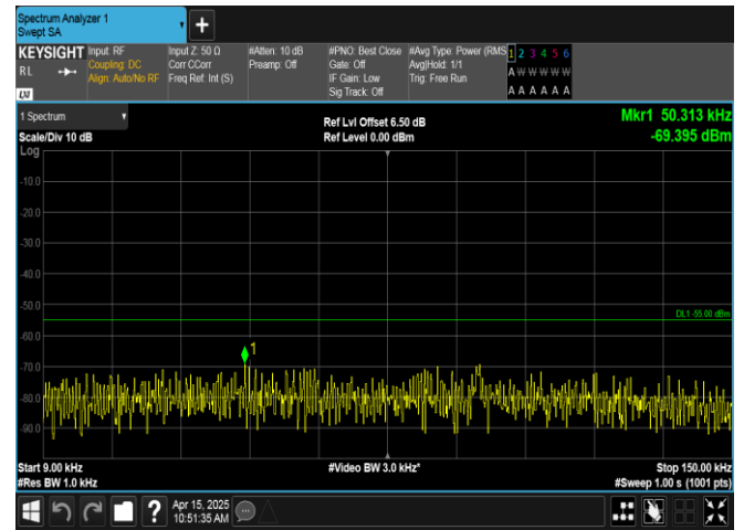
Band41-15MHz-16QAM-39725-1RB#0-0.009~0.15-PASS
