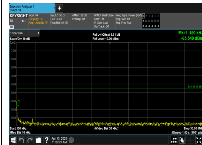
Band41-15MHz-16QAM-41515-1RB#0-0.15~30-PASS
