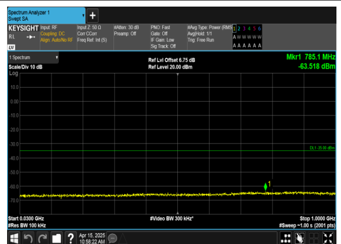
Band41-15MHz-16QAM-40620-1RB#74-30~1000-PASS
