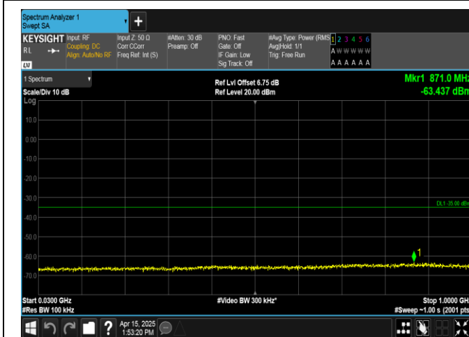
Band41-15MHz-QPSK-39725-75RB#0-30~1000-PASS
