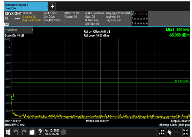
Band41-15MHz-QPSK-40620-1RB#74-0.15~30-PASS
