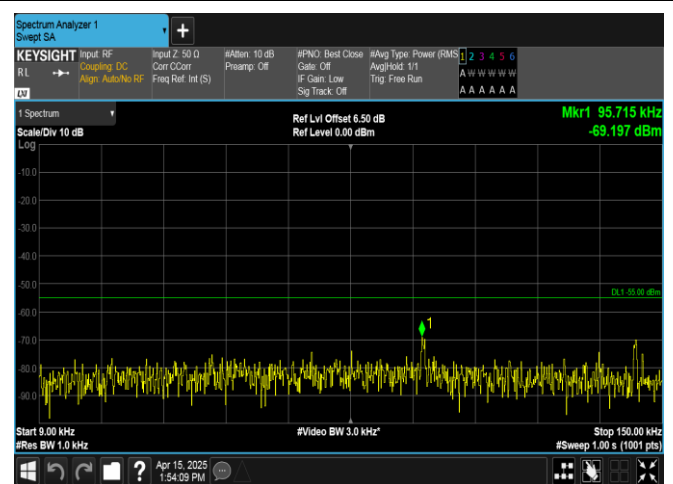
Band41-15MHz-16QAM-39725-75RB#0-0.009~0.15-PASS
