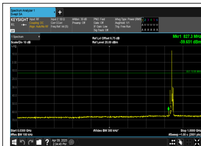
Band5-5MHz-QPSK-20625-1RB#0-30~1000-PASS
