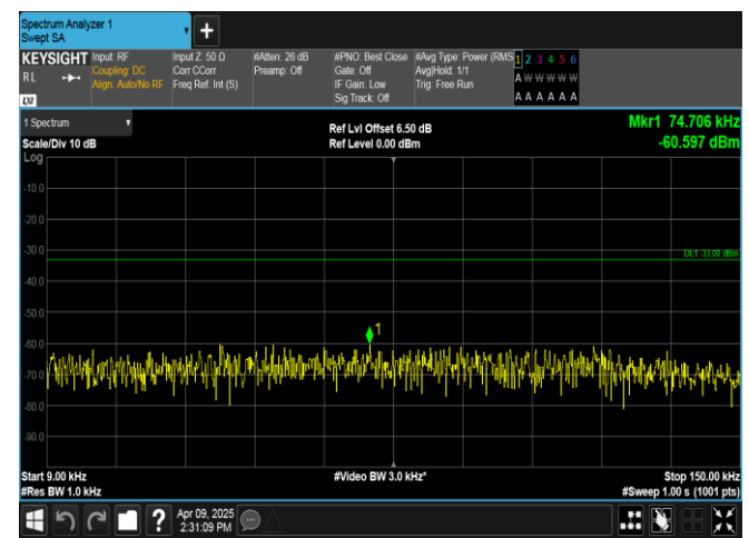
Band5-5MHz-16QAM-20525-1RB#24-0.009~0.15-PASS
