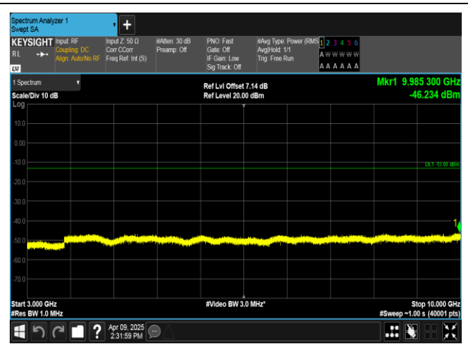
Band5-5MHz-16QAM-20525-1RB#24-3000~10000-PASS
