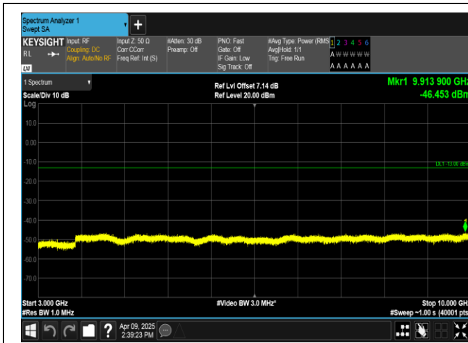
Band5-5MHz-QPSK-20625-25RB#0-3000~10000-PASS
