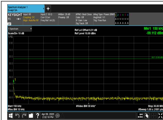
Band5-5MHz-QPSK-20525-25RB#0-0.15~30-PASS
