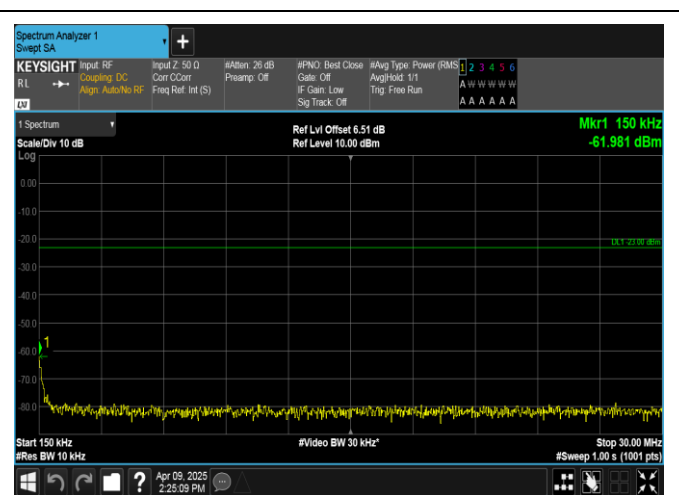
Band5-5MHz-16QAM-20425-1RB#24-0.15~30-PASS
