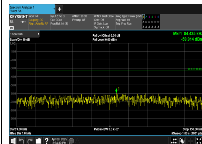
Band5-5MHz-QPSK-20625-1RB#0-0.009~0.15-PASS
