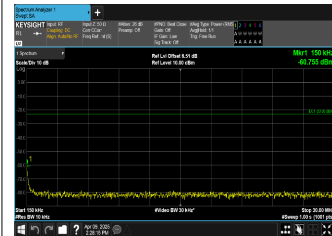
Band5-5MHz-QPSK-20525-1RB#0-0.15~30-PASS
