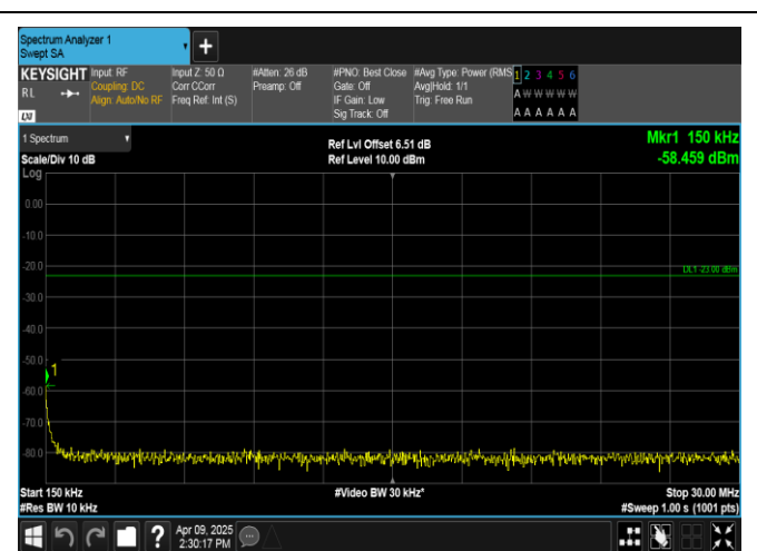
Band5-5MHz-QPSK-20525-1RB#24-0.15~30-PASS
