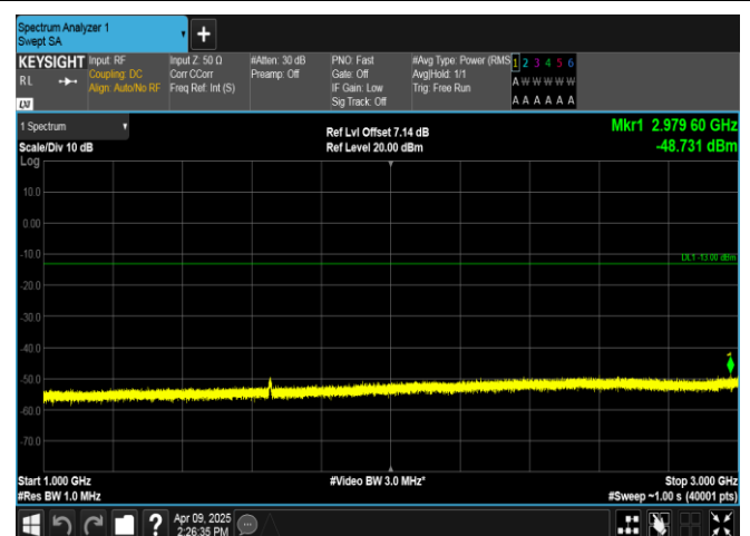
Band5-5MHz-QPSK-20425-25RB#0-1000~3000-PASS
