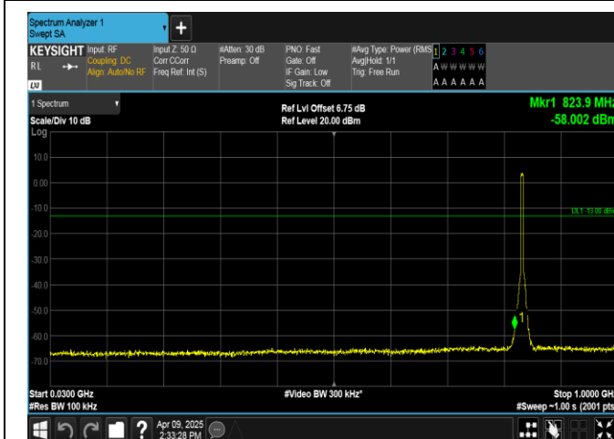
Band5-5MHz-16QAM-20525-25RB#0-30~1000-PASS
