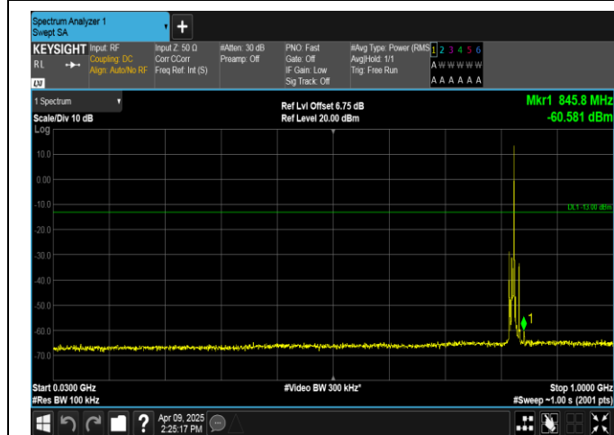
Band5-5MHz-16QAM-20425-1RB#24-30~1000-PASS
