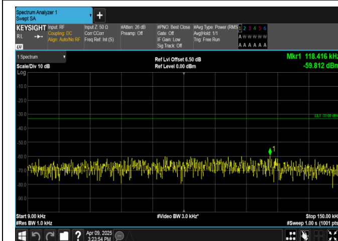
Band5-10MHz-QPSK-20450-1RB#0-0.009~0.15-PASS
