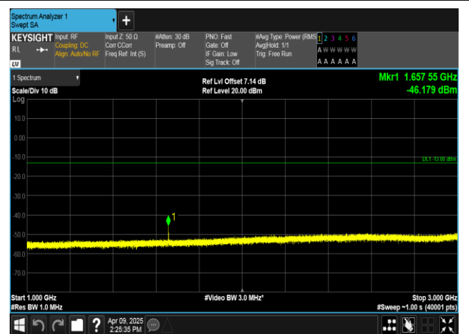
Band5-5MHz-16QAM-20425-1RB#24-1000~3000-PASS
