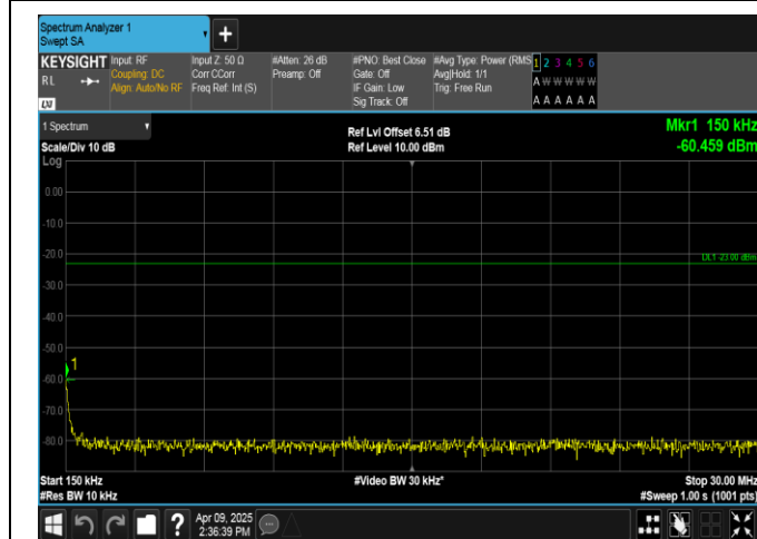
Band5-5MHz-QPSK-20625-1RB#24-0.15~30-PASS
