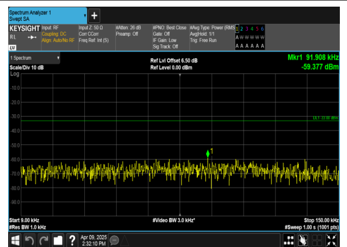
Band5-5MHz-QPSK-20525-25RB#0-0.009~0.15-PASS
