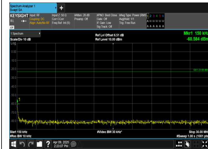
Band5-5MHz-16QAM-20425-1RB#0-0.15~30-PASS
