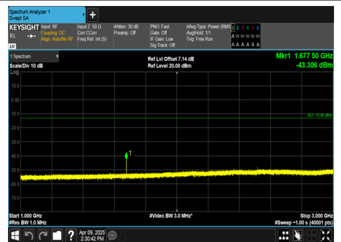
Band5-5MHz-QPSK-20525-1RB#24-1000~3000-PASS
