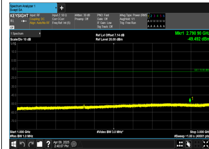
Band5-5MHz-16QAM-20625-25RB#0-1000~3000-PASS
