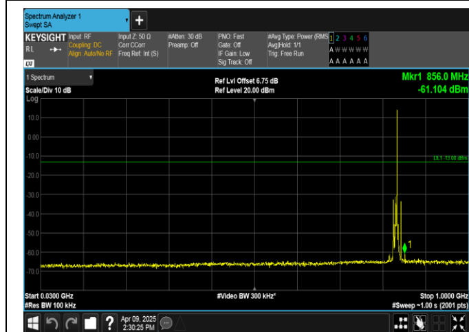
Band5-5MHz-QPSK-20525-1RB#24-30~1000-PASS
