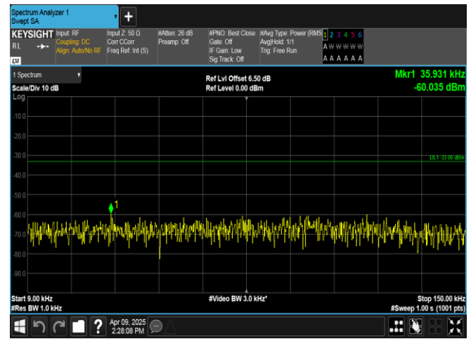
Band5-5MHz-QPSK-20525-1RB#0-0.009~0.15-PASS
