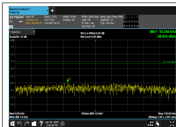
Band5-5MHz-QPSK-20525-1RB#24-0.009~0.15-PASS
