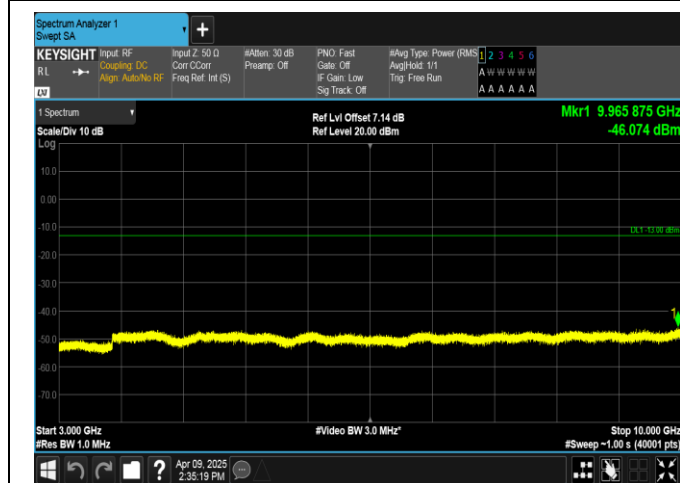
Band5-5MHz-QPSK-20625-1RB#0-3000~10000-PASS
