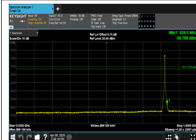
Band5-5MHz-QPSK-20425-25RB#0-30~1000-PASS
