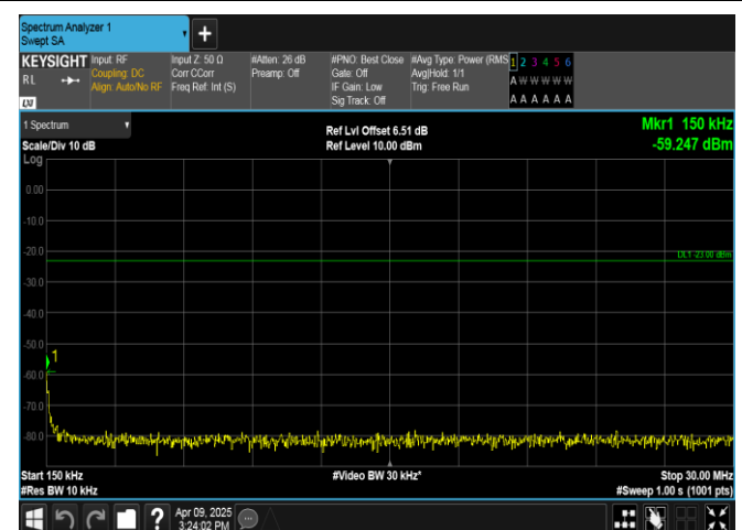
Band5-10MHz-QPSK-20450-1RB#0-0.15~30-PASS
