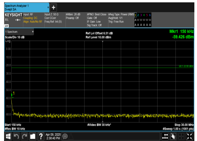
Band5-5MHz-QPSK-20625-25RB#0-0.15~30-PASS
