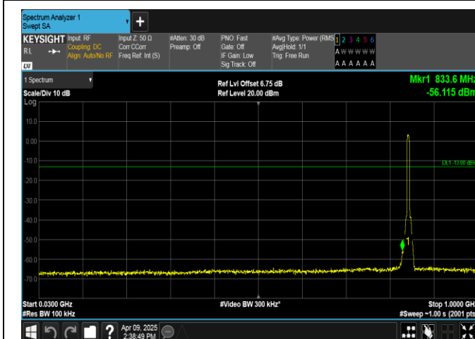
Band5-5MHz-QPSK-20625-25RB#0-30~1000-PASS
