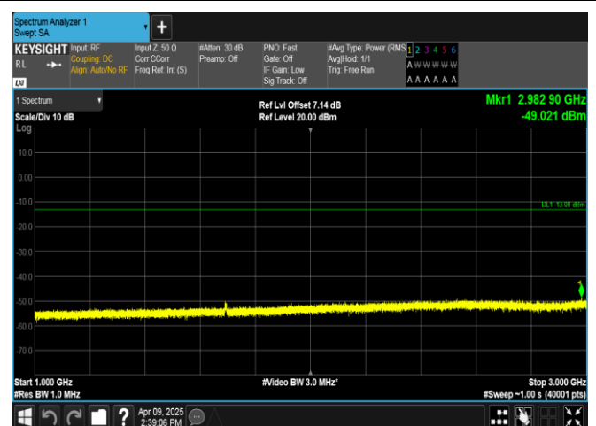
Band5-5MHz-QPSK-20625-25RB#0-1000~3000-PASS
