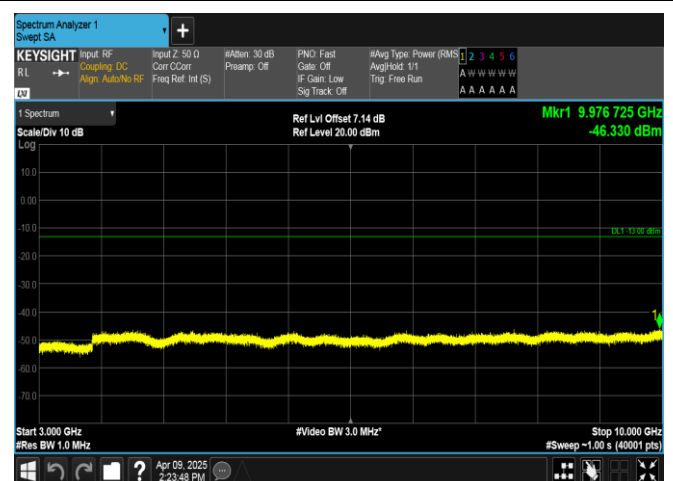
Band5-5MHz-16QAM-20425-1RB#0-3000~10000-PASS
