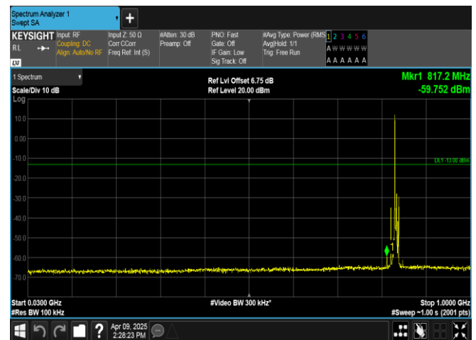
Band5-5MHz-QPSK-20525-1RB#0-30~1000-PASS
