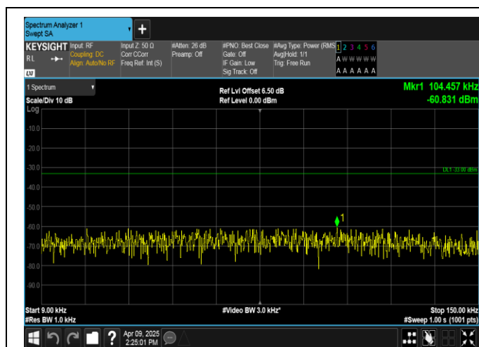
Band5-5MHz-16QAM-20425-1RB#24-0.009~0.15-PASS
