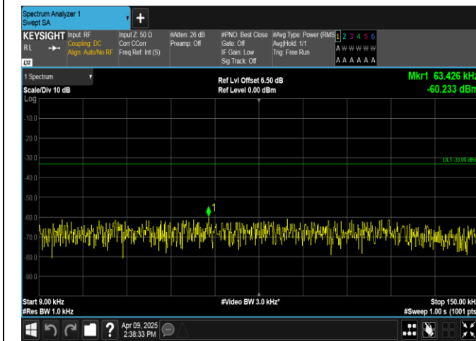
Band5-5MHz-QPSK-20625-25RB#0-0.009~0.15-PASS
