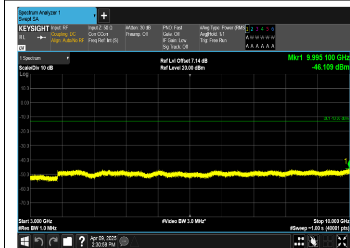
Band5-5MHz-QPSK-20525-1RB#24-3000~10000-PASS
