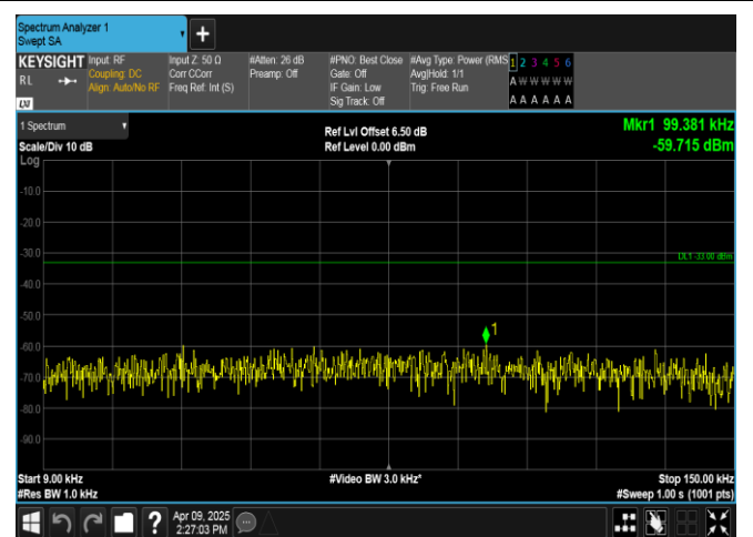
Band5-5MHz-16QAM-20425-25RB#0-0.009~0.15-PASS
