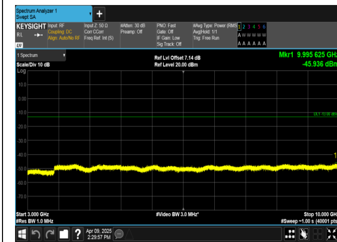
Band5-5MHz-16QAM-20525-1RB#0-3000~10000-PASS
