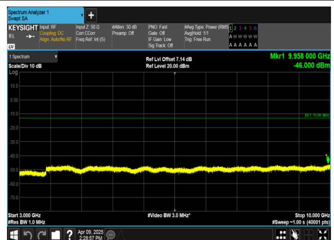
Band5-5MHz-QPSK-20525-1RB#0-3000~10000-PASS
