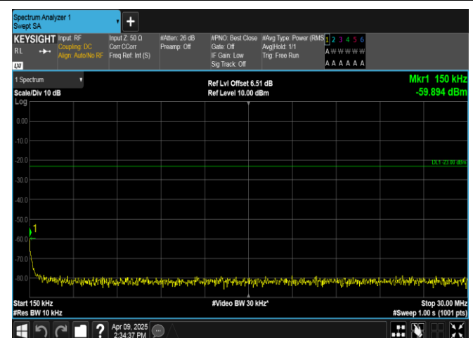
Band5-5MHz-QPSK-20625-1RB#0-0.15~30-PASS
