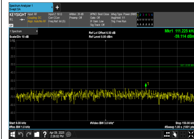
Band5-5MHz-QPSK-20425-25RB#0-0.009~0.15-PASS
