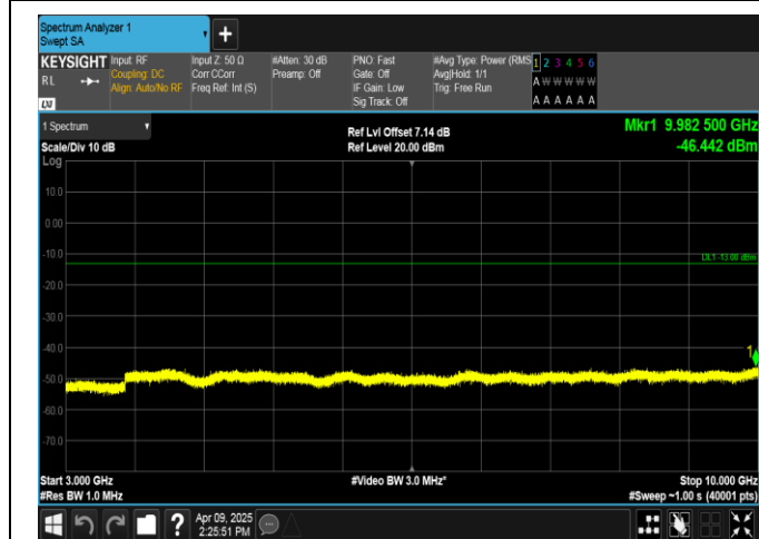
Band5-5MHz-16QAM-20425-1RB#24-3000~10000-PASS
