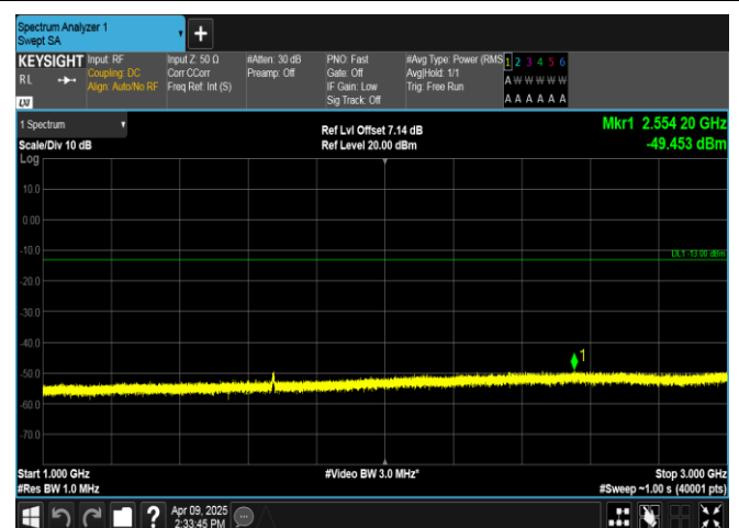
Band5-5MHz-16QAM-20525-25RB#0-1000~3000-PASS
