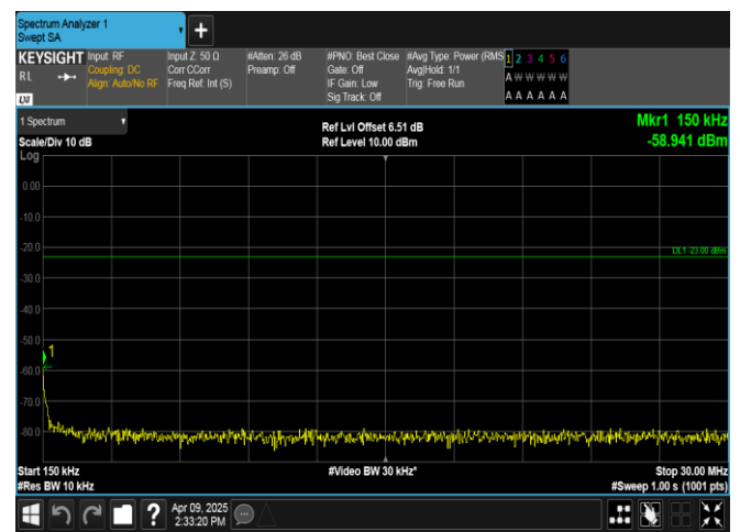
Band5-5MHz-16QAM-20525-25RB#0-0.15~30-PASS
