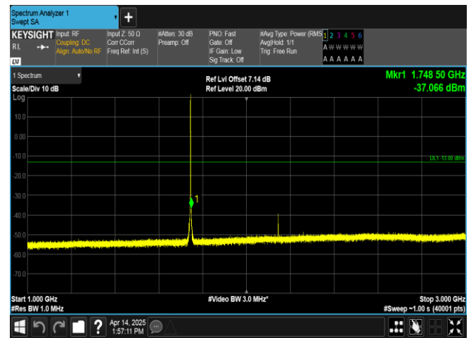
Band66-1.4MHz-16QAM-132322-1RB#0-1000~3000-PASS
