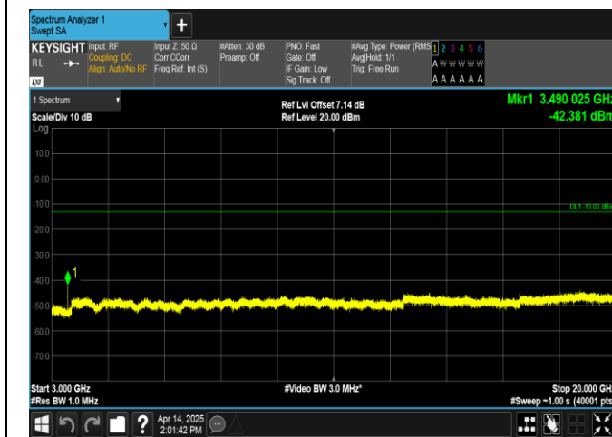
Band66-1.4MHz-16QAM-132322-6RB#0-3000~20000-PASS
