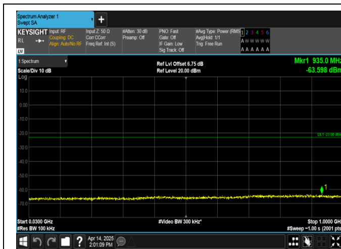
Band66-1.4MHz-16QAM-132322-6RB#0-30~1000-PASS
