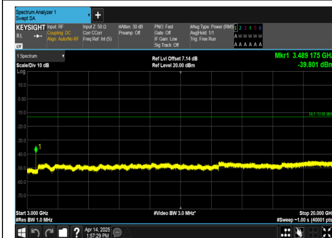
Band66-1.4MHz-16QAM-132322-1RB#0-3000~20000-PASS
