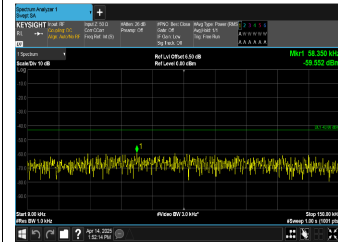
Band66-1.4MHz-16QAM-131979-1RB#5-0.009~0.15-PASS
