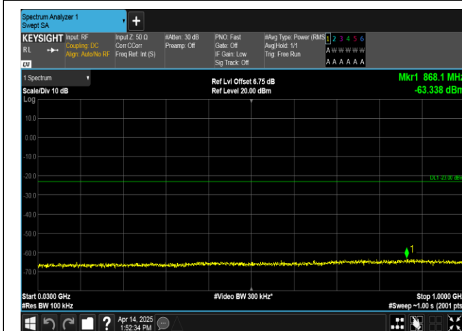
Band66-1.4MHz-16QAM-131979-1RB#5-30~1000-PASS
