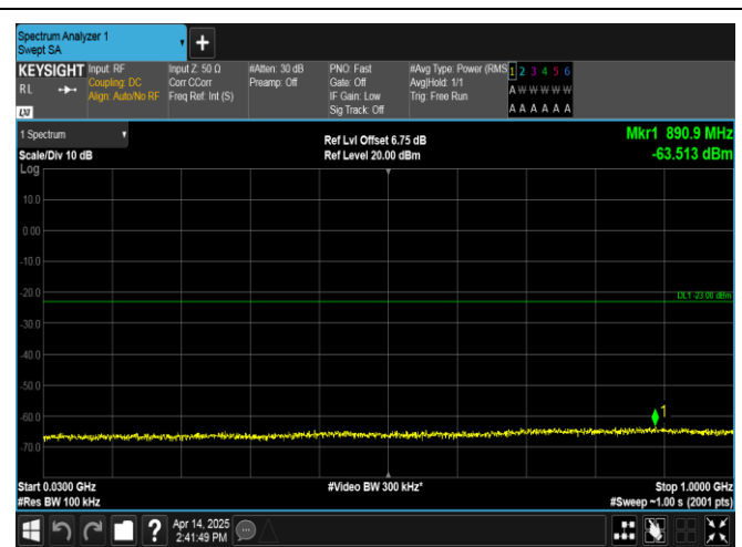
Band66-3MHz-QPSK-131987-1RB#14-30~1000-PASS
