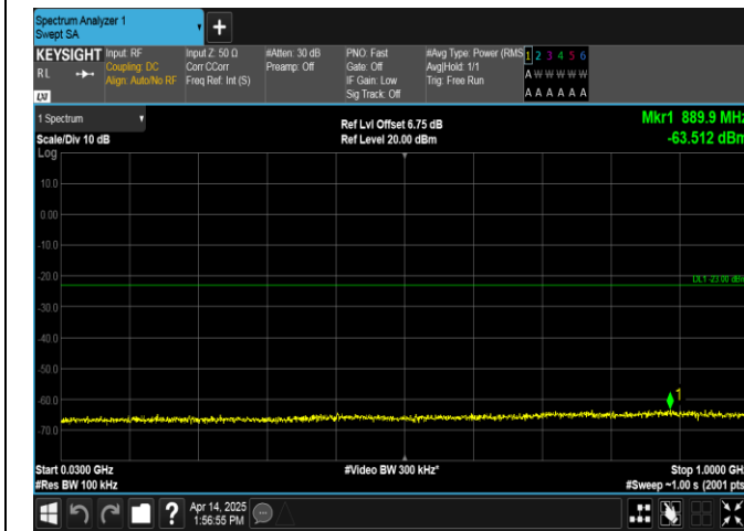
Band66-1.4MHz-16QAM-132322-1RB#0-30~1000-PASS
