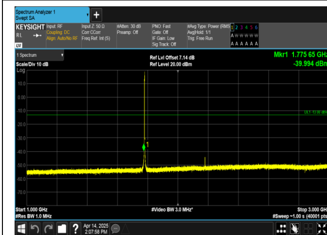
Band66-1.4MHz-16QAM-132665-6RB#0-1000~3000-PASS
