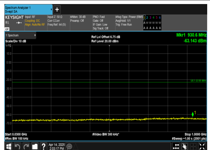
Band66-1.4MHz-16QAM-132665-1RB#0-30~1000-PASS
