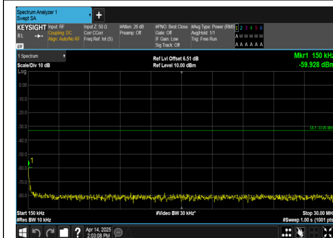
Band66-1.4MHz-16QAM-132665-1RB#0-0.15~30-PASS
