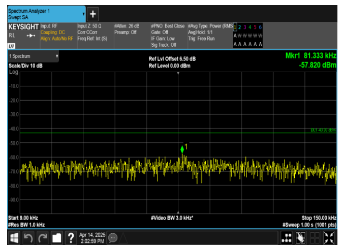
Band66-1.4MHz-16QAM-132665-1RB#0-0.009~0.15-PASS
