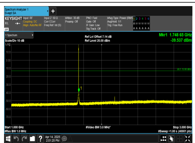
Band66-1.4MHz-16QAM-132322-6RB#0-1000~3000-PASS
