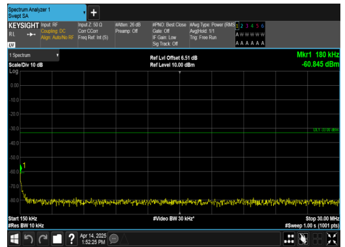
Band66-1.4MHz-16QAM-131979-1RB#5-0.15~30-PASS
