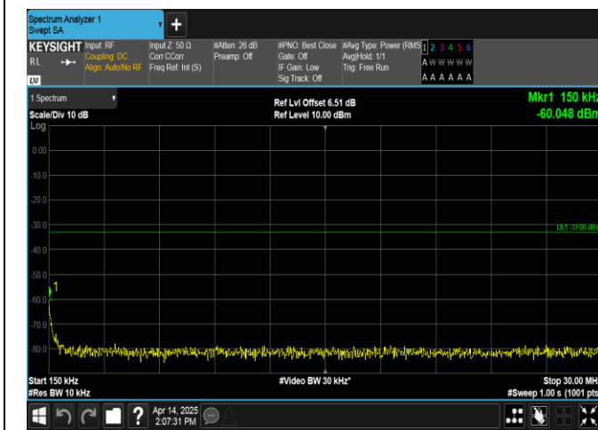
Band66-1.4MHz-16QAM-132665-6RB#0-0.15~30-PASS
