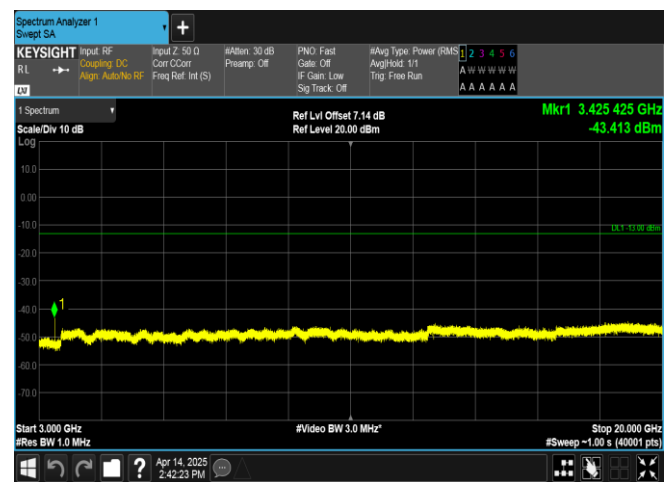
Band66-3MHz-QPSK-131987-1RB#14-3000~20000-PASS
