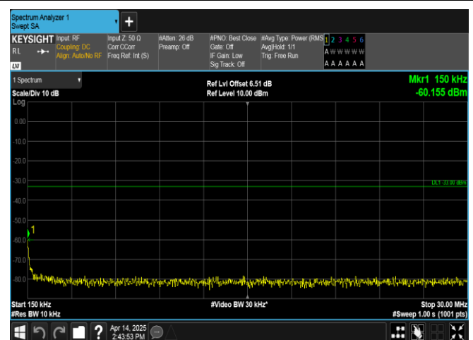
Band66-3MHz-QPSK-131987-15RB#0-0.15~30-PASS
