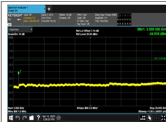
Band66-1.4MHz-16QAM-132665-1RB#5-3000~20000-PASS
