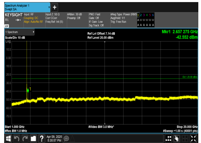
Band7-5MHz-16QAM-21100-1RB#0-1000~20000-PASS
