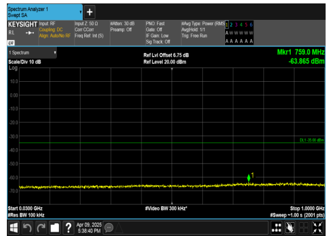
Band7-5MHz-QPSK-21100-25RB#0-30~1000-PASS
