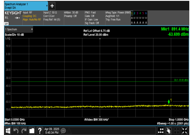
Band7-5MHz-16QAM-21425-25RB#0-30~1000-PASS
