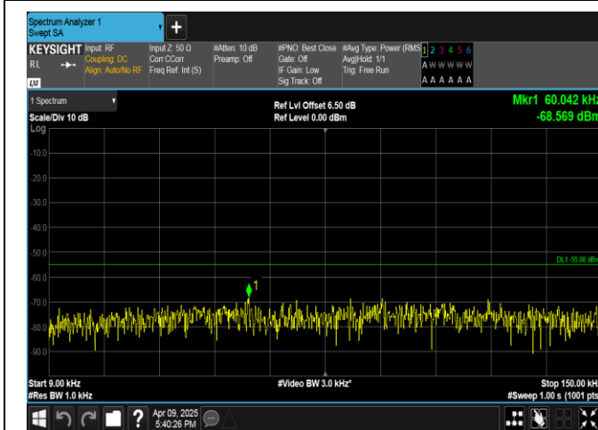
Band7-5MHz-QPSK-21425-1RB#0-0.009~0.15-PASS
