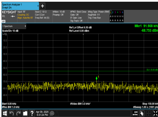
Band7-5MHz-16QAM-20775-1RB#24-0.009~0.15-PASS
