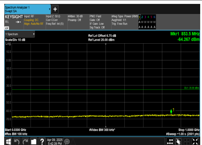
Band7-5MHz-QPSK-21425-1RB#24-30~1000-PASS
