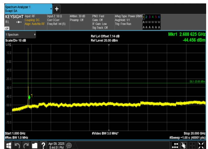
Band7-5MHz-QPSK-21425-25RB#0-1000~20000-PASS
