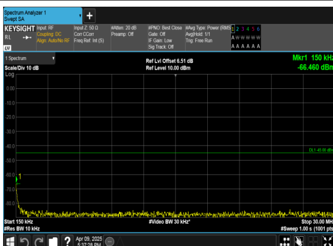
Band7-5MHz-16QAM-21100-1RB#24-0.15~30-PASS
