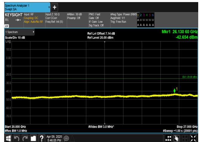
Band7-5MHz-16QAM-21425-25RB#0-20000~27000-PASS
