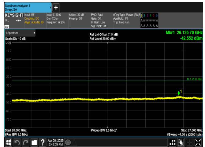
Band7-5MHz-QPSK-21425-1RB#24-20000~27000-PASS
