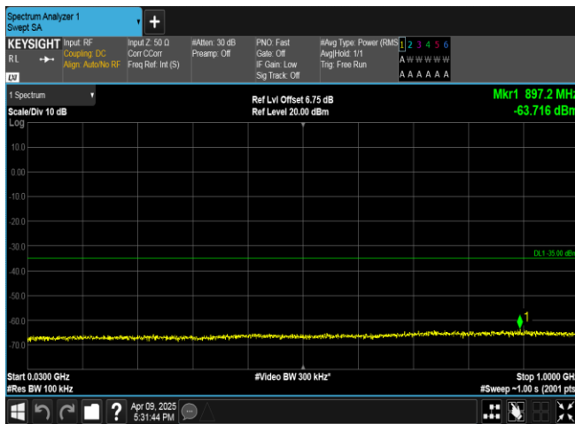
Band7-5MHz-16QAM-20775-1RB#24-30~1000-PASS
