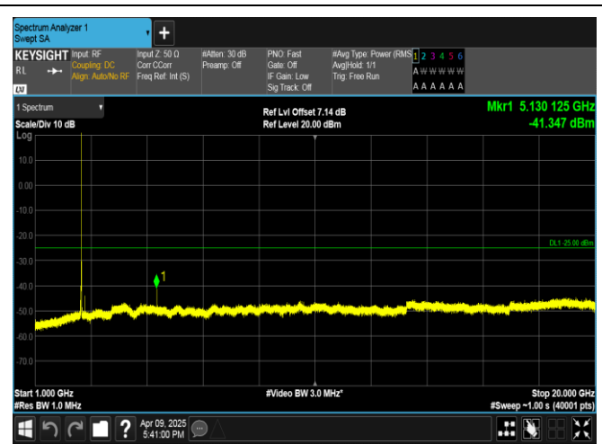
Band7-5MHz-QPSK-21425-1RB#0-1000~20000-PASS
