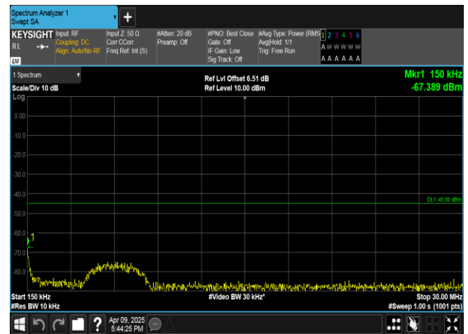
Band7-5MHz-QPSK-21425-25RB#0-0.15~30-PASS
