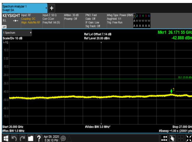
Band7-5MHz-16QAM-21100-1RB#0-20000~27000-PASS
