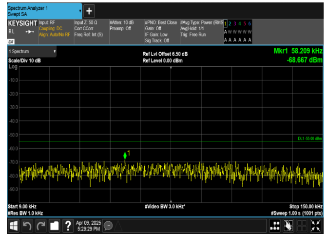
Band7-5MHz-16QAM-20775-1RB#0-0.009~0.15-PASS
