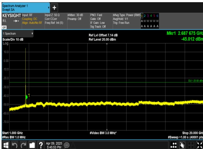
Band7-5MHz-16QAM-21425-25RB#0-1000~20000-PASS
