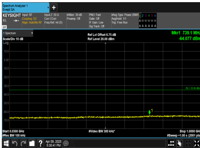
Band7-5MHz-16QAM-21100-1RB#0-30~1000-PASS
