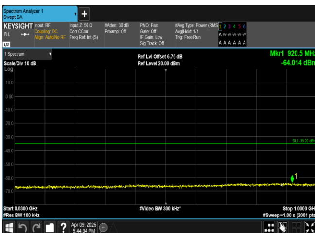
Band7-5MHz-QPSK-21425-25RB#0-30~1000-PASS
