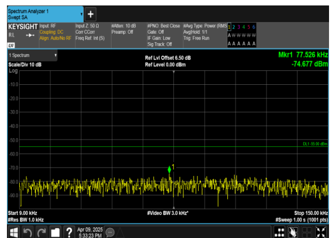
Band7-5MHz-16QAM-20775-25RB#0-0.009~0.15-PASS
