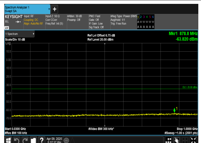
Band7-5MHz-16QAM-21100-1RB#24-30~1000-PASS
