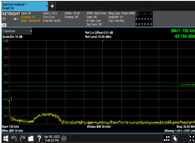
Band7-5MHz-16QAM-21425-25RB#0-0.15~30-PASS
