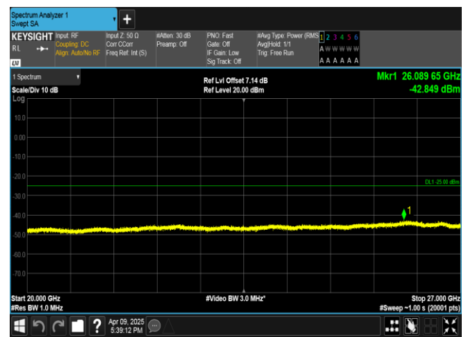
Band7-5MHz-QPSK-21100-25RB#0-20000~27000-PASS
