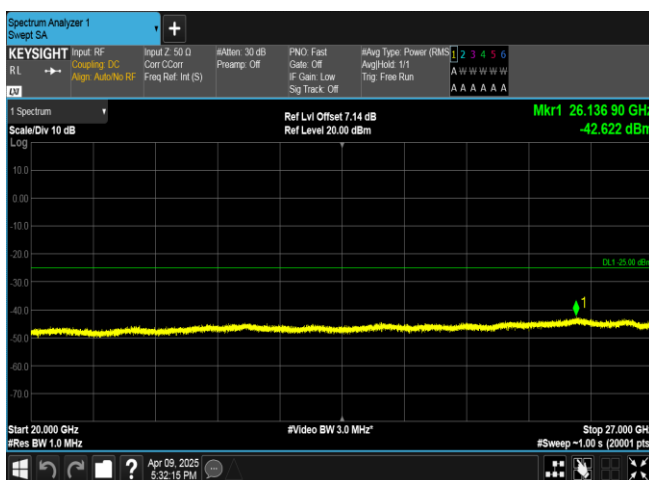
Band7-5MHz-16QAM-20775-1RB#24-20000~27000-PASS
