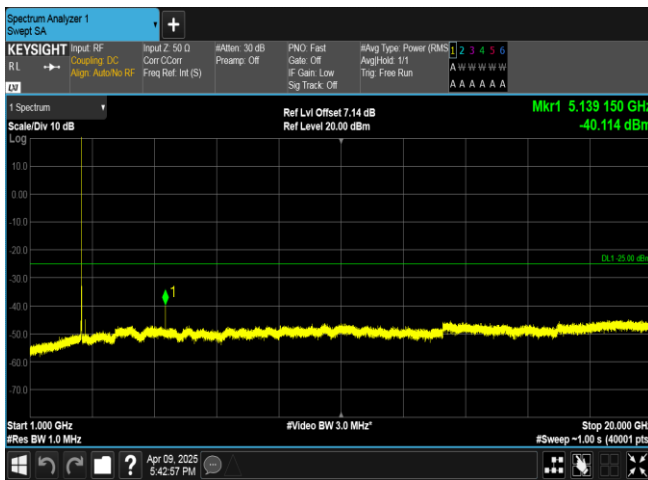
Band7-5MHz-QPSK-21425-1RB#24-1000~20000-PASS
