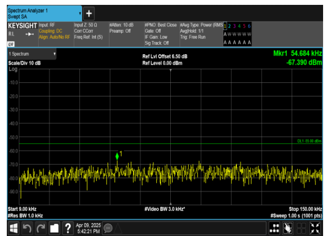
Band7-5MHz-QPSK-21425-1RB#24-0.009~0.15-PASS
