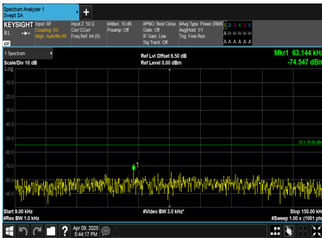
Band7-5MHz-QPSK-21425-25RB#0-0.009~0.15-PASS
