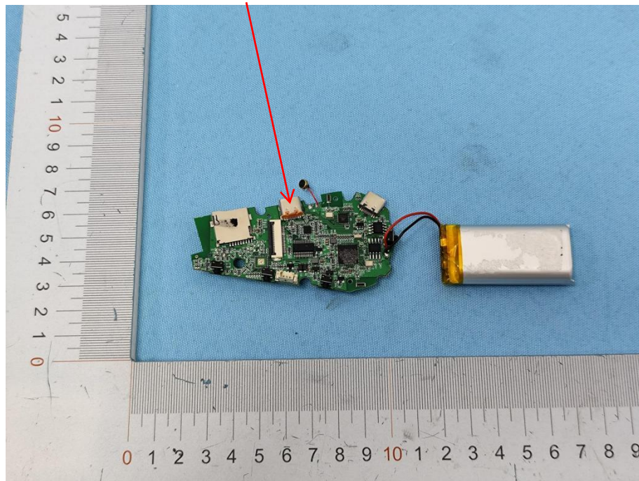
FM ANT port (Headphone jack)
