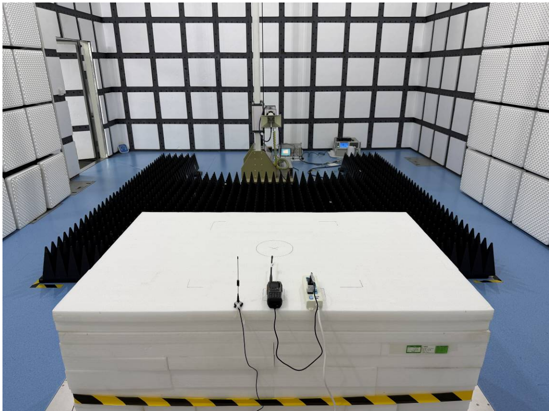
Radiation Emission -Back View (Above 1GHz)_Mode 3
