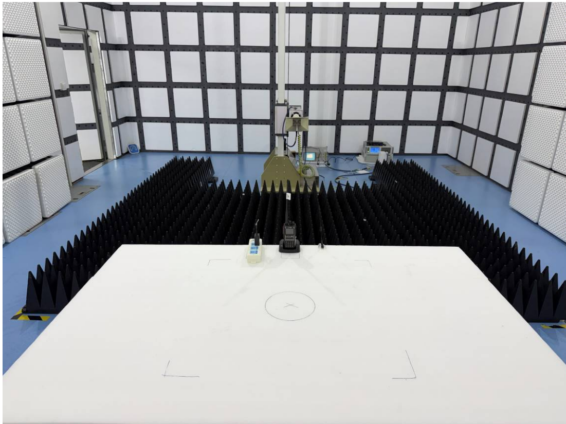
Radiation Emission -Back View (Above 1GHz) _Mode 4
