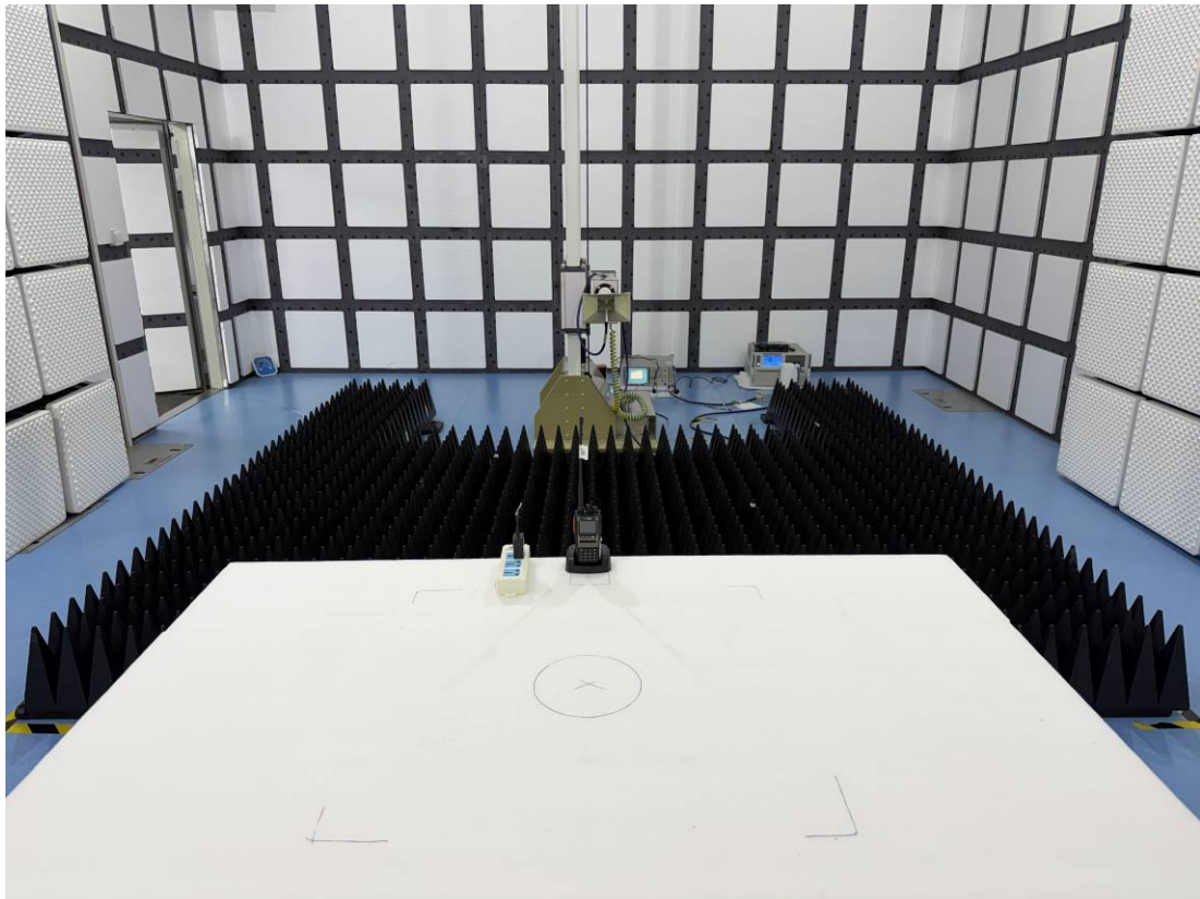
Radiation Emission -Back View (Above 1GHz)_Mode 2
