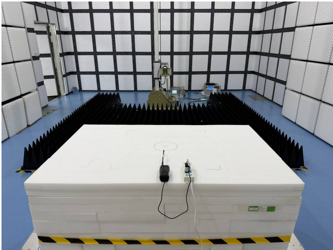
Radiation Emission – Back View (Above 1GHz) _Model1
