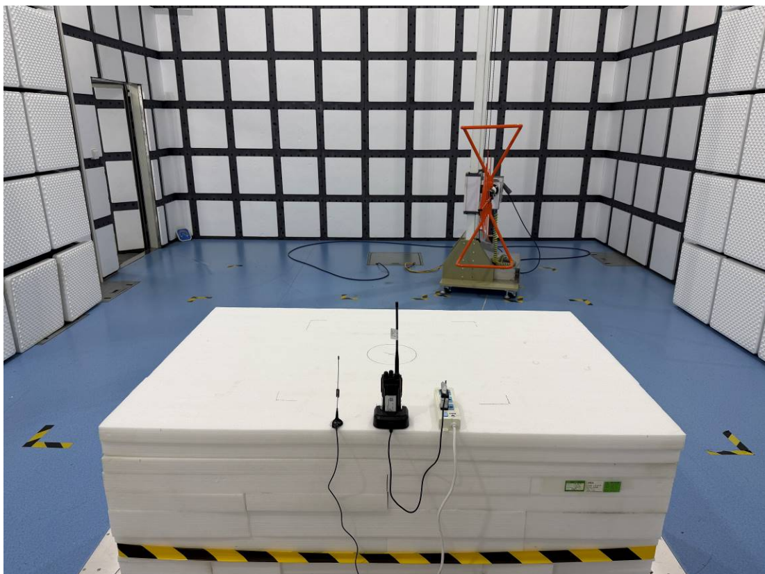
Radiation Emission - Back View (Below 1GHz)_Mode 4
