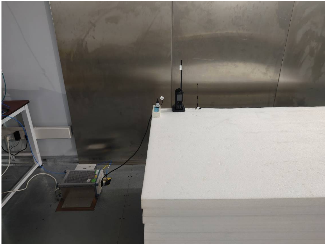
CE - Side View (Below 1GHz) – Mode 4
