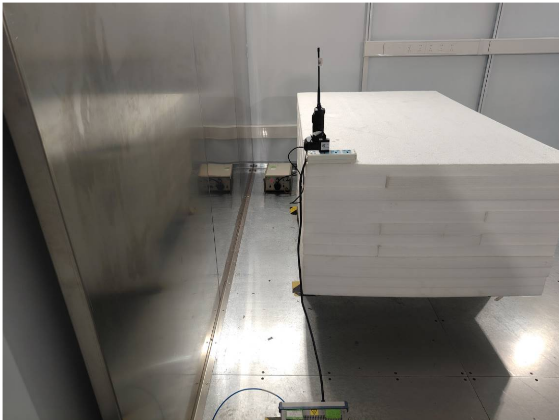
CE - Side View (Below 1GHz) – Mode 2
