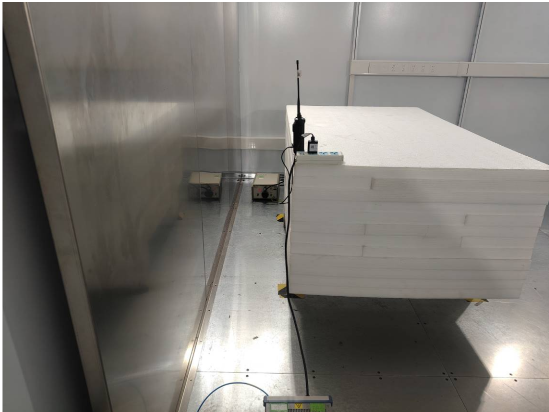
CE - Side View (Below 1GHz) – Mode 1
