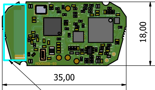
View Top ( 2 : 1 )
