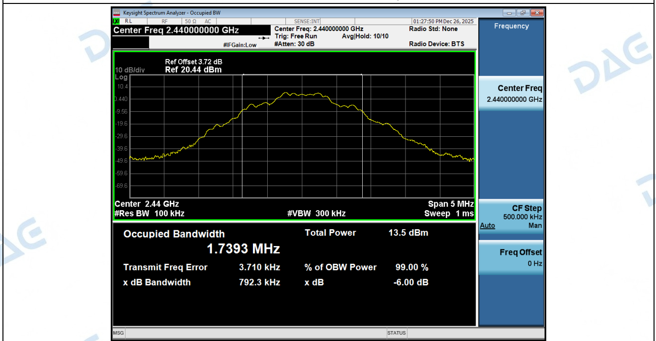
-6dB Bandwidth_NVNT_ANT1_1Mbps_2440
