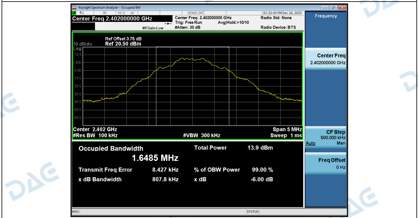
-6dB Bandwidth_NVNT_ANT1_1Mbps_2402
