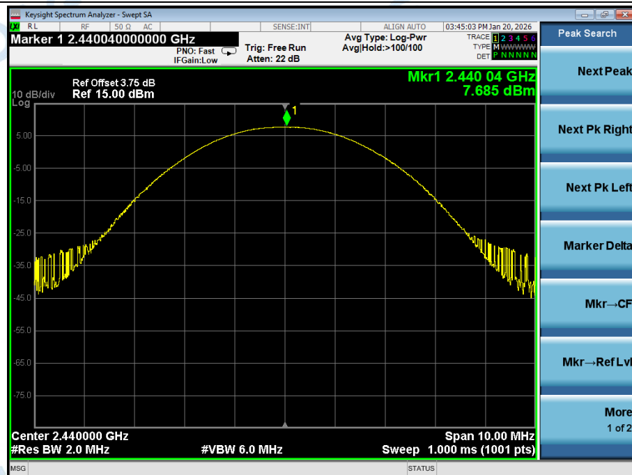
Peak_Output_Power_NVNT_ANT1_1Mbps_2440
