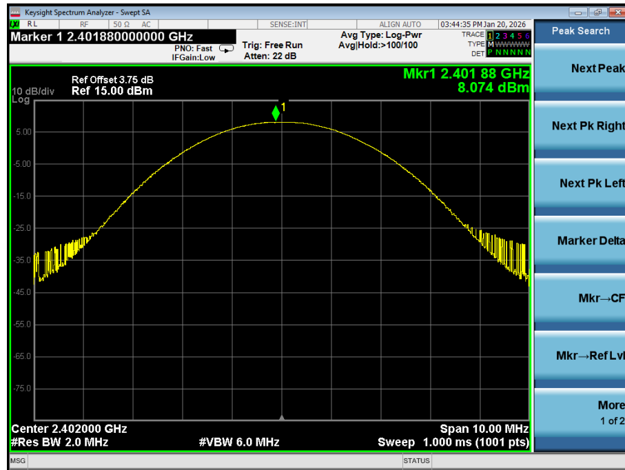
Peak_Output_Power_NVNT_ANT1_1Mbps_2402
